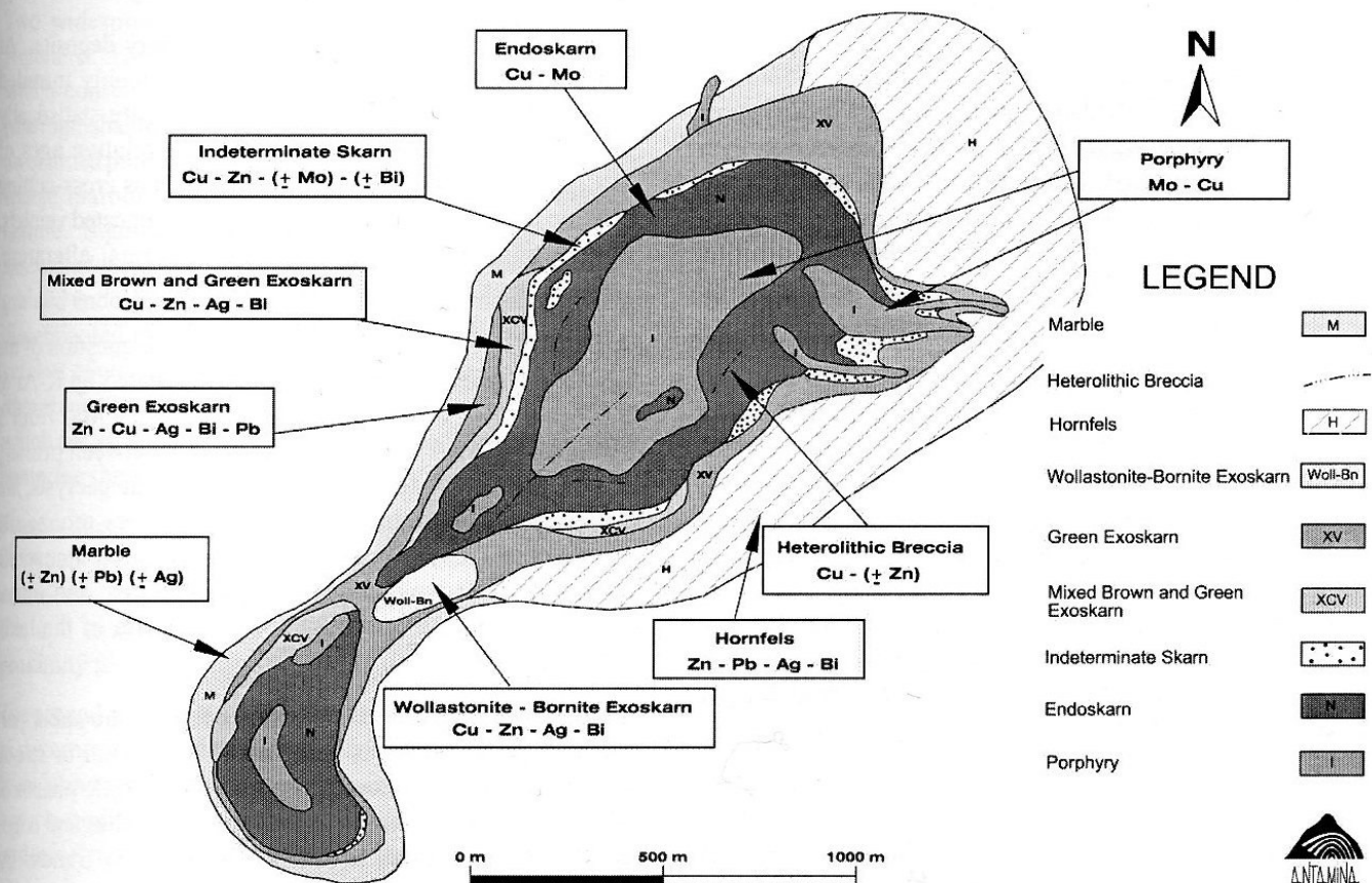
Figure 5: Schematic Plan of Lithology and Metal Zonation
