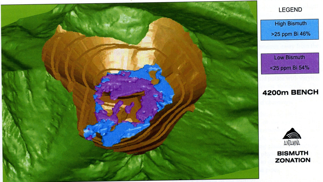
Figure 9: Antamina Deposit, Bismuth Zonation
