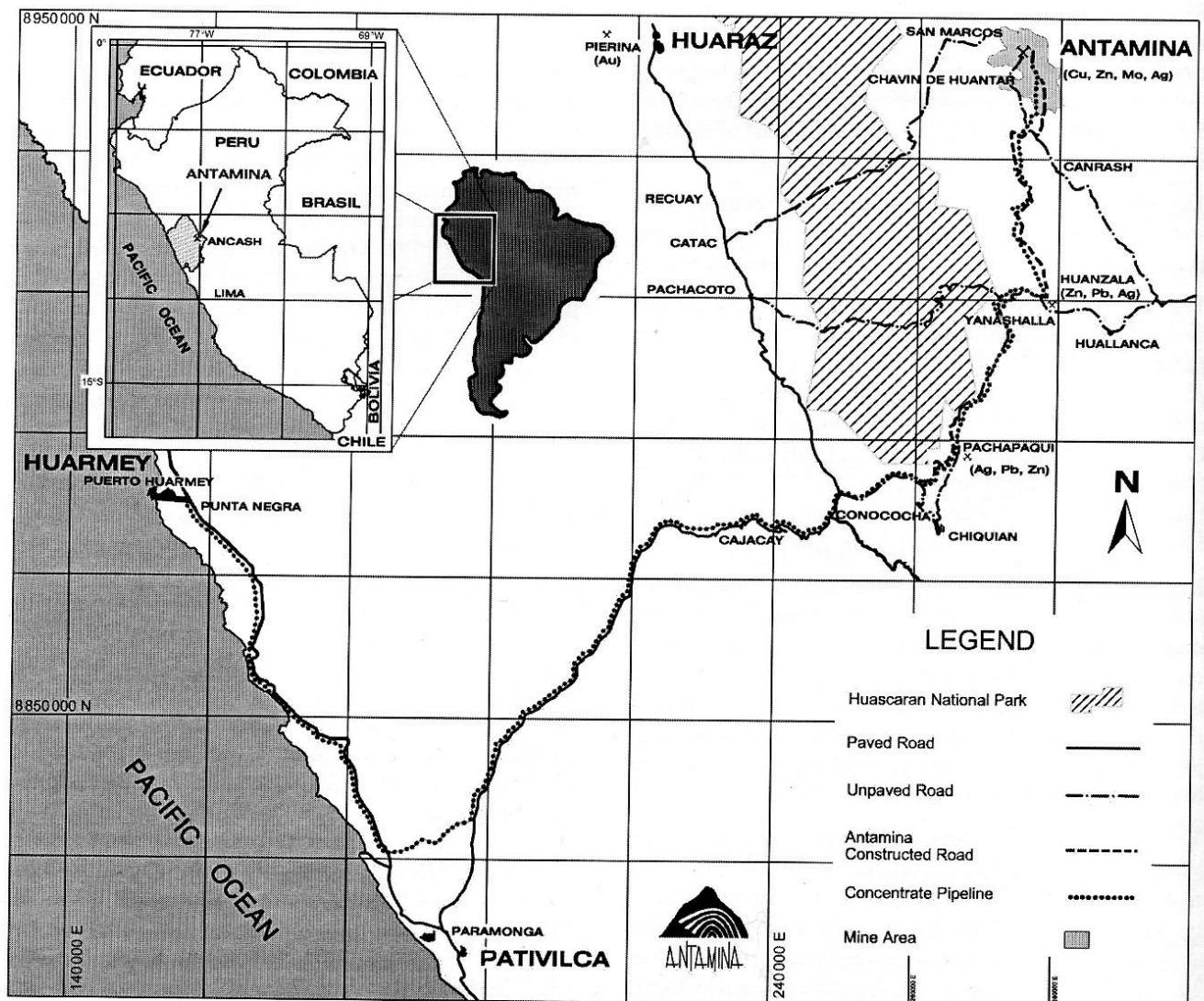
Figure 1: Location Map of the Antamina Mine
