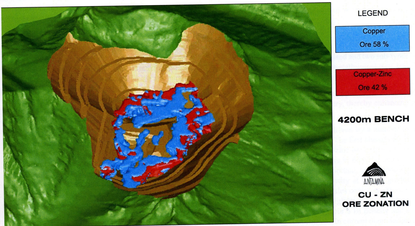
Figure 10: Antamina Deposit Copper-Zinc Zonation
