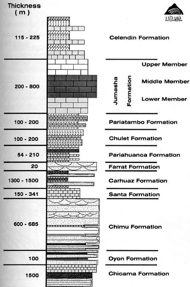
Figure 3: Stratigraphy of the Antamina District
