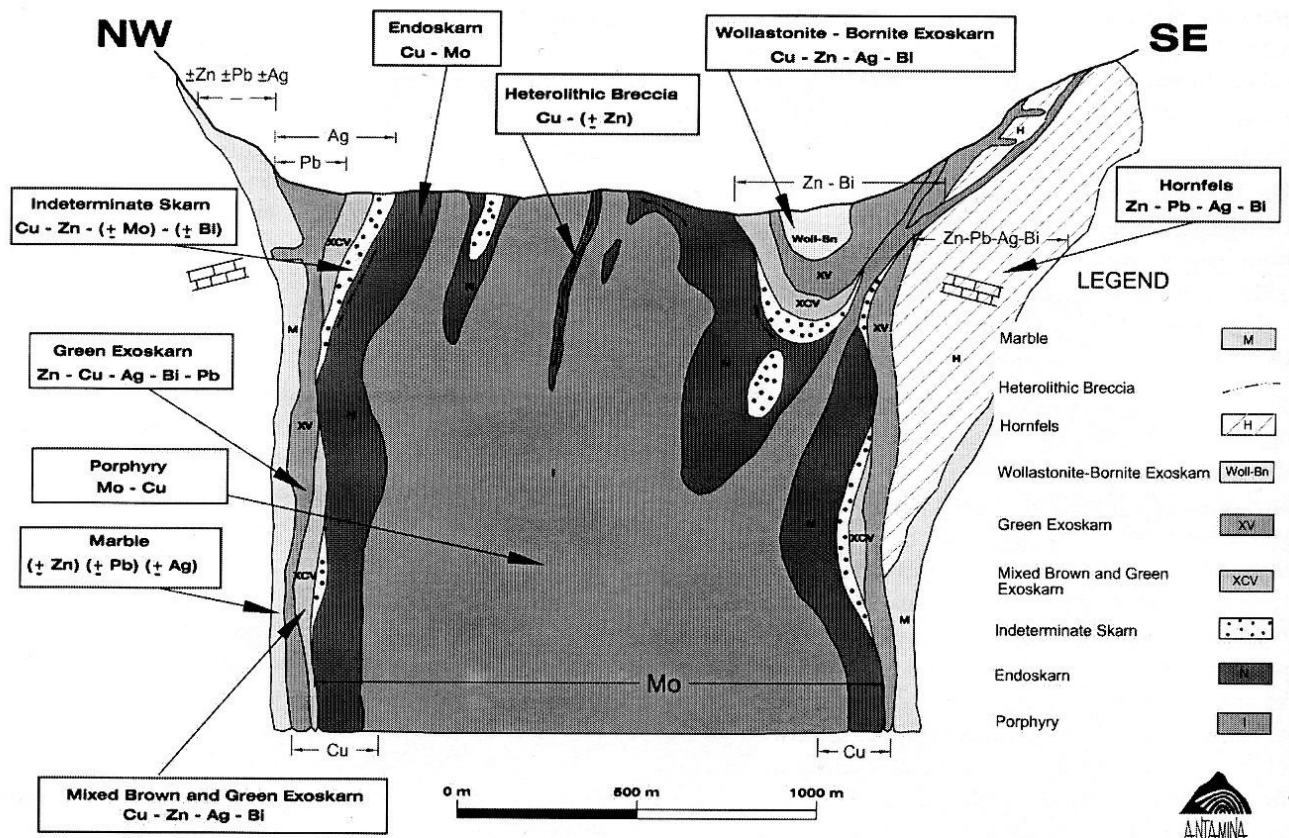
Figure 6: Schematic Section of Lithology and Metal Zonation
