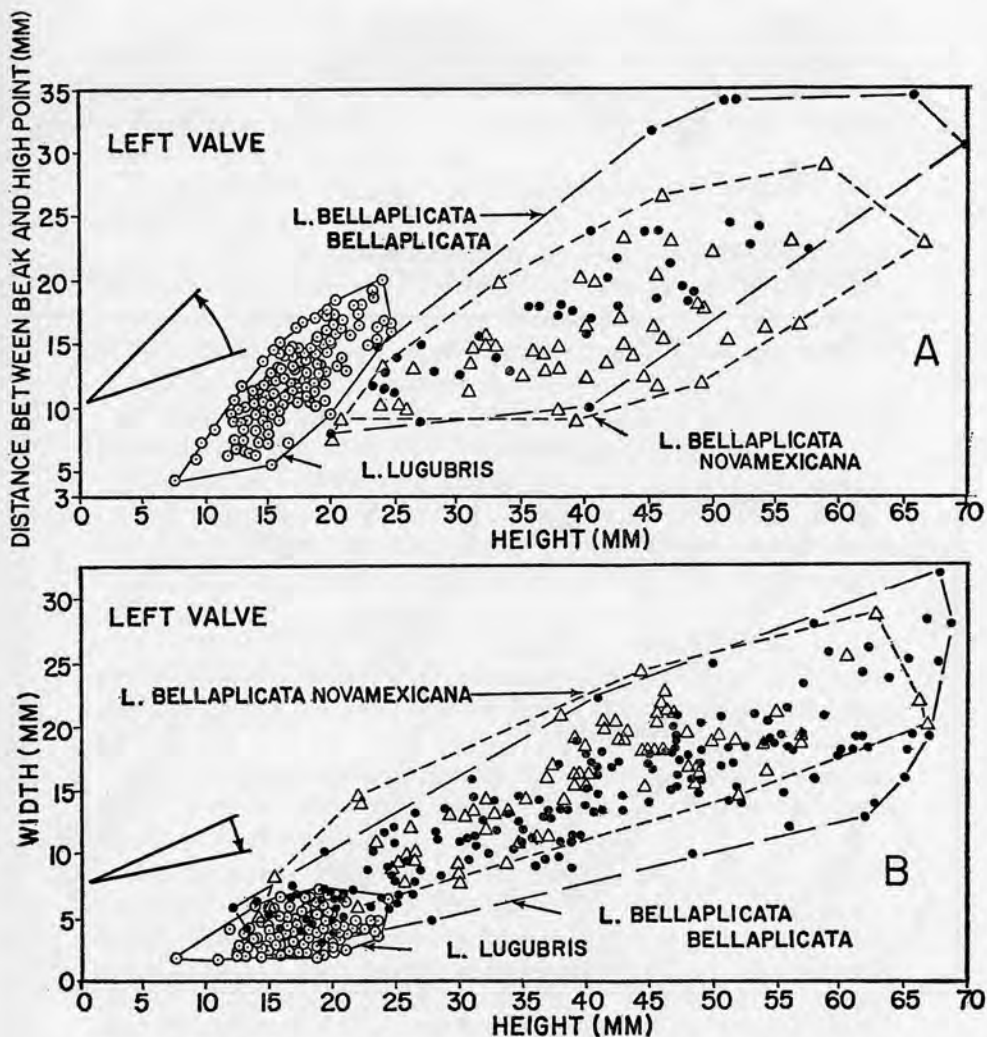
FIG. 4.—Evolution in the Lopho lugubris group. A, Scattergram showing relationship between valve height and the distance between the beak and high point of the left valve, measured parallel to height. Note ventral shift of the high point in progressively younger forms. Arrow in lower left-hand corner denotes direction of ventral migration of high point as illustrated by hypothetical regression lines fitted visually to plots of end members of group. B, Scattergram showing relationship between height and width of left valves. Note slight decrease in relative convexity of left valve in progressively younger forms. Arrow in lower left-hand corner denotes direction of decreasing convexity as illustrated by hypothetical regression lines fitted visually to plots of end members of lineage.
