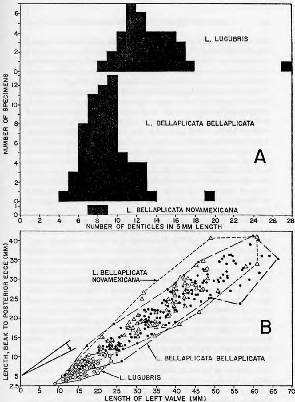
FIG. 9.—Evolution in the Lopho lugubris group. A, Increase in the density of the denticles along the inner lateral and dorsolateral margins in successively younger species. B, Ventral shifting of the beaks along the dorsal margin in successively younger species and subspecies, and decrease in the length of the posterior auricle. Arrow in lower left-hand corner denotes direction of central shifting of beak along dorsal margin as shown by hypothetical regression lines visually fitted to plots of terminal species in lineage.
