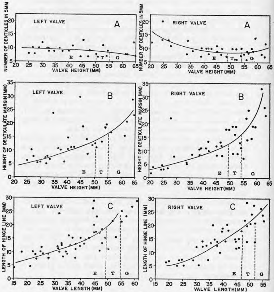
FIG. 17.—Ontogenetic development of Lopha bellaplicata bellaplicata (Shumard). A, Relationship between number of denticles in 5 mm. length (measured along margin) and valve height, showing decrease in density with age, and with increase in size. B, Relationship between the height of the valve and the extent of the denticulate portion of the margin, measured in terms of height, showing increase in extent of denticles with age and size. C, Relationship between length of hinge line and valve length, showing increase in size of hinge line relative to lateral expansion with age and size. All lines fitted visually. Approximate boundaries between ontogenetic stages marked by dashed lines. E = Ephebic; T = Ephebic-Gerontic transition; G = Gerontic.
