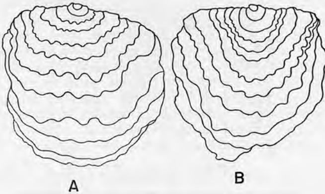
FIG. 15.—Ontogeny of Lopha bellaplicata bellaplicata (Shumard). Growth line traces at approximately 2.5 mm. intervals on representative left (A) and right (B) valves of the species. Traces show developmental history of the valve outline and the auricles. Drawings \times 1 . A, U.S.N.M. 132225; B, U.S.N.M. 132239.
