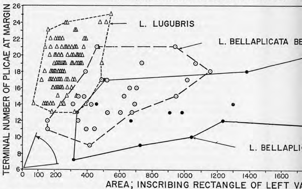
FIG. 2.—Evolution of the Lopha lugubris group. Increase in the density of the plicae, number per unit area, measured, from Colorado, New Mexico, Texas. B, Scattergram of Colorado sample only. Arrows indicate direction of increase in density as shown by hypothetical regression lines visually fitted to plots of terminal species in group.
