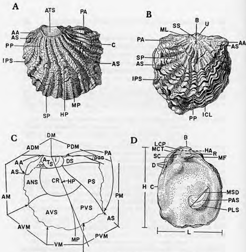
FIG. 10.—Morphology of oysters in the Lopho lugubris group, using specimens of L. bellaplicata bellaplicata for illustration (A, C, U.S.N.M. 132222; B, U.S.N.M. 132239; D, U.S.N.M. 8024d). A, External shell morphology of left valve. B, External shell morphology of right valve. C, Spatial divisions of valve referred to in text. D, Interior morphology of right valve. Symbols explained in detail under "Shell Morphology." AA, Anterior auricle. ADM, Anterodorsal margin. AM, Anterior margin. ANS, Anterior slope. AS, Auricular sulcus. ATS, Attachment scar. AVM, Anteroventral margin. AVS, Anteroventral slope. B, Beak. C, Commissure. CR, Crest of valve. D, Denticles. DM, Dorsal margin. DS, Dorsal slope. H, Height of valve. HA, Hinge axis. HP, High point of valve. i , Angle of inclination. ICL, Imbricating concentric lamellae. IPS, Interperical sulcus. L, Length of valve. LCP, Lateral cardinal plate. MCT, Marginal cardinal trough. MF, Midcardinal fold. MP, Median plica. MSD, Maximum diameter of posterior adductor muscle scar. PA, Posterior auricle. paa , Posterior auricular angle. PAS, Posterior adductor muscle scar. PDM, Posterodorsal margin. PLS, Posteroventral lip of the muscle scar. PM, Posterior margin. PP, Primary plica. PS, Posterior slope. PVM, Posteroventral margin. PVS, Posteroventral slope. R, Resilifer. SC, Subcardinal cavity. SP, Secondary plica. SS, Smooth stage of umbo. U, Umbo. VM, Ventral margin. All figures \times 1 .
