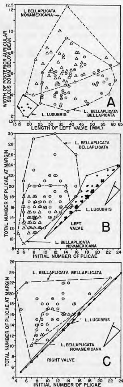
FIG. 6.—Evolution in the Loph lugubris group. A, Variation plot showing relationship between the width of the posterior auricular sulcus 20 mm. below the beak and the length of the left valve, the most variable linear measurement. Note variation within each form and good separation of variation plots, lack of correlation between width and valve length, and decrease in the relative width of the sulcus at this point in progressively younger species and subspecies (the latter defined by differences in the vertical range of the individual variation plots). B, C, Comparison of the bifurcation rates of the radiating plicae on various members of the group, showing an increase in bifurcation of the plicae from L. bellaplicata novamexicana to the younger L. bellaplicata bellaplicata and then an abrupt decrease in bifurcation rate with the evolution of L. lugubris , in which the majority of specimens lack bifurcating plicae. Arrows on right central portion of B and C denote direction of increasing bifurcation rate as illustrated by hypothetical regression lines visually fitted to plots of terminal members of group.
