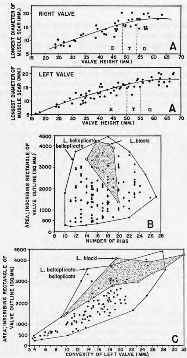
FIG. 16.—A, Ontogeny of the muscle scar in Lophya bellaplicata bellaplicata (Shumard), showing relationship between maximum diameter of the posterior adductor muscle scar and the height of the valve. Note the decline and virtual cessation of scar growth with increased size and age. Approximate boundaries between ontogenetic stages marked by dashed lines. E = Ephebic; T = Ephebic-Gerontic transition; G = Gerontic. B, Comparison of the plication density of Lophya bellaplicata bellaplicata with that of L. blacki (White), showing total overlap of the two forms. C, Comparison of the relative convexity of L. bellaplicata bellaplicata and L. blacki , showing nearly total overlap between the two forms.
