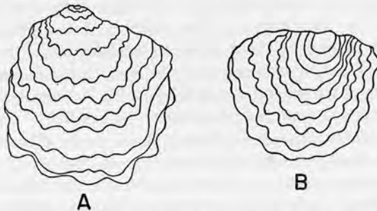
FIG. 18.—Ontogeny of Lopha bellaplicata novamexicana new subspecies. Growth line traces at approximately 2.5 mm. intervals on representative left (A) and right (B) valves of the subspecies, showing developmental history of the marginal outline and the auricles. Drawings \times 1 . A, U.S.N.M. 132267, B, U.S.N.M. 132265.
