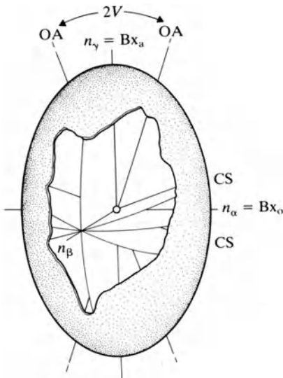
Figure 4.3 Positive biaxial indicatrices. OA, optic axis; CS, circular section; Bx_\alpha , acute bisectrix; Bx_o , obtuse bisectrix.
