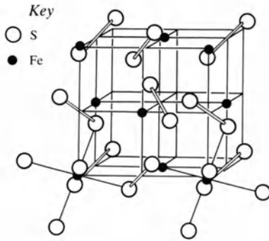
Figure 3.3 Sulphide structures (after Vaughan & Craig 1978).
