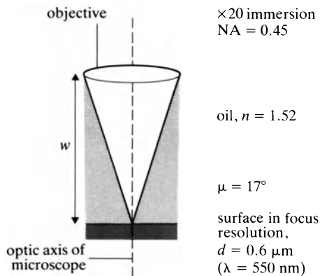
Figure 1.5 Numerical aperture and resolution. \text{N.A.} = n \sin \mu , where N.A. = numerical aperture, n = refractive index of immersion medium, and \mu = half the angle of the light cone entering the objective lens (for air, n = 1.0 ). d = 0.5 \lambda / \text{N.A.} where d = the resolution (the distance between two points that can be resolved) and \lambda is in microns (1 micron = 1000 nm). The working distance ( w in the diagram) depends on the construction of the lens; for the same magnification, oil immersion lenses usually have a shorter distance than dry objectives.
