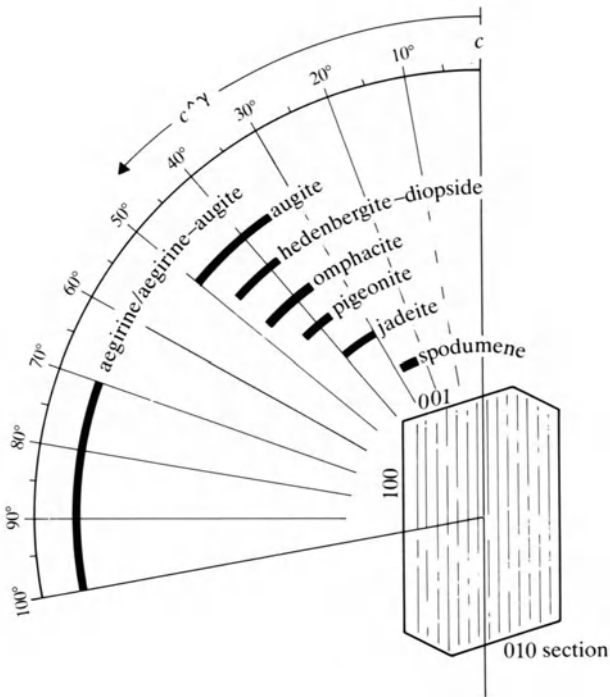
Figure 2.22 Extinction angles for clinopyroxenes. Ranges of c^{\gamma} (maximum extinction angles) for several common pyroxene minerals. Note that c^{\alpha} extinction angles for aegirine/aegirine-augite vary from 0^{\circ} to \sim 20^{\circ} .
