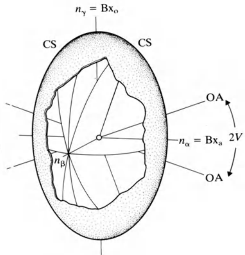
Figure 4.4 Negative biaxial indicatrices. OA, optic axis; CS, circular section; Bx_\alpha , acute bisectrix; Bx_o , obtuse bisectrix.
