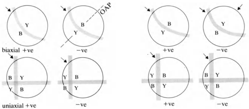
Figure 4.20 Determination of optical sign of interference figures using either length slow or length fast accessory plates, and with their direction of insertion either NE-SW or NW-SE. In the sets of cartoons, numbers (a) and (d) are probably the most helpful. In (a) and (b), the uniaxial cross is placed in the lower left-hand corner of the field of view, and the biaxial single optic axis isogyre is rotated until it is concave towards the north-east. The cross and isogyre can, however, also be placed in the lower right-hand corner of the field of view with the isogyre concave towards the north-west. This is shown in (c) and (d).
