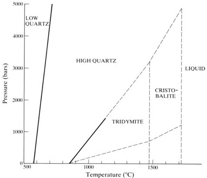
Figure 2.29 Pressure–temperature diagram for \text{SiO}_2 (after Tuttle & Bowen 1958).
