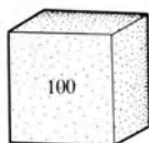
cube 100
