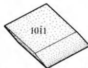
rhombohedron 10\bar{1}1
