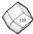
dodecahedron 110
