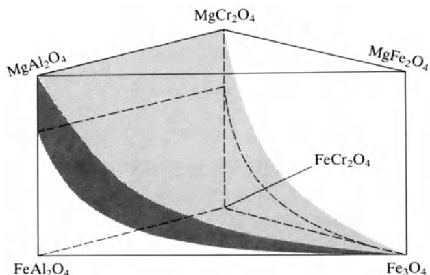
Figure 3.10 Solid solution in spinel.
