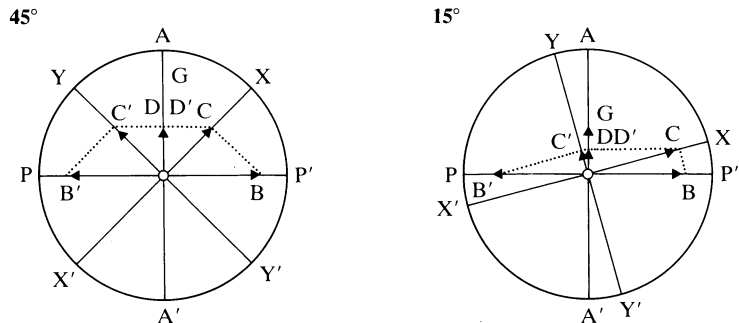
Figure 4.14 Constructive interference.
