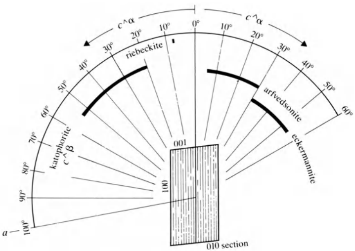
Figure 2.5 Extinction angles of amphiboles. Note that c^{\wedge}\beta for katophorite will be cleavage's slow ray, since the other component in this orientation is \alpha .
