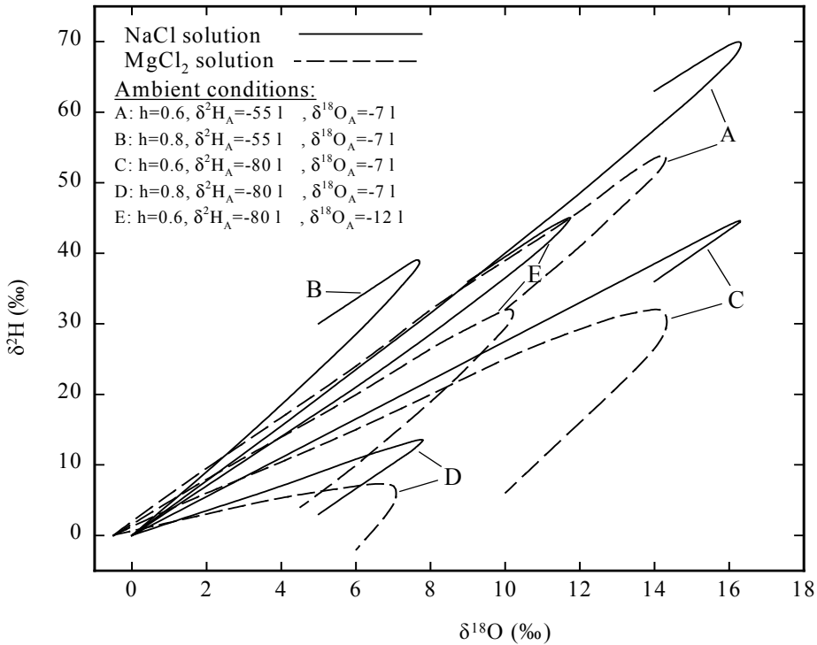
FIG. 4. Computed \delta^2\text{H} composition and \delta^{18}\text{O} activity values for 0.5 molal \text{NaCl} or \text{MgCl}_2 solutions evaporating under different environmental conditions. The "loop" occurs only in the very late stages of desiccation (from Sofer and Gat, 1975).
