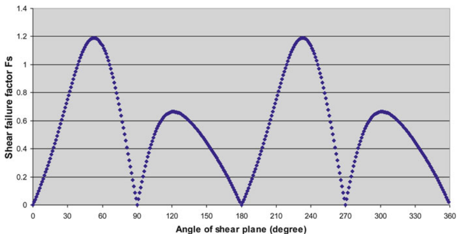
Fig. 11.2 Four potential shear failure planes at which the failure factor F_s reaches a peak. The planes with maximum F_s are the actual failure planes
