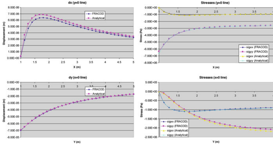
Fig. 13.11 Comparison between FRANC3D results and analytical results for the circular tunnel
