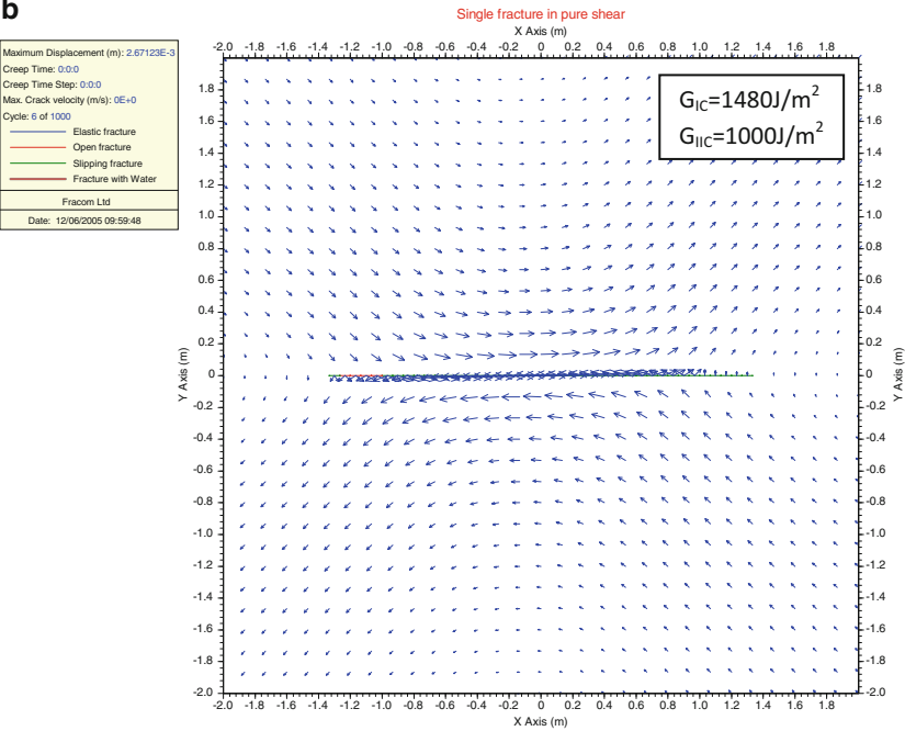
Fig. 13.2 Fracture propagation in Mode I ( top ) and Mode II ( bottom ) depending on the ratio of G_{IIC}/G_{IC}
