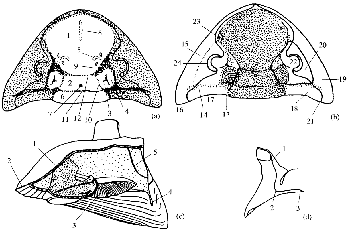
Fig. 20. Structure of the trilobite cephalon in the subfamily Asaphinae: (a) rachis area (pale): (1–5) glabella lobes: (1) frontal, (2) medial, (3, 4) basal: (3) glabellar, (4) genal composite, (5) rudimentary lobes, (6) occipital ring, (7) medial (occipital) tubercle, (8) keel-like ridge, (9–11) furrows: (9) glabellar, (10) pseudodorsal, (11) occipital, (12) transverse flexure of glabella; (b) pleural area (pale): (13–15) furrows: (13) dorsal, (14) posterior marginal, (15) paradoublural, (16, 17) genae: (16) librigena, (17) fixed gena, (18) posterior marginal bordering, (19) lateral portion of gena, (20) ocular area (outlined), (21) facial suture, (22) ocular ridge, (23) fossula, (24) watching surface of eye; (c) scheme of attaching hypostome to cephalon: (1) anterior flange of hypostome, (2) anterior branch of facial suture, (3) wedgelike process of hypostomal bordering, (4) panderian organs, (5) posterior branch of facial suture (inner surface of carapace is dotted); (d) bends of anterior branch of facial suture: (1) ocular, (2) marginal, (3) anterior.
