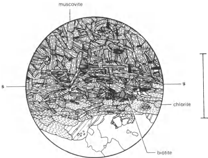
Figure 2.19 Thin section of schist, from below the garnet isograd, Sulitjelma, Norway. Scale bar 1 mm.
