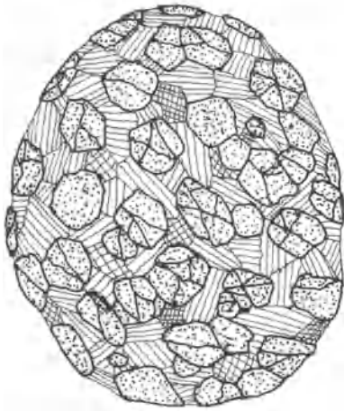
Figure 9.1 Hand specimen of Roberts Victor eclogite from South Africa. The oval shape is the shape of the eclogite xenolith in the soft matrix of the kimberlite. The garnets stand out, having been less abraded than the green omphacite pyroxene between them during the time when the eclogite xenolith was brought to the surface. Scale in cm.
