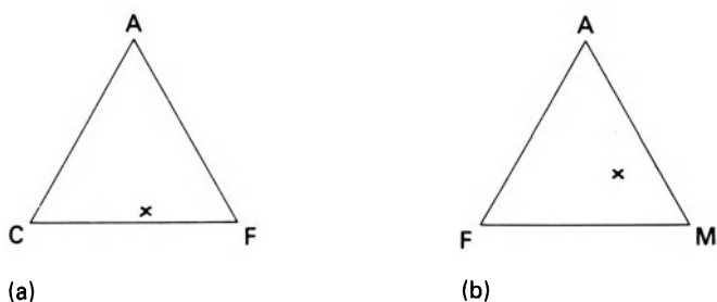
Figure 2.14 (a) ACF triangular composition-assemblage diagram for the calculation in Table 2.2 (b) AFM triangular composition-assemblage diagram for the calculation in Table 2.3.
