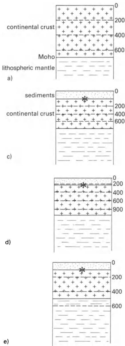
Figure 5.12 Sequence of events in the sedimentary basin formed by the filling of the basin in Figure 5.11. (Letters are in the same sequence as in Figure 5.11). (a) Steady-state continental geotherm before extension. (c) Basin has filled quickly with cold sediment after extension. (d) High geothermal gradient migrates upwards and heats sediments in basin. (e) Geothermal gradient relaxes back to steady-state. Asterisk – position of sedimentary rock whose d-T-t path is shown in Fig. 5.13.
