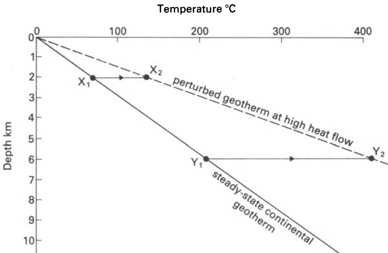
Figure 2.24 Schematic geothermal gradients from example discussed in the text. X_1 – X_2 change in temperature of rock 2 km below surface, Y_1 – Y_2 change of temperature in rock 6 km below surface.
