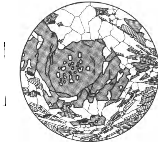
Figure 7.13 Garnet-mica schist, Otervatn. Scale bar 1 mm.
