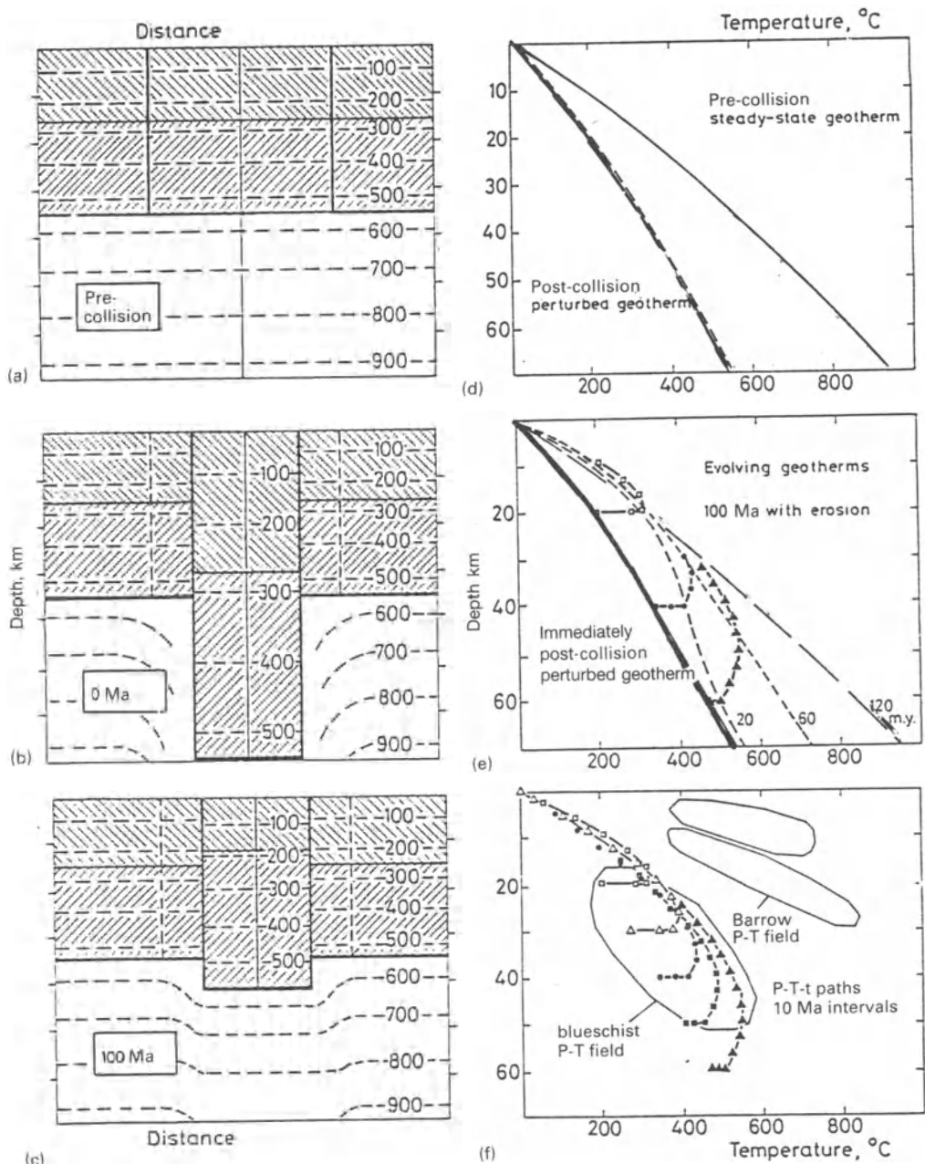
Figure 7.2 Thermotectonic model for continental collision by homogeneous strain, from Thompson (1981). (a) Steady-state conditions at the onset of collision. (b) Deformation of prism of continental lithosphere by homogeneous strain after collision. The isotherms have moved further apart, producing a perturbed geotherm with a low geothermal gradient. (c) 100 Ma after collision, with uplift and erosion of deformed orogenic prism, and partial relaxation of isotherms. (d) Post collision perturbed geotherm compared with steady-state geotherm. (e) Evolving geotherms, at 20, 60 and 120 Ma after collision. (f) Depth-T-t curves for rocks at different depths within the deformed prism.
