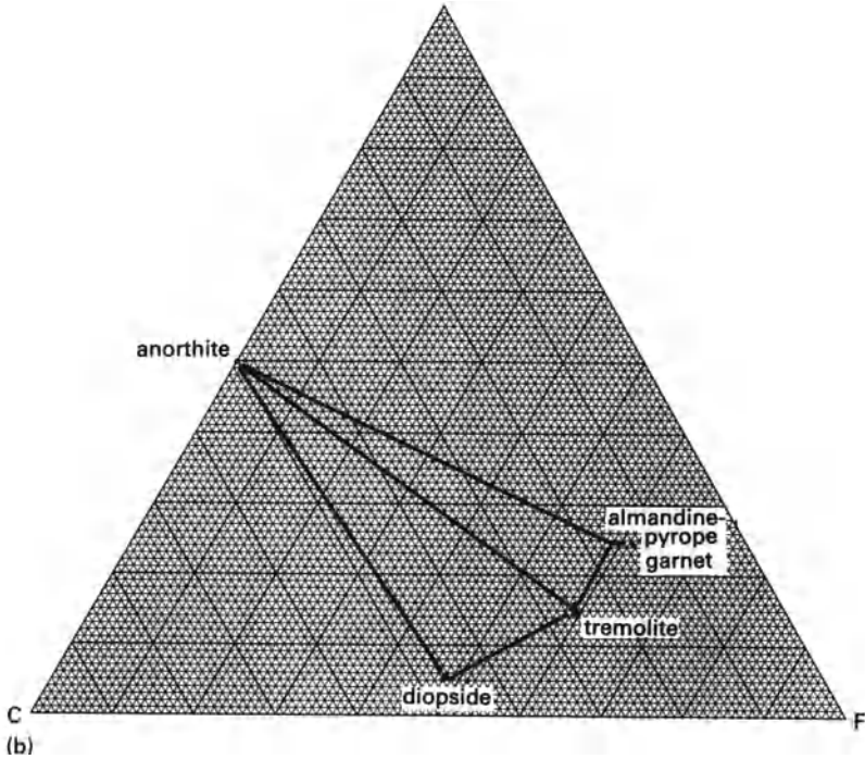
Figure 2.16 (a) ACF diagram for skarns from Neyriz, Iran, plotting 'ideal' compositions for minerals. (b) The same diagram, plotting actual mineral compositions as dots. Notice that there are fewer minerals on this diagram, because the only minerals plotted are those which have actually been analysed. From data supplied by R. Hall.
