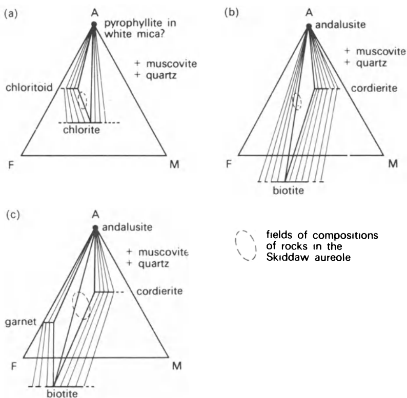
Figure 3.13 AFM diagrams summarizing the mineral assemblages of the Skiddaw aureole. (a) Mineral assemblages of the outer zone (b) Mineral assemblages of the intermediate zone (c) Mineral assemblages of the inner hornfels zone.
