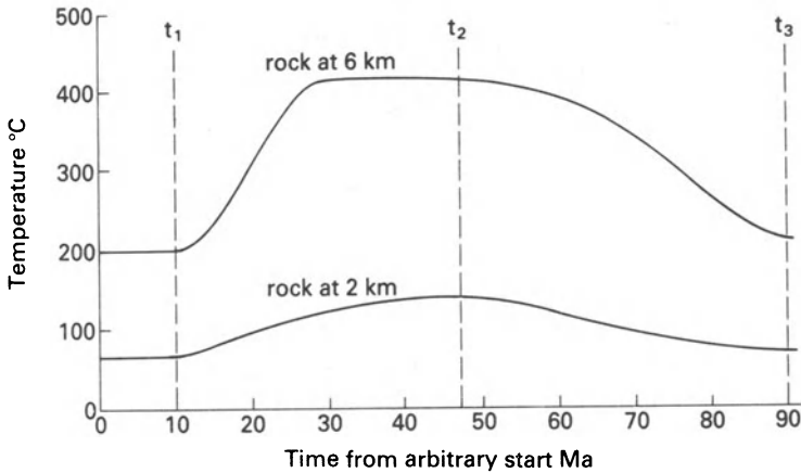
Figure 2.25 Temperature–time curves from example discussed in the text. Upper curve, rock at 6 km depth, lower curve, rock at 2 km depth.
