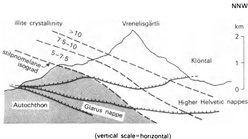
Figure 5.19 Cross section along the western side of the Linth Valley, Canton Glarus, Switzerland, showing the variation of illite crystallinity with height, and the incoming of stilpnomelane. The surface marking the first appearance of stilpnomelane is called an isograd.
