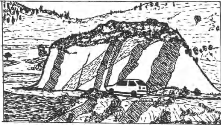
Figure 5.6 Dykes in the Sheeted Complex at Zoopiye, Troodos Ophiolite, looking northwards. The dykes are intruded into light-coloured plagiogranite, in the lower part of the Sheeted Complex. The gently dipping dyke is metamorphosed to greenstone, while the near vertical dykes are unmetamorphosed dolerite. Models for the evolution of sheeted complexes by repeated dyke intrusion suggest that initially vertical dykes rotate to a gentler dip as they spread away from the ridge. Thus this drawing suggests that the ocean-floor metamorphism occurred close to the ridge, but not exactly on it.
