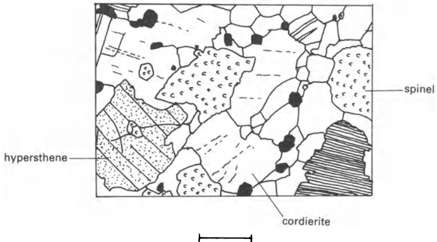
Figure 3.3 Hornfels showing equilibrium granoblastic texture with 120^\circ triple junctions. Contact aureole of Sulitjelma gabbro, Norway. Scale bar 0.1 mm.
