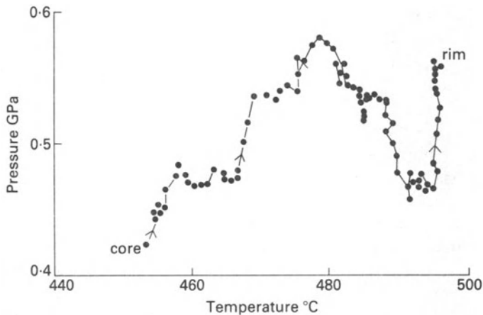
Figure 7.17 Part of a P–T–t path derived by calculation from the zoned garnet porphyroblast in Figure 7.16.
