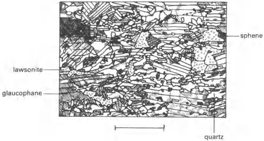
Figure 6.4 Glaucophane-lawsonite schist from Berkeley Hills, California, USA. Scale bar 1 mm.
