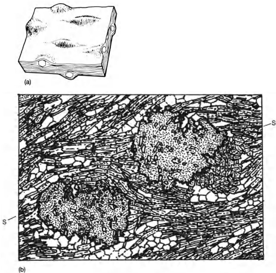
Figure 2.1 (a) Drawing of hand specimen of schist from Sulitjelma, Norway, with garnet porphyroblasts causing a change in the schistosity direction. (b) Thin section of the same schist, showing garnet porphyroblasts surrounded by a groundmass of biotite, muscovite, quartz and plagioclase feldspar. The schistosity is marked s-s. Scale bar 1 mm.
