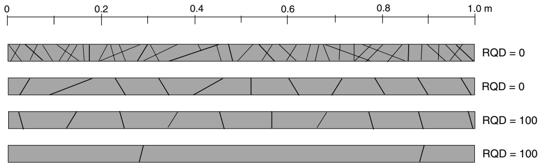
Fig. 11. Examples of minimum and maximum values of RQD for various joint densities along drill cores (from Palmstrom, 2001).
