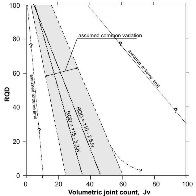
Fig. 18. The probable common variation for RQD– J_v and suggested equations.
