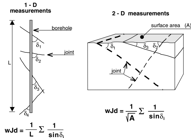
Fig. 8. The definitions of wJd measurement for borehole and surface registrations. (Palmstrom, 1995).
