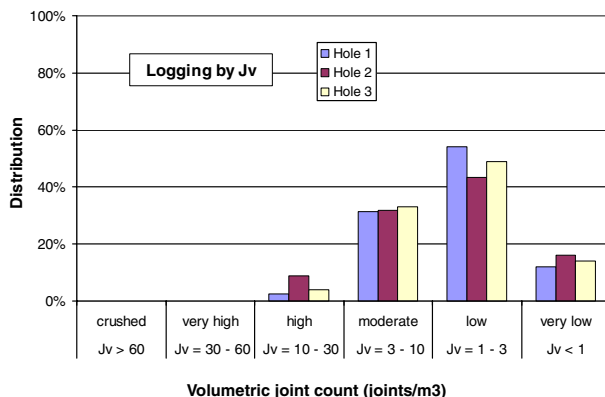
Fig. 20. Measurements of J_v (=wJd) and RQD in 3 boreholes with total length of 450 m in gneiss and amphibolite.
