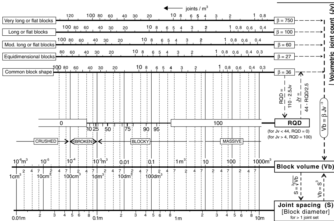
Fig. 22. Correlations between various measurements of block size. The block volume ( V_b ) and volumetric joint count ( J_v ) cover a significantly larger interval of the jointing than the RQD. The best correlation exists between J_v and V_b . However, also the block shape influences on the correlations. Example: For a block size of V_b = 0.1 \text{ m}^3 the J_v = 6.5 when block shape factor \beta = 27 ; but J_v = 9 when \beta = 100 .
