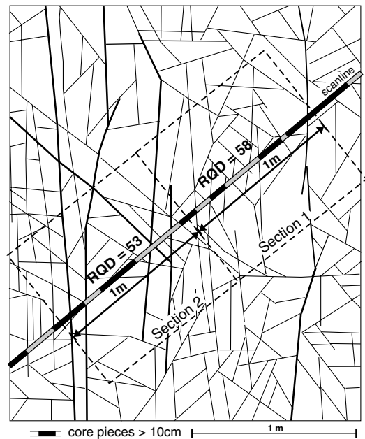
Fig. 10. By applying a scanline in Fig. 2, the RQD-values can be found. “Core pieces” > 10 cm are shown in black. However, this measurement does not show the large variation in block sizes as is seen in Fig. 5.
