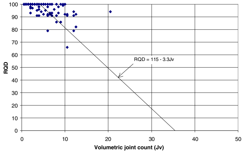
Fig. 14. Results from logging of a 223 m long core drill hole at Ormen Lange petrochemical terminal, Norway, where both RQD and wJd measurement were performed.
