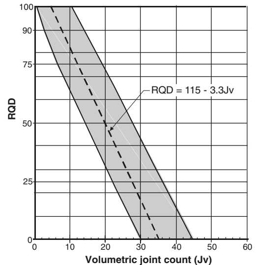
Fig. 13. Correlation J_v -RQD with the variation range (modified into linear scale for J_v , from Palmstrom, 1974).
