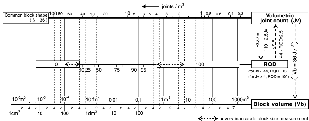
Fig. 23. Correlations between different methods for block size measurements.
