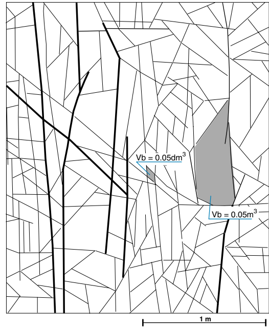
Fig. 5. The block volumes in Fig. 2 vary between approx. 5 \times 10^{-5} m 3 and 5 \times 10^{-2} m 3 . Average block size \approx 0.025 m 3 .
