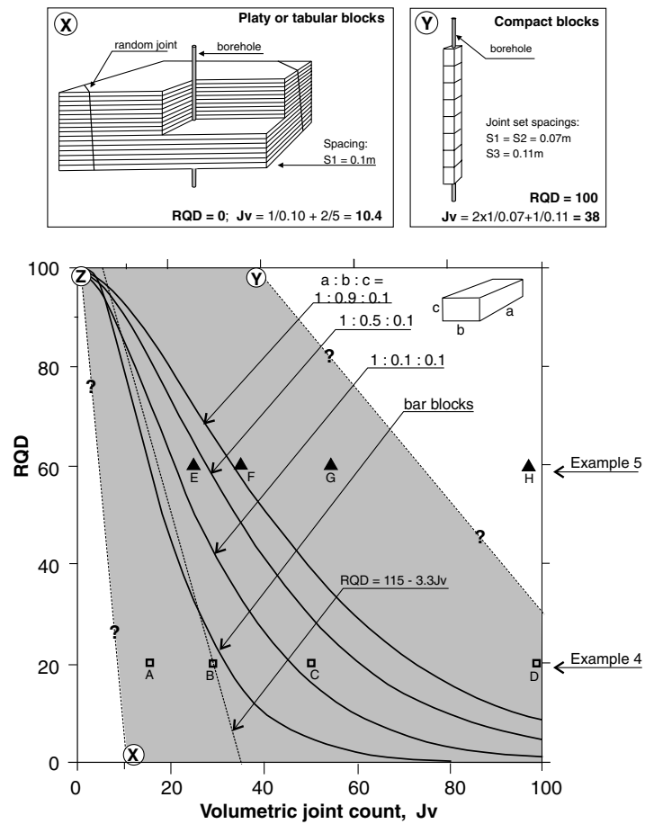
Fig. 17. The approximate correlation between RQD and J_v based on Figs. 14–16. The points (X) and (Y) show extreme jointing conditions to indicate the variation limits of RQD.
