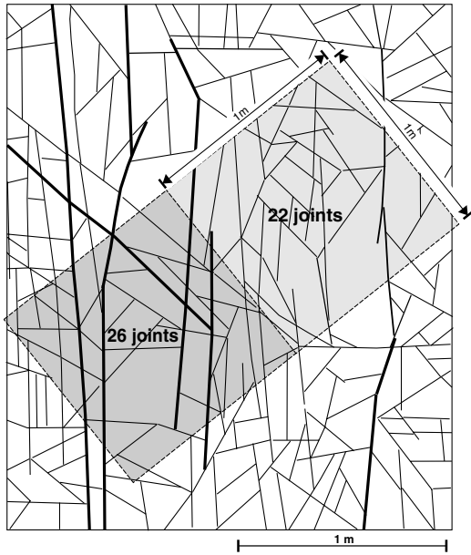
Fig. 7. Observation of the number of joints in the location of Fig. 2. The many short joints in this location cause inaccuracy of J_v (because its definition applies for joints longer than 1 m) with too high value of J_v . Therefore, J_v as defined in Eq. (15) does not characterize the degree of jointing correctly in this location.
