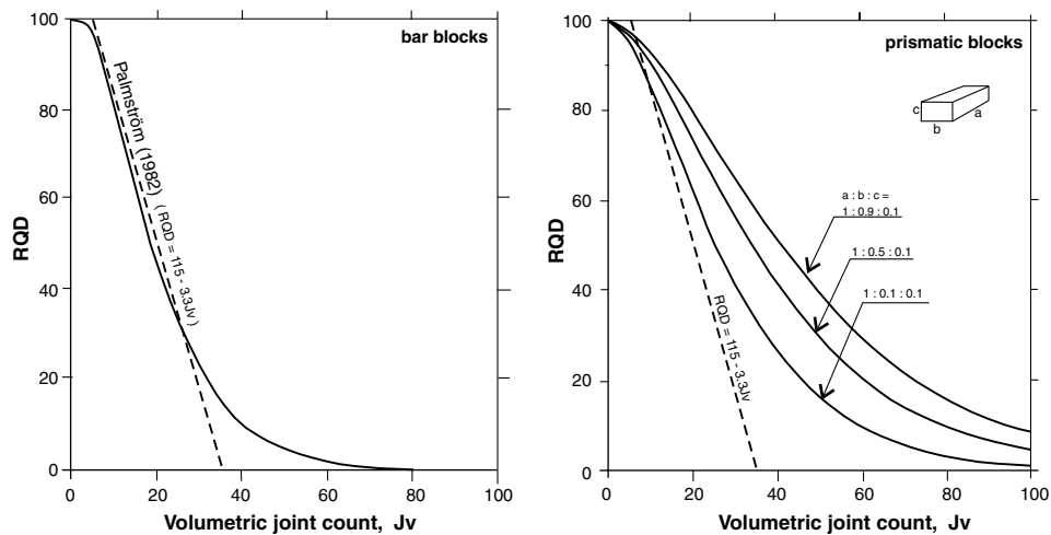
Fig. 15. Correlation J_v -RQD, modified from Sen and Eissa (1991) for bar (long) blocks (left figure) and for prismatic blocks.
