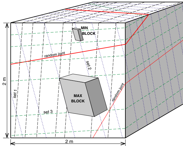
Fig. 4. Regular jointing with 3 joint sets and a few random joints. The minimum and maximum block size in a rock mass volume of 2 × 2 × 2 m (from Palmstrom, 2001).
