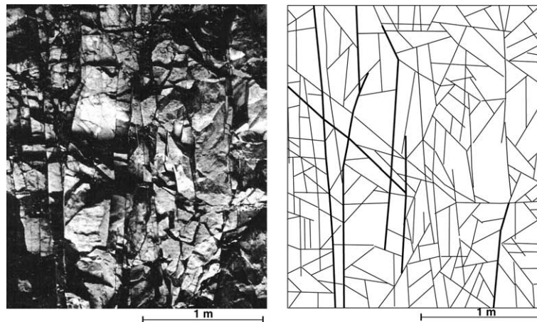
Fig. 2. Photo and interpretation of (irregular) jointing of a dolerite (diabase), which shows the difficulties involved in block size measurement. The jointing consists of some medium (3–10 m long) and many small (short) joints causing great variation in block sizes, as is seen on the right figure.
