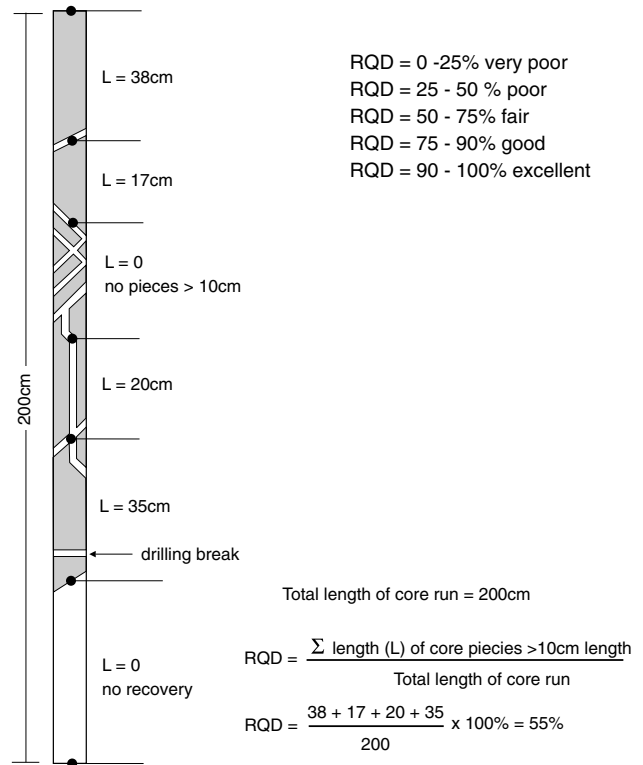
Fig. 9. Procedure for measurement and calculation of RQD (slightly modified after Deere, 1989).
