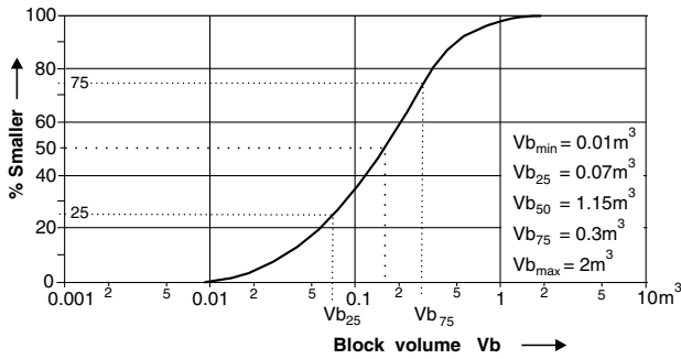
Fig. 6. Example of a distribution curve for block sizes (from Palmstrom, 2001).
