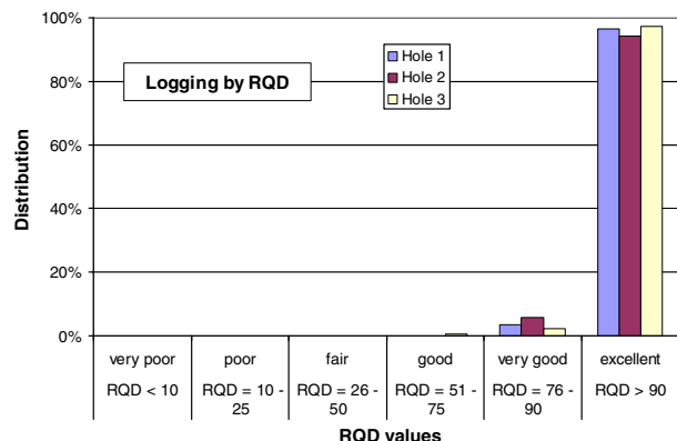
Fig. 20. Measurements of J_v (=wJd) and RQD in 3 boreholes with total length of 450 m in gneiss and amphibolite.
