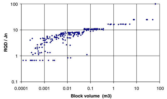
Fig. 21. Block volume RQD/Jn based on the same conditions as for Fig. 16. Note that both axes are logarithmic (from Palmstrom et al., 2002).
