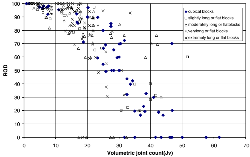
Fig. 16. Correlations between RQD and J_v . Results from a computer calculation of lines penetrating blocks of the same size at different angles (from Palmstrom et al., 2002).
