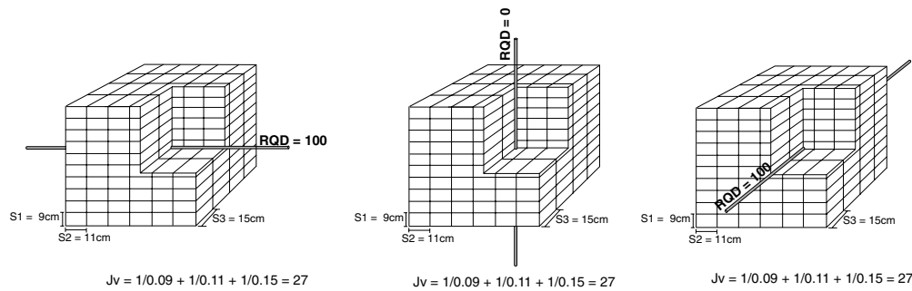
Fig. 12. Three boreholes penetrate the same rock mass in different directions. As seen, the RQD can be both 0 and 100.
