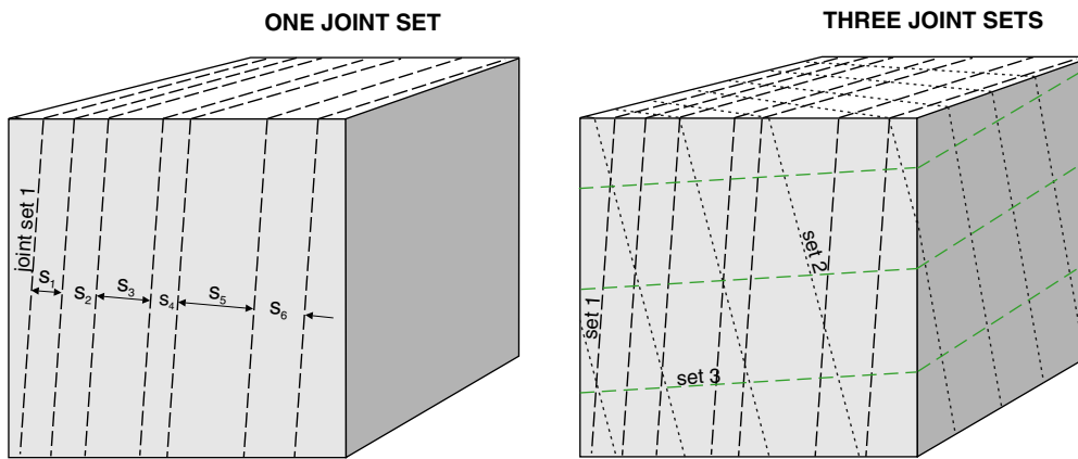
Fig. 3. Joint sets and joint set spacing.
