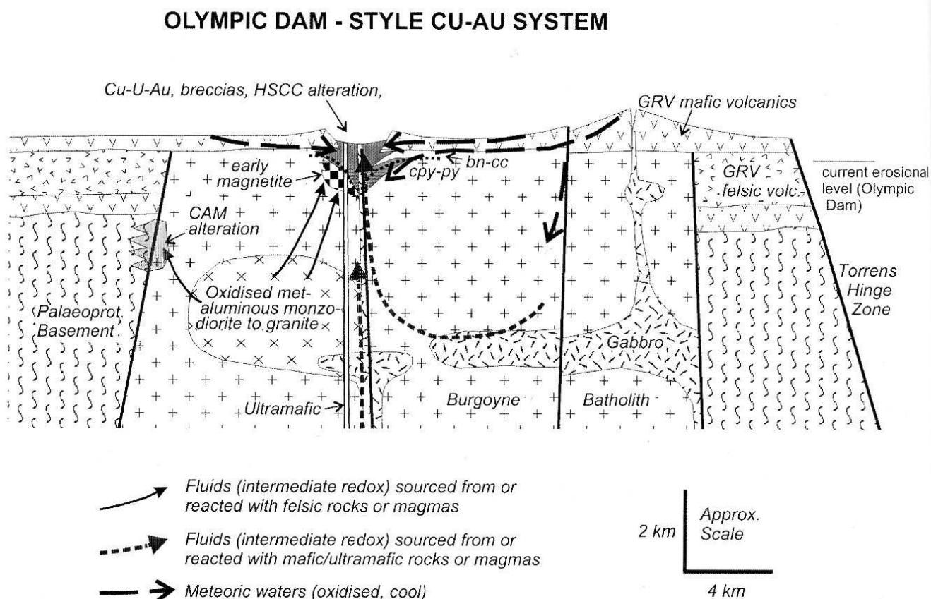
Figure 6: Schematic cross section of an Olympic Dam style hydrothermal system, showing Cu-U-Au mineralisation associated with hematite-sericite-chlorite-carbonate (HSCC) alteration. Deeper level and/or distal calcsilicate-alkali feldspar-magnetite alteration (CAM), and alternative fluid types that may have been active in the system, are also shown (see text). The interface between chalcopyrite-pyrite (cpy-py) and bornite-chalcocite (bn-cc) assemblages is indicated. Geology based on Reeve et al. (1990) and Haynes et al. (1995).
