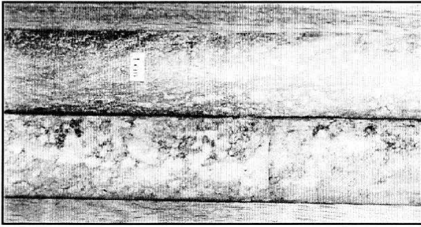
Amigdaloidal metandesite with quartz - Drill hole ALM-FD09.
