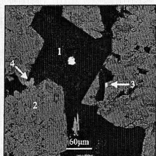
BSE image showing a uraninite crystal inclusion in greenalite (1) surrounded by magnetite (2), and inclusions of monazite (3) in chalcopyrite (4). Drill hole ALM-FD 09.
