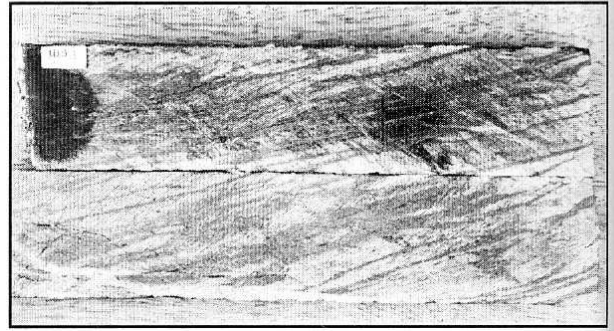
Laminated iron formation (oxide facies) -Drill hole ALM-FD09.
