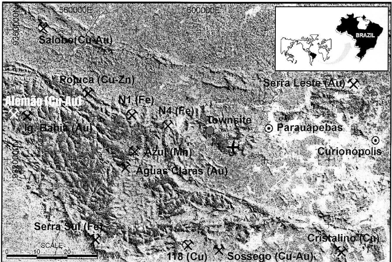
Figure 1 - Location Map - Carajás Province ( X Mine / Deposit + Airport O City)
