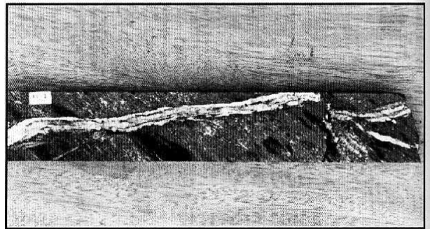
Calcite and chlorite vein cutting sulphided magnetitic breccia - Drill hole ALM-FD09.
