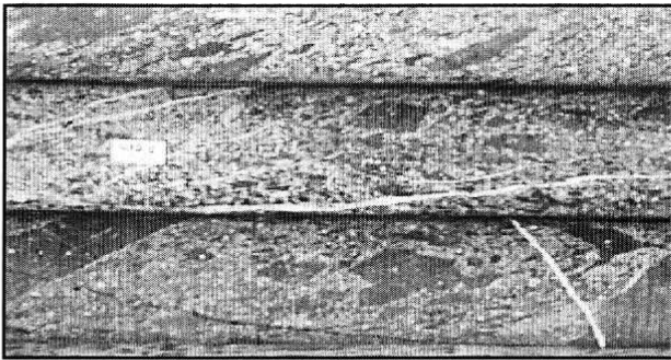
Metalapili tuff with fragments of quartz rich and metandesite -Drill hole ALM-FD34.
