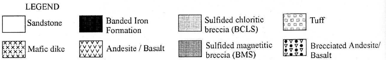
Figure 8 - Simplified lithological log with geophysical and geochemical data for diamond drill hole ALM-FD09.
