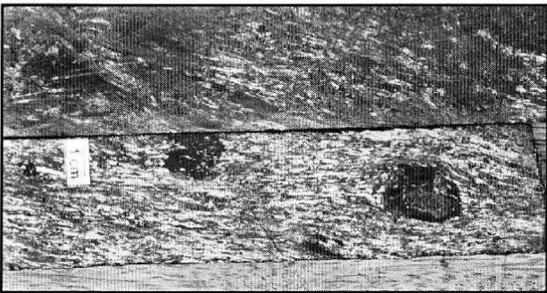
Sulphided magnetitic breccia fragments in a amphibol - chalcopyrite rich matrix - Drill hole ALM-FD09.
