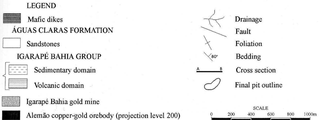
Figure 3 - Alemão Deposit and Igarapé Bahia Mine - Geological Map
