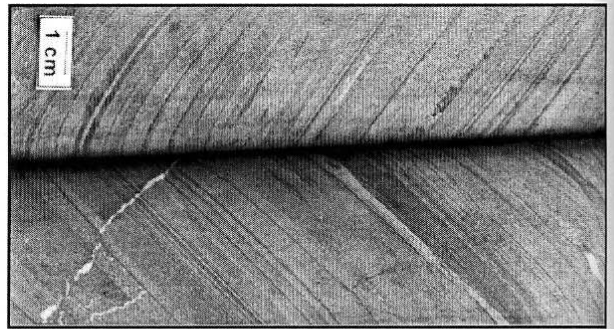
Metarhythmite with chalcopyrite - Drill hole BAHMAG-FD02.
