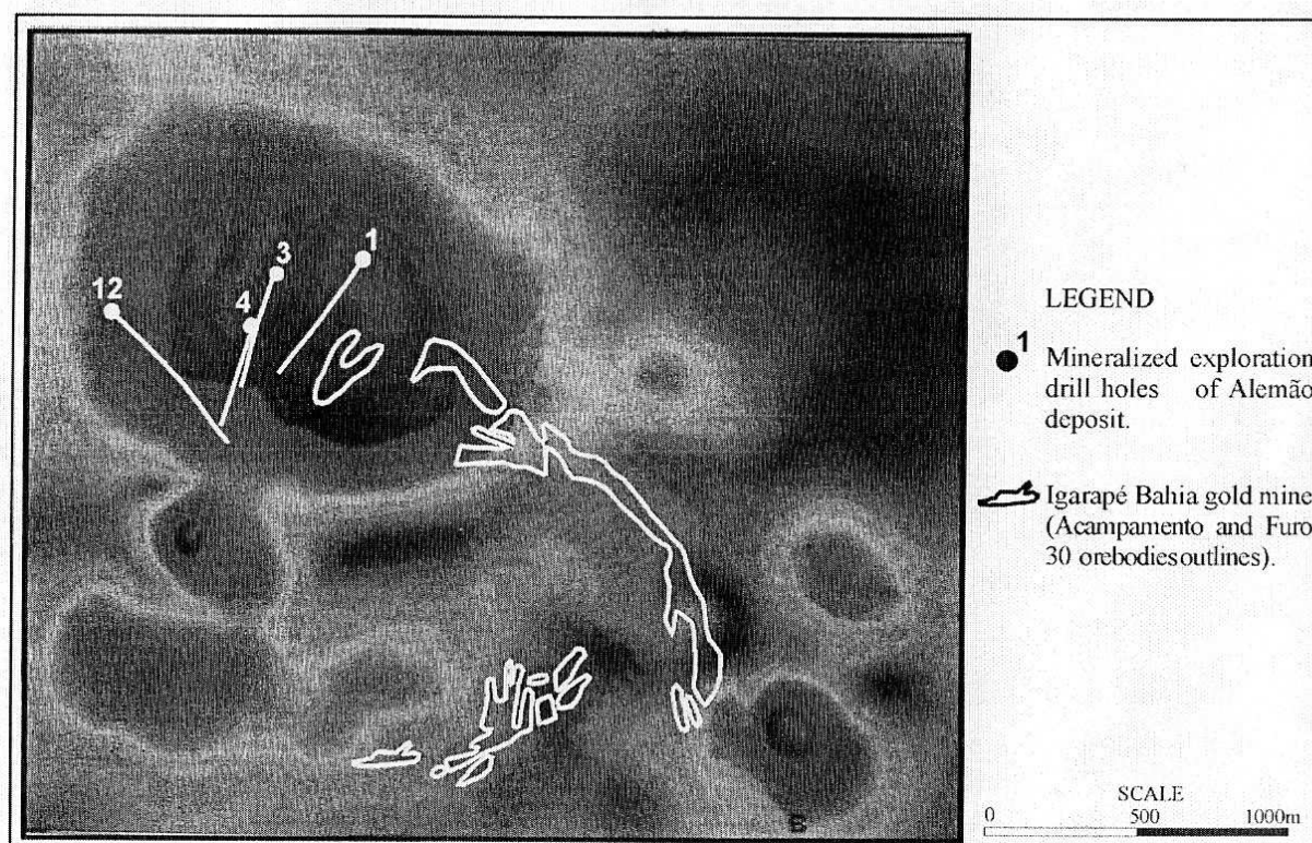
Figure 4 - Magnetic Anomaly of Alemão Deposit
