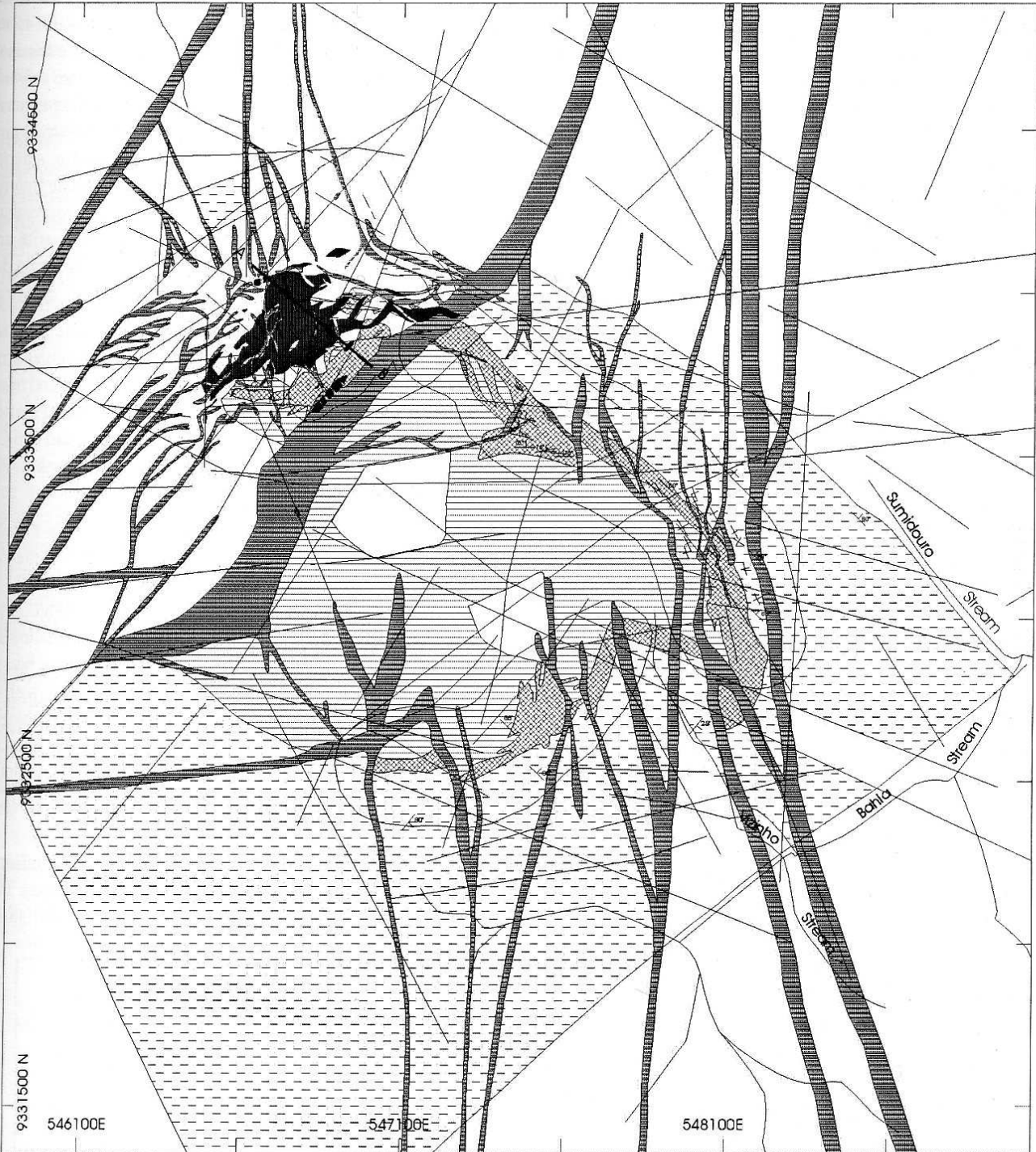
Figure 3 - Alemão Deposit and Igarapé Bahia Mine - Geological Map
