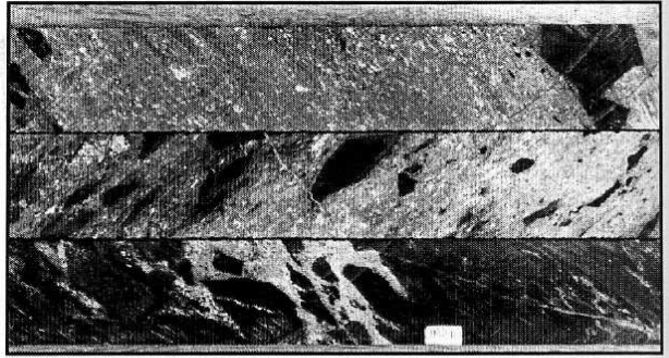
Sulphided magnetitic breccia fragments in a amphibole - chalcopyrite rich matrix - Drill hole ALM-FD09.
