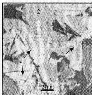
Figure 7 - BSE Images of Sulphided Chloritic Breccia and Sulphided Magnetitic Breccia of Alemão Deposit.
