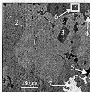
BSE image showing a ferropyrosmalite crystal (1) surrounded by siderite (2) with ankerite inclusions (3). Cut by discontinuous calcite (4) microveinlets: quartzo (5), monazite (6) and chalcopyrite (7). Drill hole ALM-FD 09.
