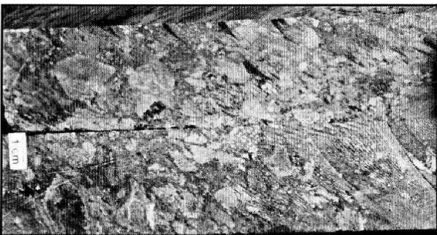
Metavolcanic fragments in a chlorite - bornite - chalcopyrite matrix (sulphided chloritic breccia) - Drill hole BAHMAG-FD01.
