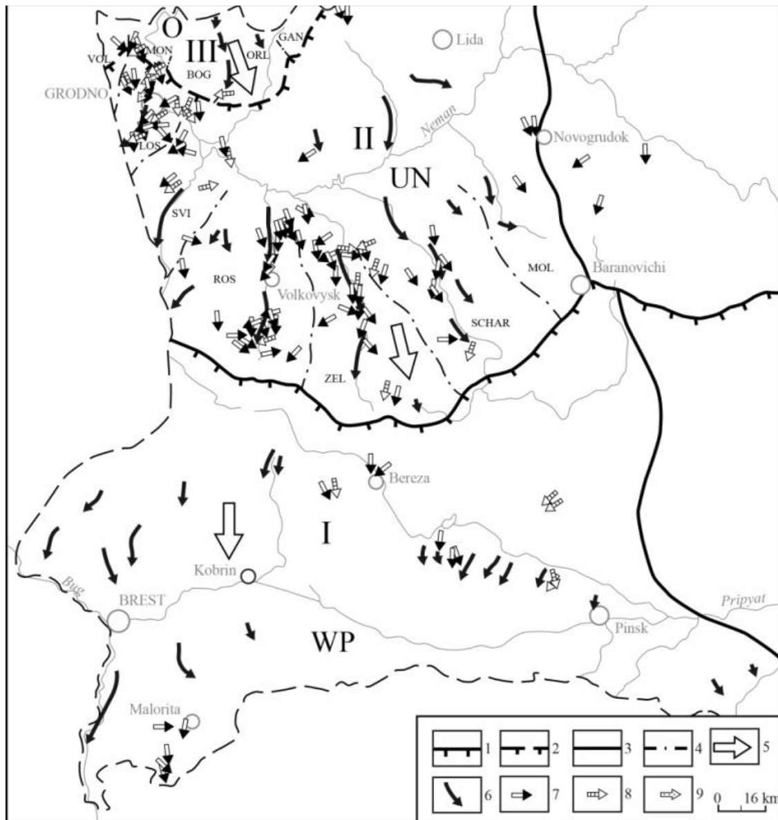
Fig. 1 Ice movement during the Pripjat and Poozerye glaciations within western Belarus
