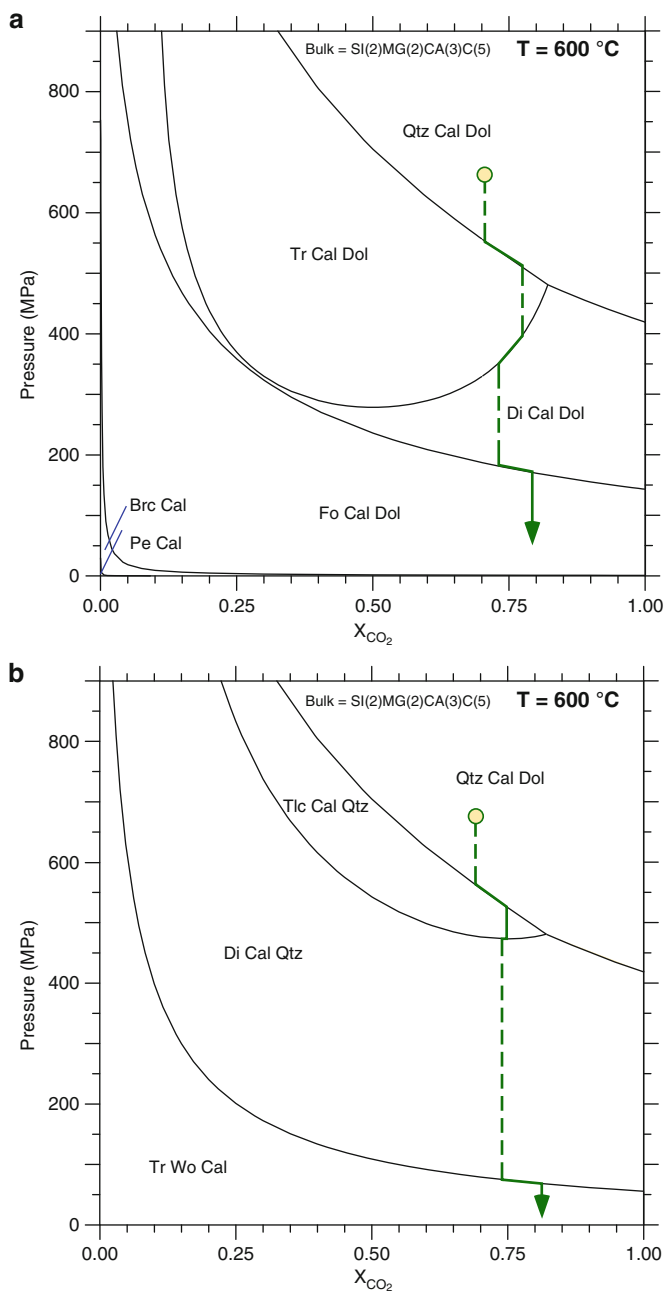
Fig. 6.15 P - a_{\text{CO}_2} phase relationships for (a) siliceous dolomites and (b) limestones (calcareous sandstone) at a constant temperature of 600^\circ\text{C} . On both figures: the stippled and arrowed path is followed by the respective rocks during isothermal decompression. It shows that high-grade assemblages in regional metamorphic marbles can be formed along late decompression paths
