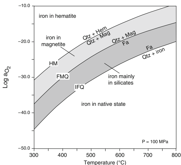
Fig. 3.20 Log oxygen activity– T diagram showing various oxidation states of iron in the system Fe–Si–O at 100 MPa. Oxygen buffered along curves by HM = hematite–magnetite; FMQ = fayalite–magnetite–quartz; IFQ = iron–fayalite–quartz. Standard state for \text{O}_2 : pure gas at T and 10^5 Pa
