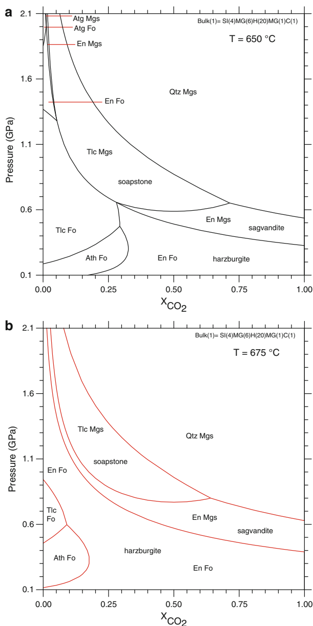
Fig. 5.15 Magnesite-bearing ultramafic rocks. (a) isothermal section at 650^\circ C : sagvandite = En + Mgs; soapstone = Tlc + Mgs; ophicarbonate = Atg + Mgs. (b) isothermal section at 675^\circ C . Note: the very different P-X-topologies at a \Delta T of only 25^\circ C . Harzburgite is not stable at mantle pressures in the presence of a fluid phase at T = 650^\circ C and below. At T = 675^\circ C , harzburgite may coexist with an extremely H_2O -rich fluid at mantle depth (it is not stable in the presence of CO_2 )
