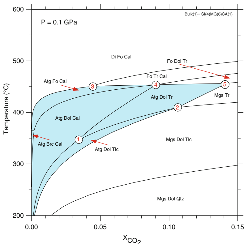
Fig. 5.12 Assemblage stability diagram for carbonate-bearing ultramafic rocks in the system CMS-HC at 100 MPa. The opficarbonate assemblages are shown in blue
