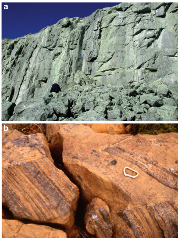
Fig. 5.1 (a) World largest olivine (dunite) mine, Almklovdaalen, Norway. Alpine type peridotite in Caledonian continental basement. The 8 m high bench in the quarry consists of coarse grained pure olivine (forsterite) rock. Note green color of fresh rock. (b) Layered peridotites in gabbro magma chamber. Leka Island, Norwegian Caledonides. Note typical yellow-brown weathering crust on peridotite matrix
