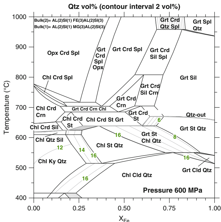
Fig. 7.17 Isobaric T - X_{Fe} section at 600 MPa showing the distribution of stable assemblages in metapelites in the FMASH system illustrating the Qtz-saturation problem. At T lower than the Ms breakdown boundary (thick gray shaded line) all assemblages include Ms, above that line they all contain Kfs. The bulk rock composition has sufficient SiO_2 that the low-grade rock contains ~ 17 mol% quartz ( X_{Fe} > 0.25 ). As a result of SiO_2 -consuming reactions free SiO_2 decreases (labeled vol% contours) and finally the rocks run out of free quartz (gray thick Qtz-out line at about 650°C). Note that corundum is present in various assemblages (Crm gneisses, Crm schists). Spinel is not present below 800°C
