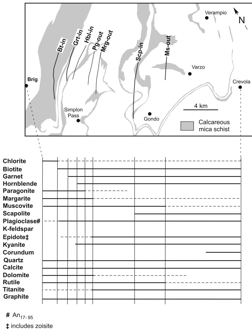
Fig. 8.5 Map showing distribution of calcareous mica schist, mineral-in and mineral-out isograds in calcareous mica schist of the Pennine Nappes, western Lepontine Alps, between Brig (Switzerland) and Crevola (Italy). Metamorphic grade increases from NW to SE (after Figs. 2 and 27 of Frank 1983). Mineral distribution in calcareous mica schist is shown below (modified after Fig. 3 of Frank 1983)
