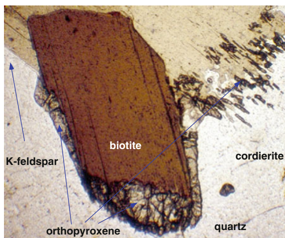
Fig. 7.14 Photomicrograph showing textural evidence for the biotite breakdown reaction \text{Bt} + \text{Qtz} = \text{Opx} + \text{Kfs} + \text{H}_2\text{O} in a granulite from the Gruf Complex, Central Alps (picture diagonal 2mm). The brown biotite crystal is encrusted by orthopyroxene (hypersthene). Biotite shows characteristic lobate resorption contacts to Opx showing that Bt is reactant and Opx is product of the reaction. Kfs and Qtz make up the gray matrix, where Kfs is in contact to Bt no Opx formed ( upper left corner ). The rock shows no structures that would indicate partial melting. The texture suggests low a_{\text{H}_2\text{O}} conditions (see text)
