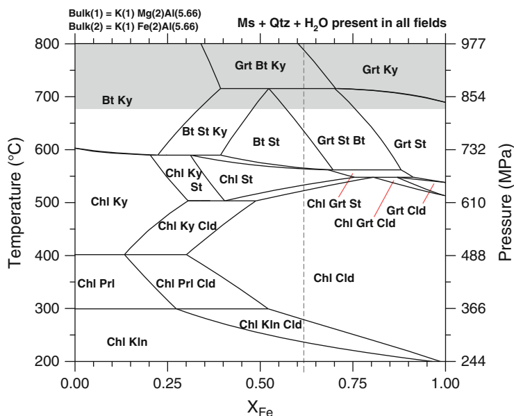
Fig. 7.7 Fe–Mg dependence of the distribution of stable assemblages in the system KFMASH along a Ky-type geotherm (continent collision type metamorphism). X_{Fe} of average pelites shown by dashed line . Note that the average pelite would define a mineral zone sequence: Cld, St, Bt, Grt, Ky, quite different from Fig. 7.1 because of different Al content of the rocks and probably also because of a different P – T path. The gray shaded area above 680°C marks the melt present region where Ms melts and is no longer present in the assemblage fields. Note that in very Mg-rich metapelites Chl–Ky decomposes not before middle amphibolite facies is reached (600°C) and that the highest grade assemblage is phlogopite + kyanite
