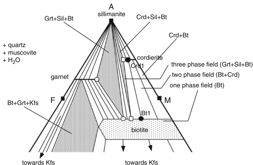
Fig. 2.12 AFM-diagram at a specified pressure and temperature showing phase relationships among some typical AFM phases
