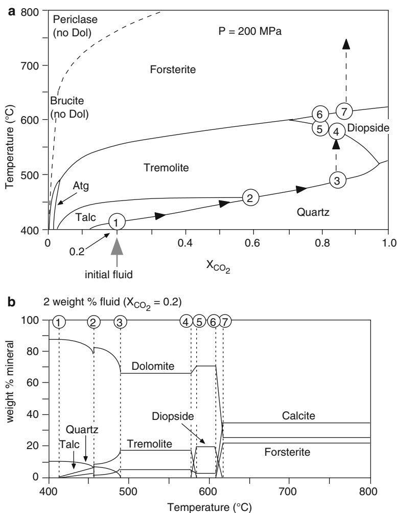
Fig. 3.27 A quantitative model for isobaric metamorphism of siliceous dolomites in terms of a quantitative isobaric T - X diagram (a) and a modal composition versus T diagram (b). The diagram has originally been calculated using the computer code EQUILAS written by Brown and Skinner (1974)
