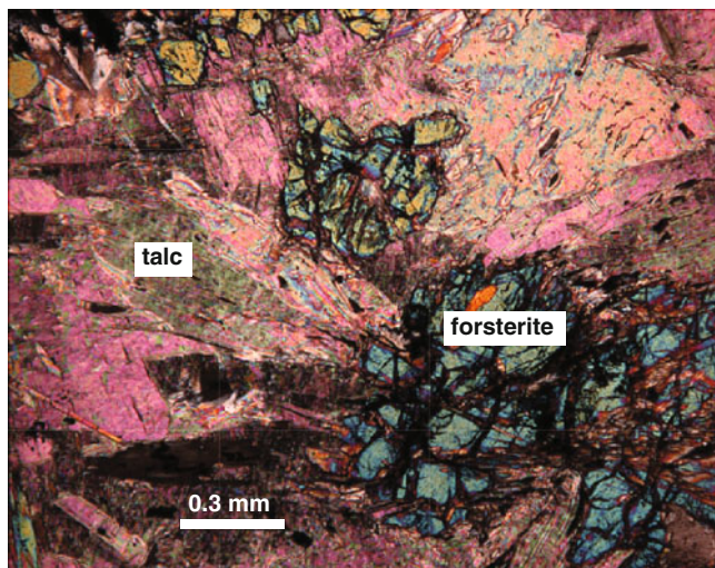
Fig. 5.16 Talcization of olivine by the open system reaction \text{Fo} + \text{SiO}_{2\text{aq}} + \text{H}_2\text{O} = \text{Tlc} . Murusjøen, N-Trøndelag, Norway
