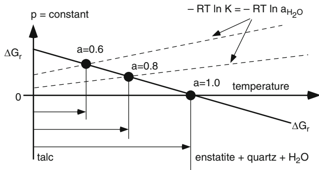
Fig. 3.15 Solutions of the equation \Delta G_r^0 = -RT \ln K for dehydration reactions and three different values of a_{H_2O}
