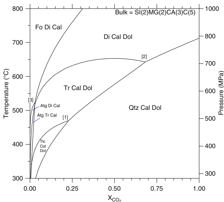
Fig. 6.5 P–T– a_{\text{CO}_2} diagram showing phase equilibria of siliceous dolomites for the composition 2\text{Qtz}+2\text{Dol}+1\text{Cal} (field 1b Fig. 6.4). The vertical axis represents an orogenic geotherm characteristic of regional metamorphism in collision belts
