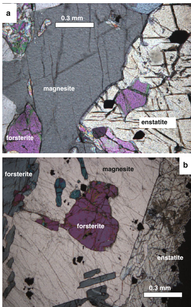
Fig. 5.14 Textural expression of the sagvandite reaction (5.24) (Table 5.2). Olivine reacts with \text{CO}_2 and binds the volatile into magnesite. Olivine is very strongly resorbed and product enstatite perfectly euhedral as a result of progress of carbonation reaction: \text{Ol} + \text{CO}_2 = \text{Mgs} + \text{En} . (a) Resorbed forsterite in euhedral enstatite, (b) Resorbed forsterite in magnesite. Ørnes sagvandite body, Nordland, Norway
