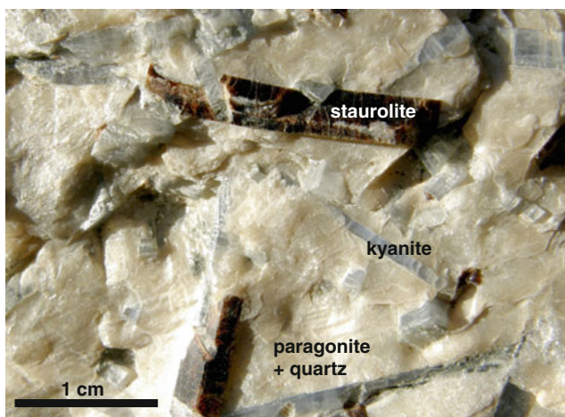
Fig. 7.10 Staurolite–kyanite schist from Alpe Sponda in the Ticino area of the Central Alps ( 5 \times 3 cm). The rock has been metamorphosed at about 600°C and 700 MPa (see Fig. 7.9) under amphibolite facies conditions during Tertiary continent collision. The rock also contains muscovite and paragonite and excess quartz
