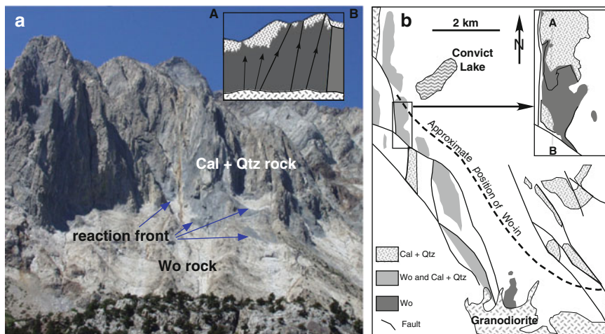
Fig. 6.13 Contact metamorphism and fluid infiltration of the Devonian Mt. Morrison formation (Ferry et al. 2001) (a) View from Convict Lake to the SW showing gray Cal + Qtz rocks in the upper portion of the mountain wall and white wollastonite rock at the base (Photograph Bucher). The two rocks are separated by a sharp reaction boundary (reaction (6.16); Table 6.1) which is driven by fluid infiltration. (b) Maps and section showing the occurrence of wollastonite in the Mt. Morrison quartz–calcite sandstone that forms part of a roof pendant within the Sierra Nevada batholith, California (simplified after Figs. 1 and 14 of Ferry et al. 2001). The N–S section line (A–B) of the cross section is indicated on the map. The cross section approximately corresponds to the picture 6.12a. Arrows in cross section indicate direction of fluid flow
