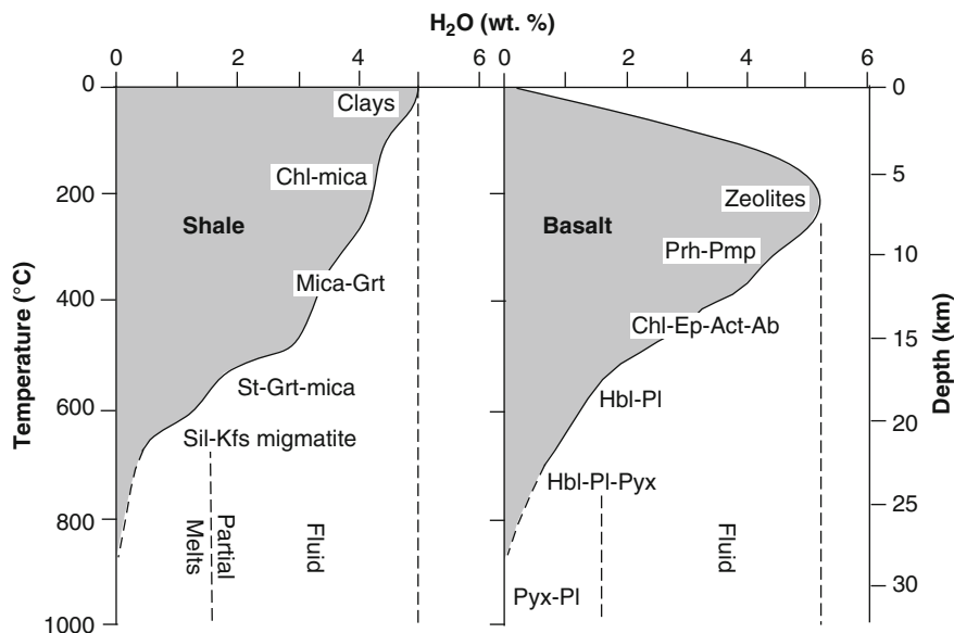
Fig. 3.14 Diagrams showing water-release curves of hydrous mineral assemblages during prograde dehydration reactions in shale and basalt along a 30^{\circ}C/km geotherm (Redrawn from Fyfe et al. 1978). Changes in the slopes of the water-release curves relate to the beginning and completion of dehydration of the main hydrous silicates. In the pelagic shale, partial melting to form migmatite can occur at \sim 620^{\circ}C depending on composition and remaining water content. Note that in the case of the basalt, which is essentially dry, hydration initially takes place to produce a zeolite facies assemblage with \sim 5 wt% H_2O . Partial melting of the basalt to form a mafic migmatite could occur at \sim 800^{\circ}C .
