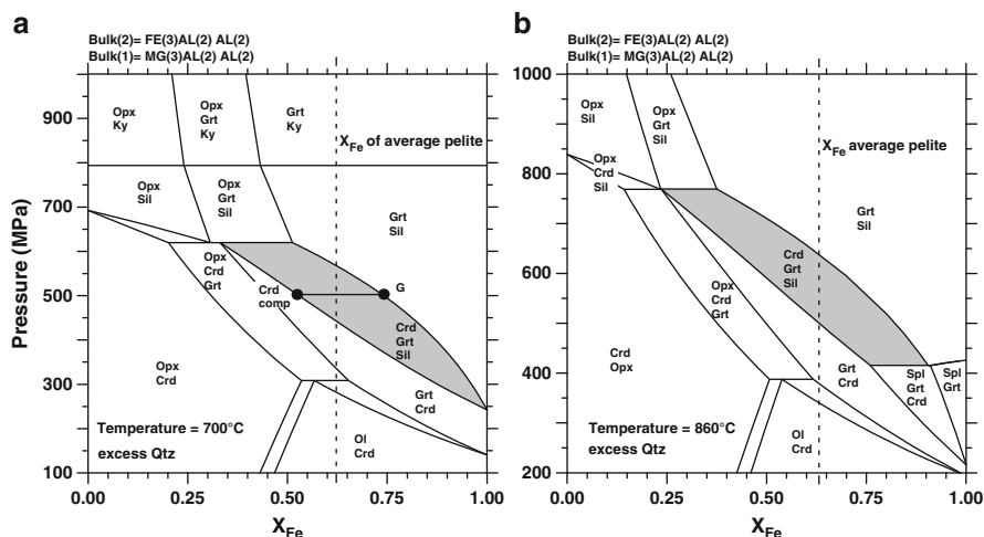
Fig. 7.16 Two isothermal P - X_{\text{Fe}} section: (a) at 700^\circ\text{C} (upper amphibolite facies) and (b) at 860^\circ\text{C} (granulite facies) showing the distribution of stable assemblages in metapelites in the FMASH system for high-grade metamorphism. All assemblages contain excess Qtz. At high X_{\text{Fe}} and low P Ol-Crd is the characteristic assemblage. The assemblage Opx-Crd occurs in low- X_{\text{Fe}} rocks over a wide range of pressures. The sequence of assemblages with progressively increasing pressure for metapelites with average X_{\text{Fe}} can be read from the dashed line. The assemblage Crd-Grt-Sil (gray shaded loop) can be used as a geologic barometer (see text). Grt-Als is stable over a very large P -range. In contrast: Opx-Als is a typical assemblage of lower crustal granulites
