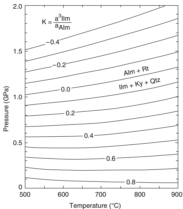
Fig. 4.14 \ln K contours for equilibrium conditions of the GRAIL reaction (Grt–Rt–Als (Ky)–Ilm–Qtz assemblage)
