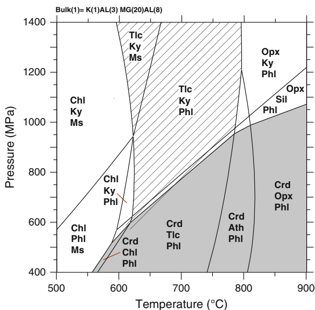
Fig. 7.23 Metamorphism of Mg-metapelites (Ms-Mg-Chl-Qtz): P - T diagram showing assemblages in the KMAH system for conditions of excess Qtz and \text{H}_2\text{O} . Mg-cordierite (gray shaded field) is present over a very large range of P - T (compare with Fig. 7.12). Mg-Crd extends to pressures in excess of 1 GPa in the granulite facies ( T > 800^\circ\text{C} ). Mg-Crd does not reach into the Ky-field. Ky present in Crd rocks may be metastable (see P - T path on Fig. 7.3). The characteristic whiteschist assemblage Tlc-Ky (diagonally ruled pattern) indicates lower crustal metamorphism (high-pressure amphibolite facies). Granulites with Opx-Als (Ky, Sil) imply P > 1 GPa. Rocks with Crd-Ath-Phl, widespread in shield areas, indicate upper amphibolite facies conditions at any pressure in the crust ( P up to 1 GPa)
