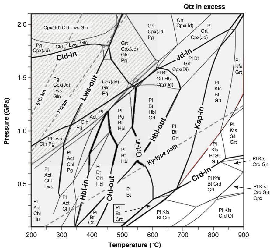
Fig. 10.2 Calculated equilibrium mineral assemblages in P - T space for a graywacke sandstone (granodiorite) composition ( \text{SiO}_2 – 73.83%; \text{Al}_2\text{O}_3 – 13.25%; \text{FeO} (total iron) – 3.37%; \text{MgO} – 1.16%; \text{CaO} – 1.41%; \text{Na}_2\text{O} – 3.10; \text{K}_2\text{O} – 2.53%). Mineral-in and -out “isograds” are highlighted. Shaded area indicates the stability field of K-white mica (Ms, Phe, Cel). Diagonally lined area = Gln stable. Quartz occurs with all mineral assemblages
