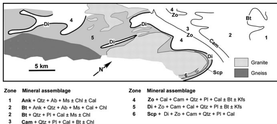
Fig. 8.2 Map showing distribution of mineral zones (numbered 1 to 6) and isograds (labelled) in metamarls of the Vassalboro Formation, south-central Maine (simplified after Fig. 1. of Ferry 1983c). Diagnostic zone mineral assemblages are listed below. Note that Pl compositions are: oligoclase-labradorite (upper Bt zone); andesine-anorthite (Cam, Zo, Di zones)
