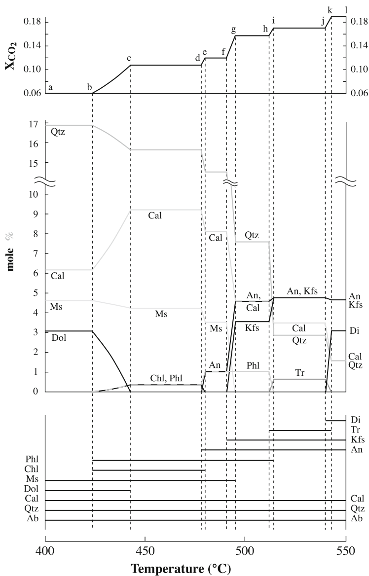
Fig. 8.4 Modal composition (mol%), fluid composition ( X_{\text{CO}_2} ) and mineral distribution along the prograde path “a–l” shown in Fig. 8.3
