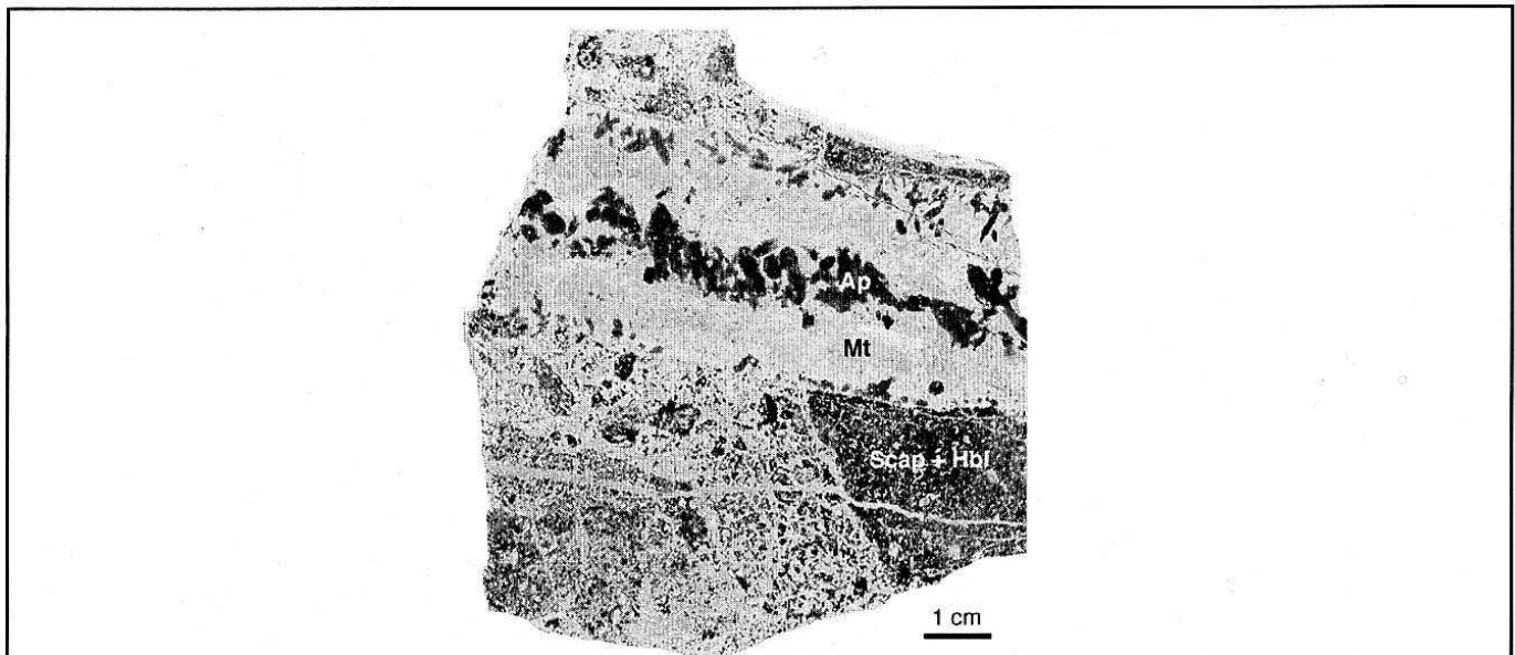
Figure 1. Hydrothermal magnetite-apatite-rich heterolithic breccias with Na scapolite + hornblende replacement of host basaltic rocks from the Jurassic-age Humboldt mafic complex, western Nevada (Johnson and Barton, 2000). This sample is representative of proximal/deep, REE-bearing, sulfide-poor assemblages found in many districts around the world. Distal to this material at Humboldt are numerous occurrences of hematite (/ magnetite) ± chalcopyrite (/ bornite) ± pyrite mineralization. The large Humboldt hydrothermal system (>900 km 3 Na ± Ca alteration; > 1 Gt Fe-oxide mineralization) represents an end-member in the overall spectrum of Fe-oxide deposits. The Humboldt system is fundamentally basaltic and has compelling geological and geochemical evidence for non-magmatic brine involvement with little if any magmatic aqueous fluid (Johnson, 2000). Such systems, which are part of a broader range from mafic to felsic, led us to postulate that non-magmatic brines can play a dominant role in some systems (Barton and Johnson, 1996; also discussion following).
