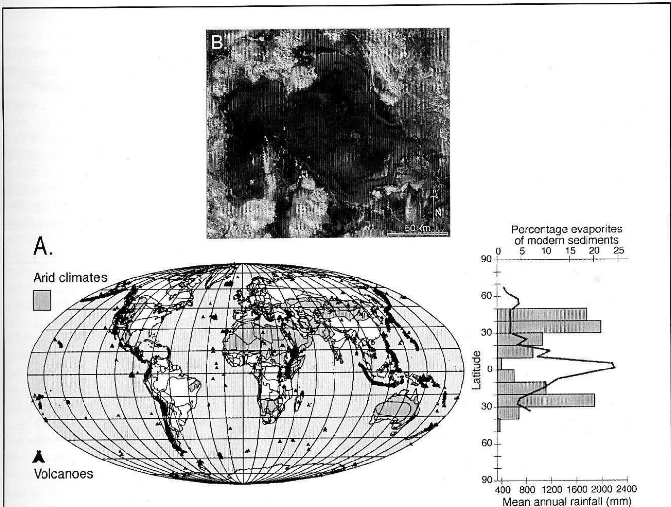
Figure 2 Overlap between modern magmatism, saline surface fluids and evaporites. A) Map showing modern climate and volcanism plus distribution of evaporitic sediments as a function of latitude. Neogene to modern Fe-oxide-rich systems occur where magmatism overlaps with arid climates (cf. Barton and Johnson, 1996). B) TM image of the Salar de Uyuni, Bolivia. Note the many modern volcanoes in the western half of the image. This area contains a number of young igneous- and sediment-hosted Cu and Fe-oxide occurrences (U.S. Geological Survey, 1992).
