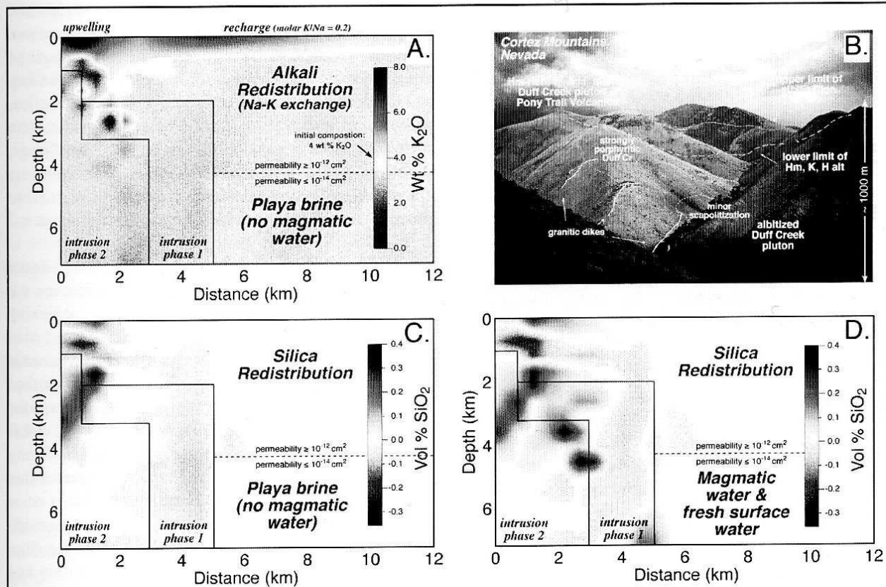
Figure 7. K-Na exchange and silica mass transfer results for numerical models of energy and mass transport in brine systems of various types (Hanson, 1995; Barton et al., 1998). The models have the same permeability structure and the same two-stage intrusion emplaced on the left. The left boundary is symmetric. A) Alkali redistribution in felsic rocks. Note (1) the laterally extensive K_2O -rich rocks where brines recharge (this will be oxidized, low-T potassic alteration), (2) the abundant Na_2O alteration (stippled) at depth, and (3) the intense concentrated K_2O addition where the brines rise toward to the surface (second type, with Fe oxides and (presumably) other ore minerals). B) An example of alteration like that modeled in (A). Photo showing shallow hematite and K-silicate-altered felsic volcanic + hypabyssal rocks (with minor Fe-oxide-Cu-Au mineralization) overlying sodically altered granitoids. Jurassic igneous complex, Cortez Mountains, Nevada. C) Silica redistribution in system with external brine. Note concentration in upwelling zone over center of intrusion and dispersed zone of leaching (stipple). D) Similar diagram showing silica redistribution for a combination of magmatic fluids and fresh water. The larger silica addition in (D) compared to (C) is due mainly to magmatic fluids.
