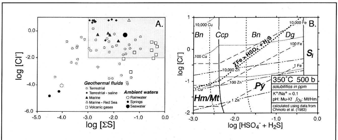
Figure 4. Log [Cl^-] vs. log [\Sigma S] plots (molality) illustrating some natural waters and metal solubilities. A) Compositions of modern fluids grouped by environment, mostly from geothermal systems. Compiled from various sources. B) Calculated Cu-Fe-S-O sulfide and oxide mineral stabilities and Fe, Cu, and Zn solubilities (in ppm; Zn buffered by sphalerite) as a function of fluid chloride and sulfur contents at 350°C (modified from Barton and Johnson, 1996). Same area as the inset in (A).
