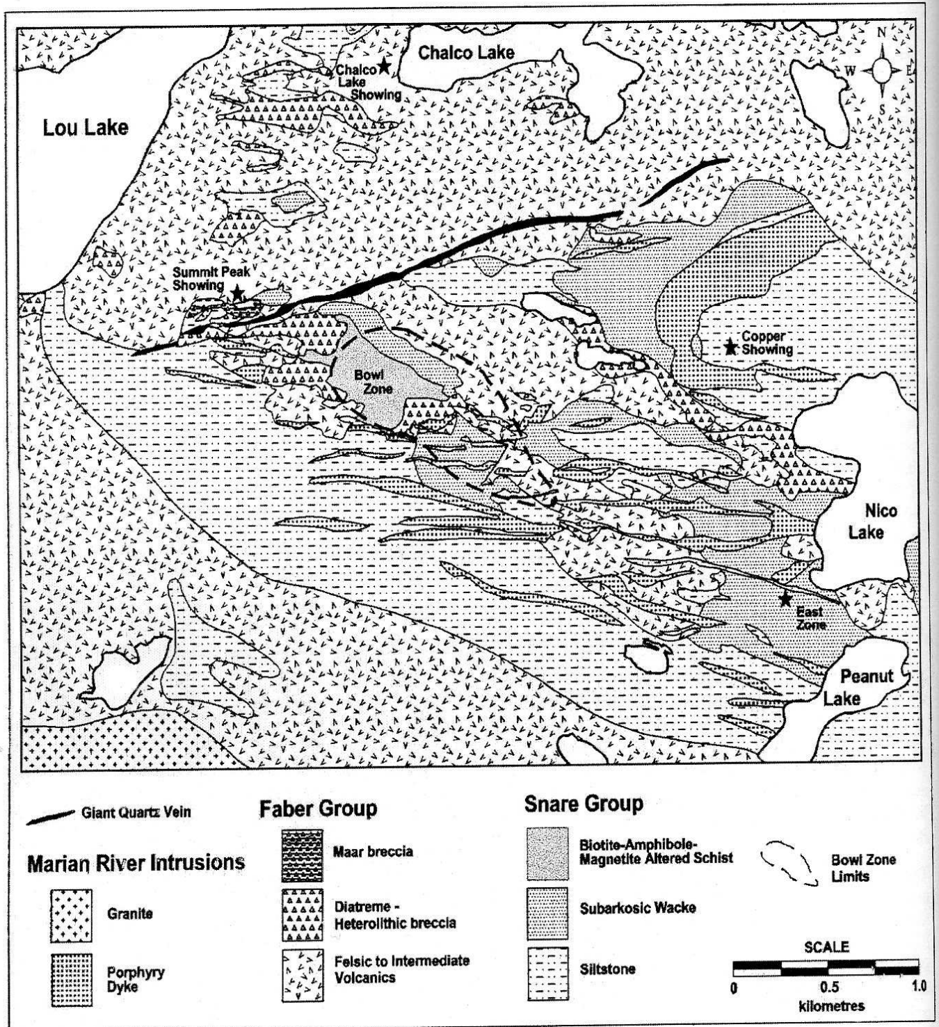
Figure 3. Geology of the central NICO claims and the Bowl Zone deposit.
