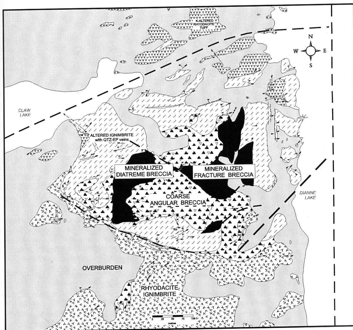
Figure 6. Geology of the Sue-Dianne copper-silver-gold iron oxide-rich breccia complex.
