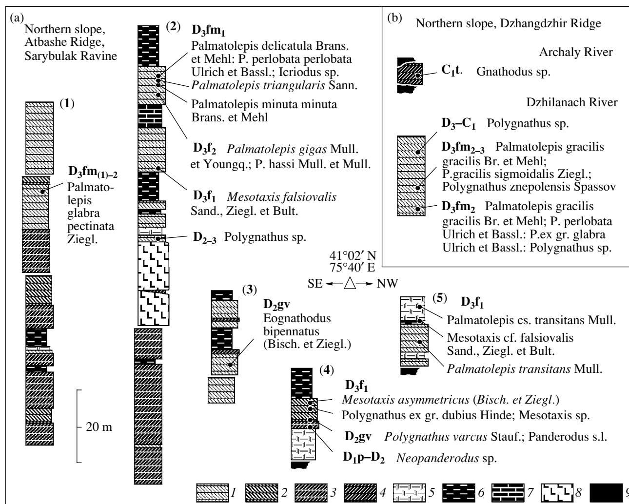
Fig. 3. Stratigraphic columns and conodont identifications. (1) Green cherts; (2) brown cherts; (3) sealing-wax jasperoids; (4) phantites; (5) siliceous shales; (6) mudstones and cherts; (7) limestones; (8) basalts; (9) serpentinites. Zonal forms in conodont lists are given in italics.
