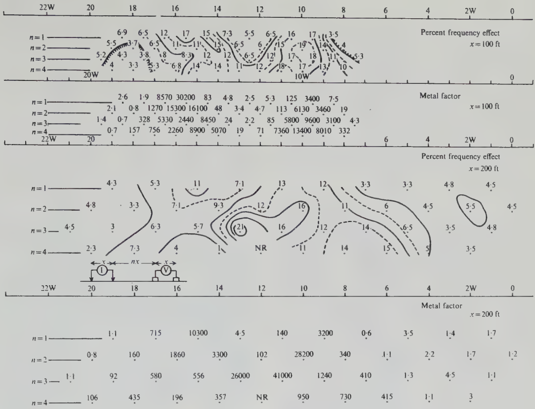
Figure 9.24. Pseudodepth plots for frequency-domain IP, western Ontario.
