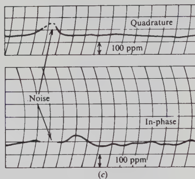
Figure 7.121. Airborne phase-component EM profiles. (a) Helicopter survey, transmitter frequency 400 Hz. (b) As in (a) for 320 Hz. (c) Fixed-wing aircraft, transmitter frequency 390 Hz.
