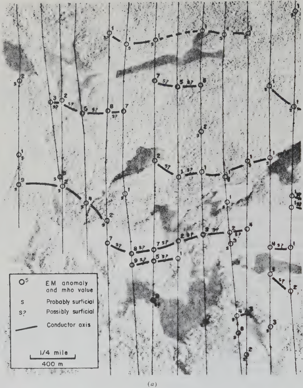
Figure 7.85. Resistivity map as an aid in distinguishing bedrock from overburden anomalies. (After Fraser, 1978.) (a) Airborne EM map showing conductor pattern similar to that for conductive overburden.
