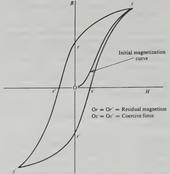
Figure 3.2. Hysteresis loop. s, s' = saturation, r and r' = remanent magnetism, c and c' = coercive force.
