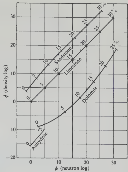
Figure 11.42. Porosity cross-plot. (Courtesy Schlumberger Ltd.)
