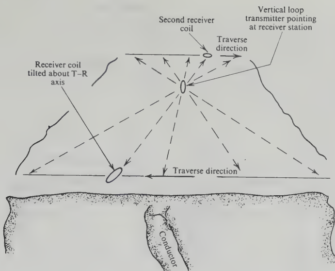
Figure 7.14. Dip-angle system, fixed transmitter.
