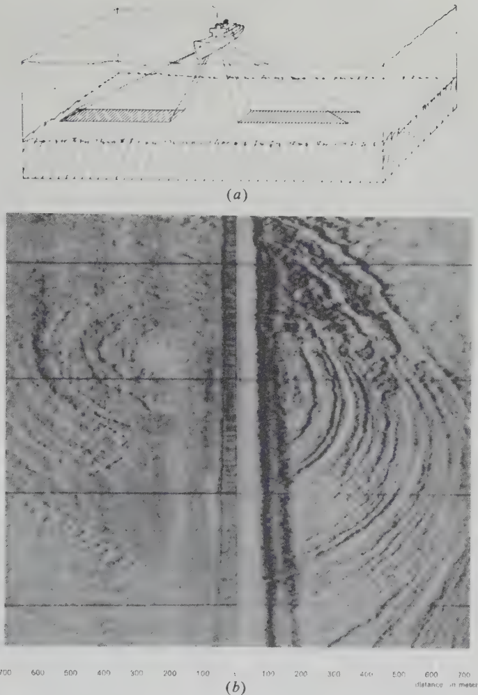
Figure 4.110. Side-scan sonar. (Courtesy Compagnie Générale de Géophysique.) (a) Schematic diagram. (b) Record showing reflections from sea-floor relief. There is a blind zone under the ship's track.
