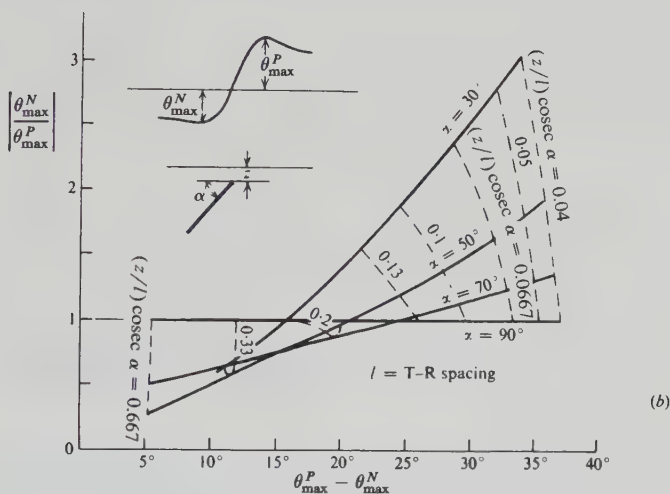
Figure 7.42. Characteristic curves for semiinfinite dipping-sheet conductor. (a) Depth to the top of a steeply dipping sheet from the crossover slope and peak tilt. Broadside array. (From Ward, 1967.) (b) Depth and dip using fixed-transmitter, dip-angle system. (From Grant and West, 1965.)
