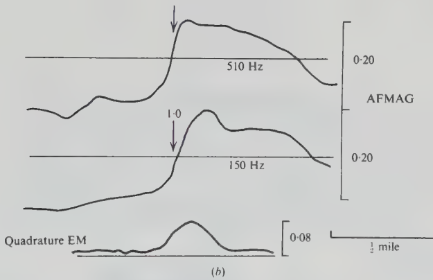
Figure 7.107. Comparison of various airborne EM systems and aeromagnetics, Whistle Mine, Sudbury, Ontario. (a) Comparison of VLF, quadrature EM, and aeromagnetics. (b) AFMAG and quadrature EM on the same line as (a). (From Ward, 1959b.)
