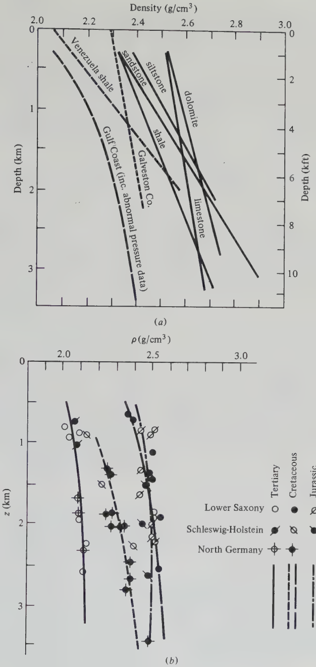
Figure 2.7. Density versus depth. (a) Western Hemisphere data: Venezuelan data from Hedberg (1936), Gulf Coast data from Dickenson (1953), Galveston County data from Bible (1964), and remaining data (Canadian) from Maxant (1980). (b) North Europe data from Hermes (1986).
