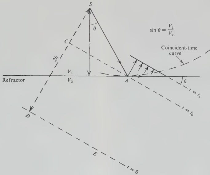
Figure 4.120. Deriving the properties of the coincident-time curve.
