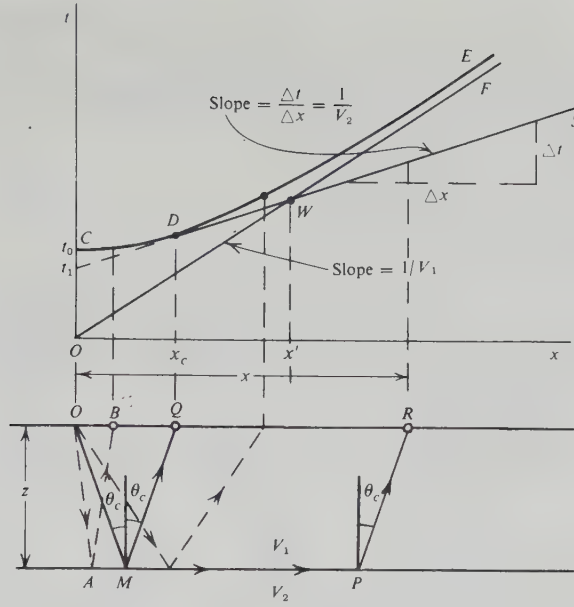
Figure 4.31. Relation between reflection and refraction raypaths and traveltime curves.
