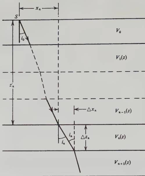
Figure 4.29. Raypath where velocity varies with depth.
