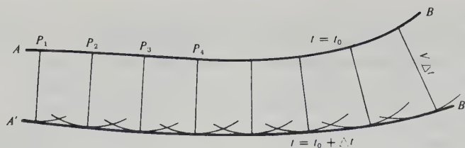
Figure 4.11. Using Huygens' principle to locate new wavefronts.
