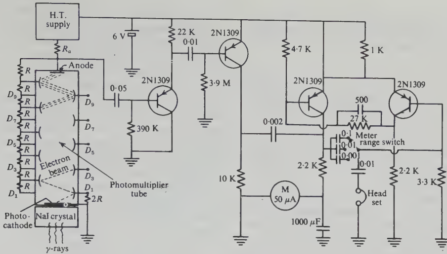
Figure 10.5. Scintillation-meter schematic.
