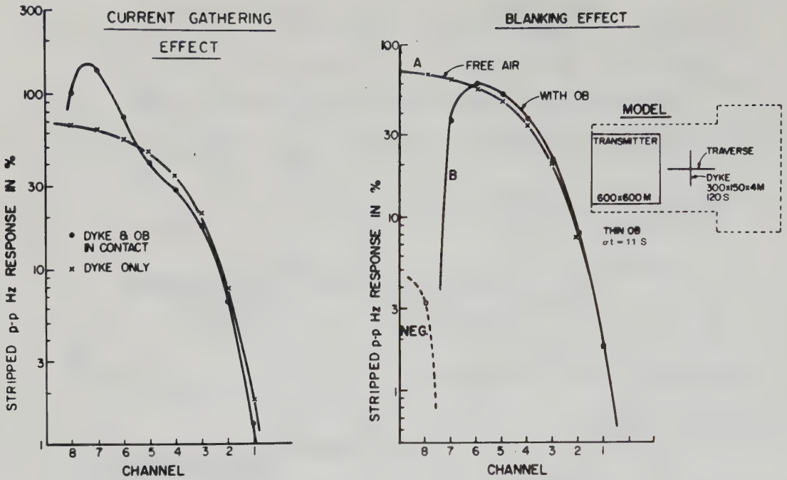
Figure 7.64. Decay plots for the H_z^5 anomalies of Figure 7.63. (After West, Macnae, and Lamontagne, 1984.)
