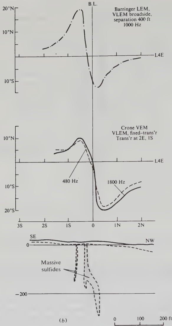
Figure 7.95. (Continued) (b) VLEM profiles and ore section.
