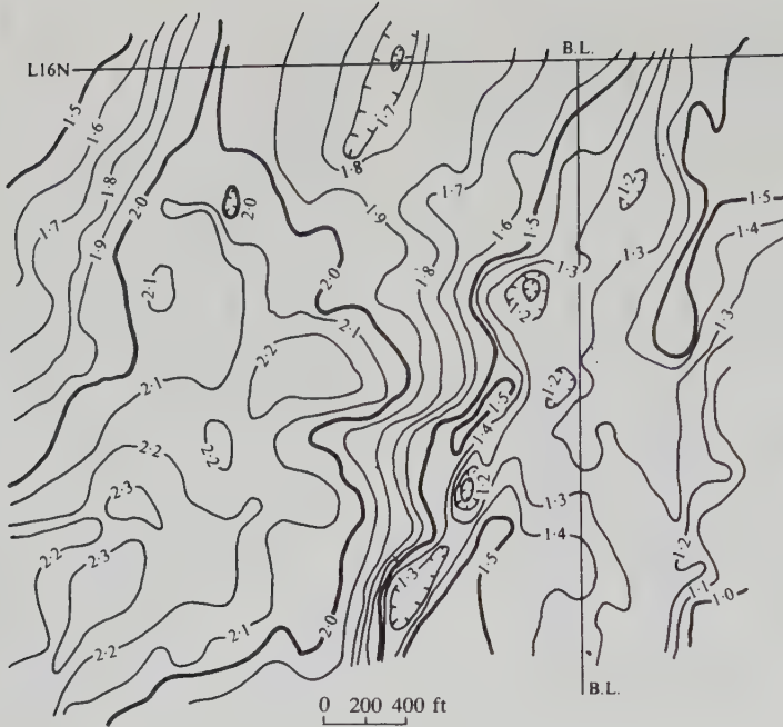
Figure 2.43. Bouguer gravity contours, eastern Nova Scotia; C.I. = 0.1 mGal.
