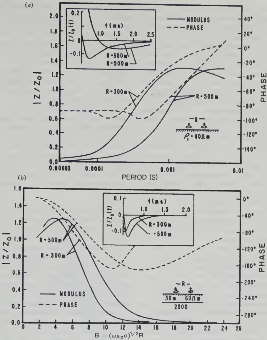
Figure 7.75. Modulus and phase of the mutual coupling ratio in the frequency domain and time domain (small insert) for the horizontal coplanar loop system [Eq. (7.41a)]. (After Patra and Mallick, 1980.) (a) Homogeneous earth. (b) Two-layer earth.
