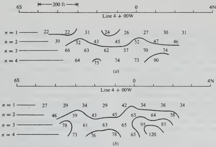
Figure 8.48. Apparent resistivities ( \rho_a/2\pi \Omega\text{ft} ) from two IP surveys using a double-dipole array with separation 100 ft. (a) Data from frequency-domain IP. (b) Data from time-domain IP.
