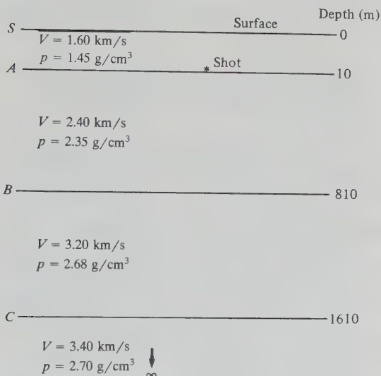
Figure 4.123. Horizontal layering situation.
