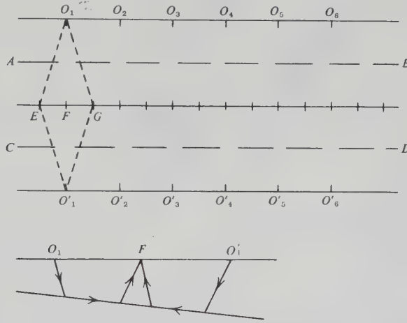
Figure 4.71. Broadside refraction profiling.
