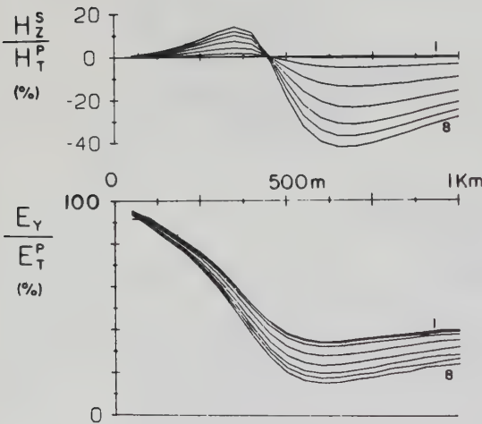
Figure 7.65. Model UTEM magnetic ( H_z ) and electric ( E_y ) responses over a vertical-plate conductor along the x axis. Tx loop = 1 \times 1 km, conductor = 1 \times 0.5 km, Tx 450 m to right of plate, z = 110 m, TCP = 20 S. (After West, Macnae, and Lamontagne, 1984.)
