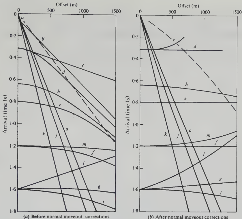
Figure 4.36. Types of events on a seismic record. Identities of events are: a = direct wave, V = 650 m/s; b = refraction at base of weathering, V_H = 1,640 m/s; c = refraction from flat refractor, V_R = 4,920 m/s; d = reflection from refractor c, V_{av} = 1,640 m/s; e = reflection from flat refractor, V_{av} = 1,970 m/s; f = reflection from flat refractor, V_{av} = 2,300 m/s; g = reflection from dipping reflector, V_{av} = 2,630 m/s; h = multiple of d; i = multiple of c; j = ground roll, V = 575 m/s; k = air wave, V = 330 m/s; l = reflected refraction from in-line disruption of the refractor c; m = reflected refraction from broadside disruption of refractor c. After normal-moveout correction, primary reflections are straight. In processing, data are usually muted, that is, data earlier than that indicated by the dashed lines are set to zero so that the data in the upper right corner do not appear.
