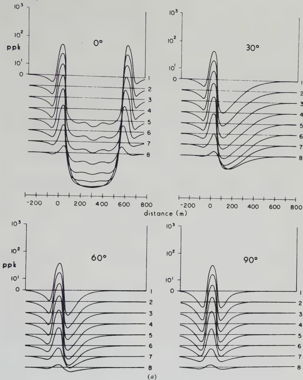
Figure 7.50. PEM(1) response to a dipping sheet as a function of dip, depth, and TCP. \ell = d = 600 m, T-R = 100 m, TCP = \sigma t = 30 S [except in (d)]. (After Bartel and Hohmann, 1985.) (a) Effect of dip; z = 50 m.
