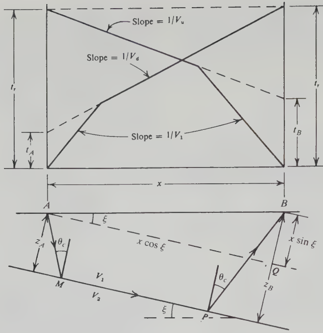
Figure 4.33. Raypaths and traveltime curves for a dipping refractor.
