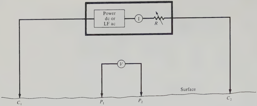
Figure 8.16. Schematic of equipment for measuring resistivity.
