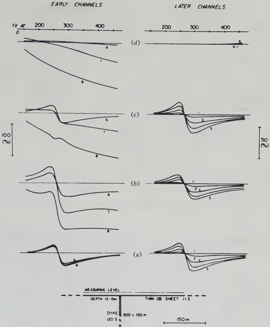
Figure 7.63. Model UTEM H_z^2 profiles over a vertical conductive sheet under a thin conductive overburden. (After West, Macnae, and Lamontagne, 1984.) (a) Effect of sheet alone. (b) Sheet in contact with the overburden. (c) Sheet not in contact with overburden. (d) Overburden alone.
