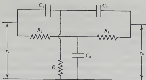
Figure 7.13. Twin-T network for EM receivers. \omega^2 = 1/(2C_1^2R_1R_2) = 2/(C_2C_2R_2^2) . Generally R_2 \approx 2R_1 , C_2 \approx 2C_1 for convenience in design.
