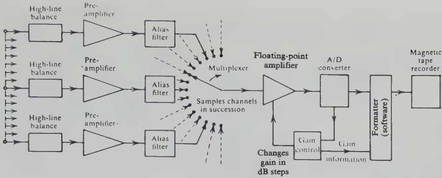
Figure 4.58. Block diagram of digital seismic amplifier.
