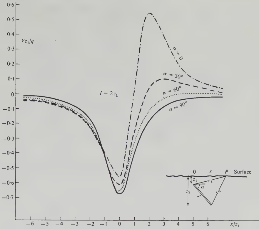
Figure 6.5. SP profiles over buried polarized rod.
