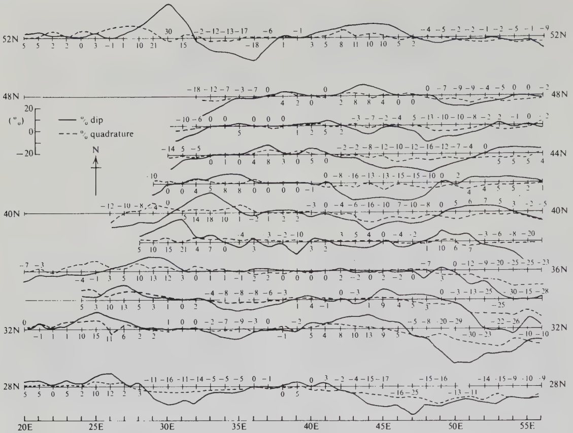
Figure 7.109. EM16 survey in eastern Nova Scotia.
