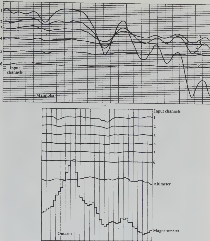
Figure 7.122. Airborne Input EM records.
