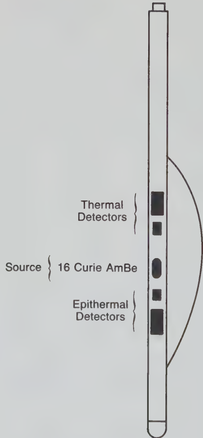
Figure 11.38. Schematic of dual-porosity neutron-logging sonde. (From Schlumberger, 1987.)
