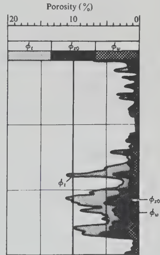
Figure 11.43. Moveable oil plot. (Courtesy Schlumberger Ltd.)
