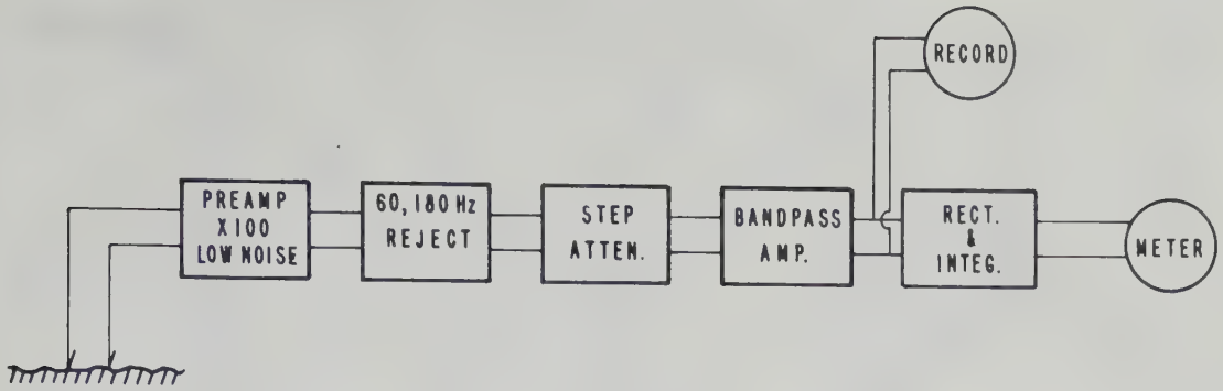
Figure 6.15. Schematic of telluric unit for audio and subaudio frequencies.
