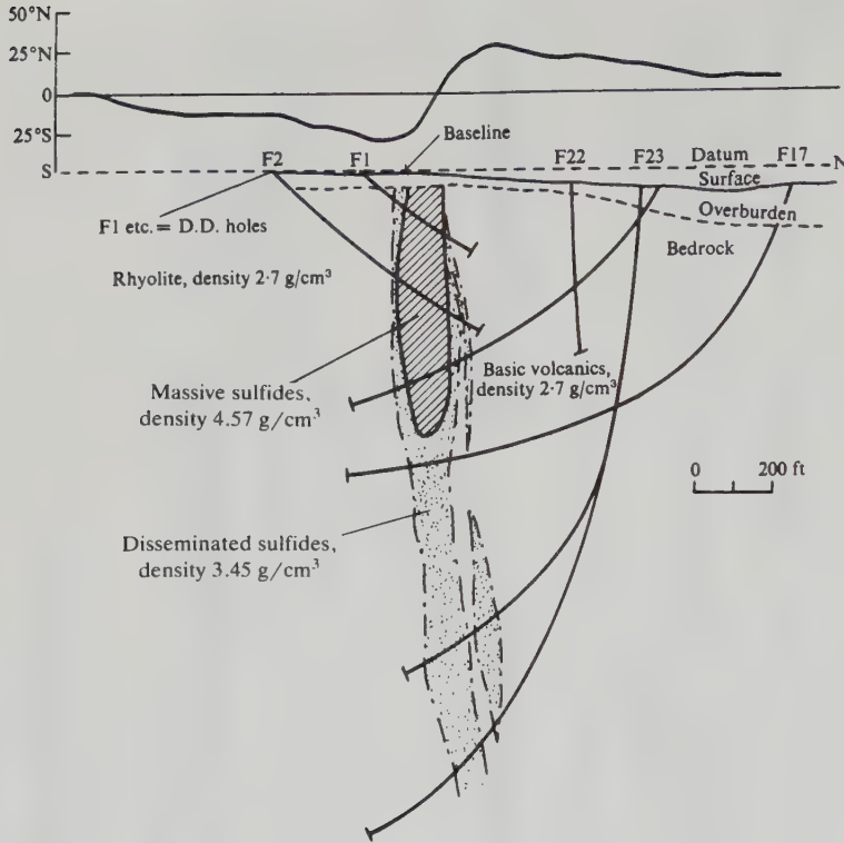
Figure 7.94. Vertical-loop fixed-transmitter profiles over Mobern orebody. (After Seigel, 1957.)
