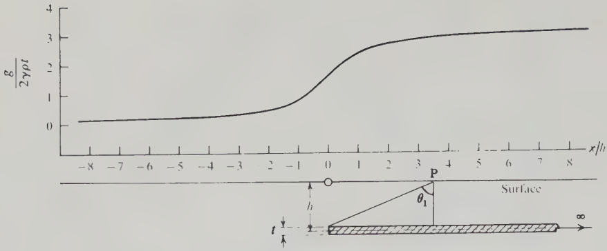
Figure 2.28. Gravity effect of a semiinfinite horizontal sheet.
