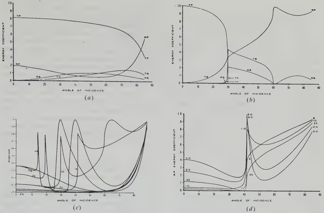
Figure 4.17. Partitioning of energy between transmitted and reflected waves as a function of angle of incidence for the case of an incident P wave. TP = fraction of energy in transmitted P wave, RP = fraction in reflected P wave, TS = fraction in transmitted S wave, and RS = fraction in reflected S wave. (From Tooley, Spencer, and Sagoci, 1965.) (a) Case where velocity in the incident medium is larger: \alpha_2/\alpha_1 = 0.5 , \rho_2/\rho_1 = 0.8 , \sigma_1 = 0.3 , and \sigma_2 = 0.25 . (b) Case where velocity in the incident medium is smaller: \alpha_2/\alpha_1 = 2.0 , \rho_2/\rho_1 = 0.5 , \sigma_1 = 0.3 , and \sigma_2 = 0.25 . (c) Fraction of energy reflected as P wave for various P-wave velocity ratios and \rho_2/\rho_1 = 1.0 , \sigma_1 = \sigma_2 = 0.25 (from Denham and Palmeira, 1984). (d) Fraction of energy reflected as a P wave for various density ratios and \alpha_2/\alpha_1 = 1.5 , \sigma_1 = \sigma_2 = 0.25 .
