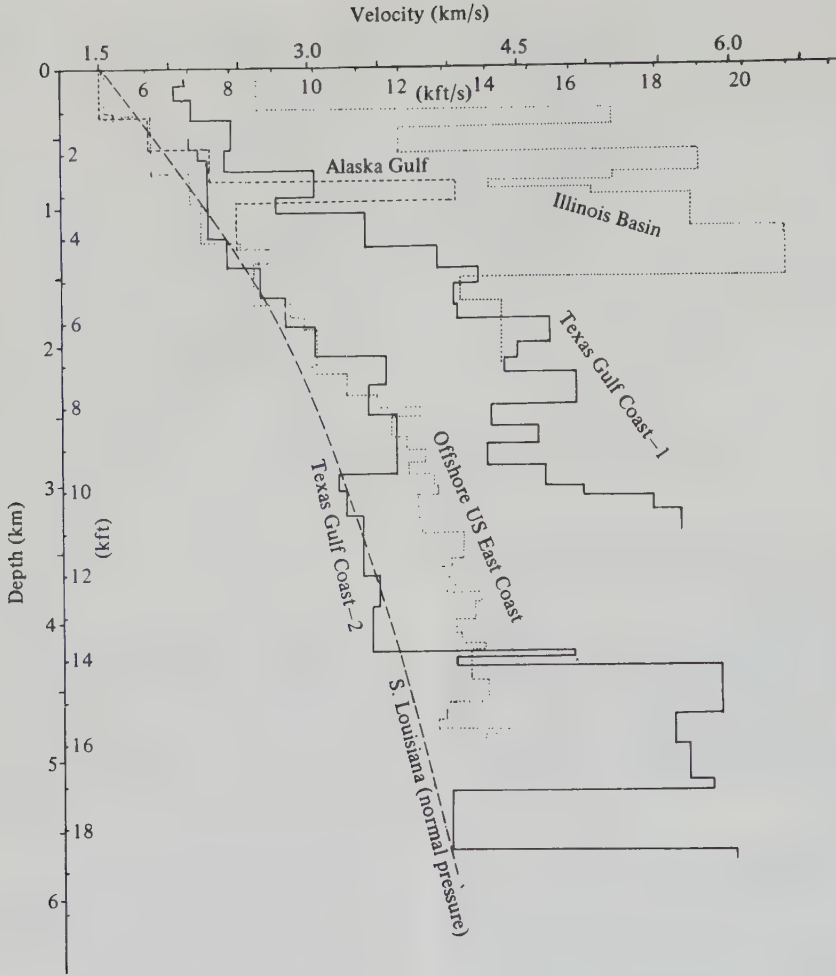
Figure 4.19. Velocity–depth relationships from selected wells. (From Sheriff and Gelfart, 1983.)
