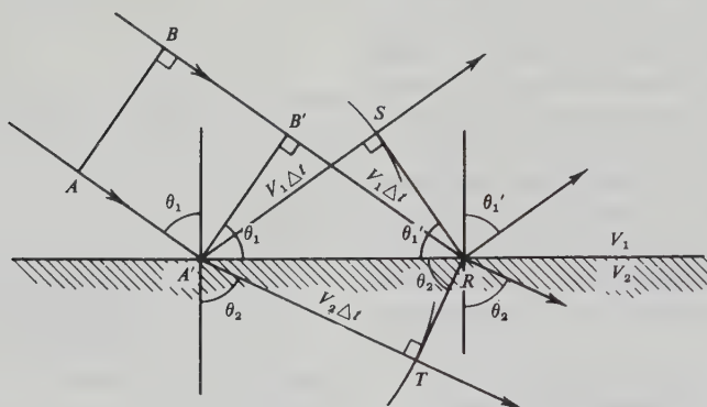
Figure 4.12. Reflection and refraction of a plane wave.
