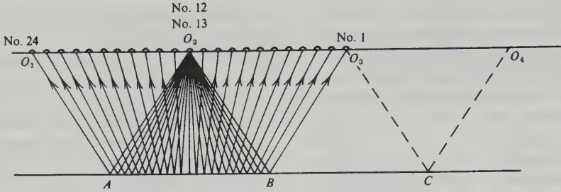
Figure 4.45. Symmetrical spread with continuous subsurface coverage.
