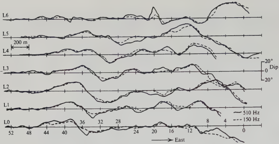
Figure 7.111. AFMAG profiles, northeastern Brazil.
