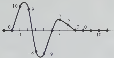
Figure 4.124. A minimum-phase wavelet.
