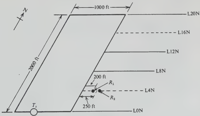
Figure 7.114. Model Turam configuration.
