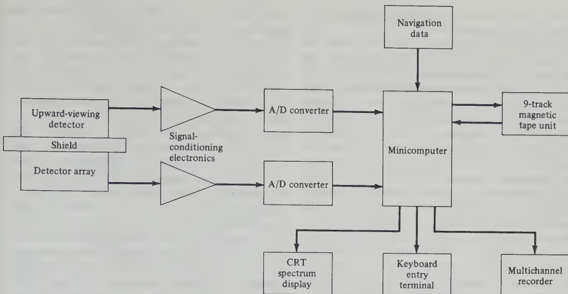
Figure 10.9. Modern \gamma -ray spectrometer. (After Bristow, 1979.)
