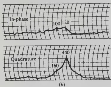
Figure 7.121. Airborne phase-component EM profiles. (a) Helicopter survey, transmitter frequency 400 Hz. (b) As in (a) for 320 Hz. (c) Fixed-wing aircraft, transmitter frequency 390 Hz.
