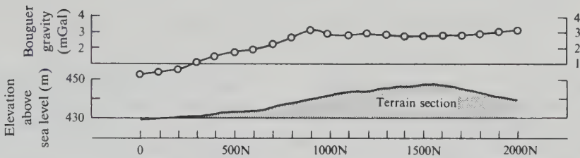
Figure 2.42. Bouguer gravity and topographic profiles, East Africa.
