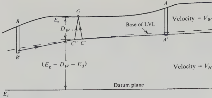
Figure 4.75. Datum correction for geophone between shotpoints.
