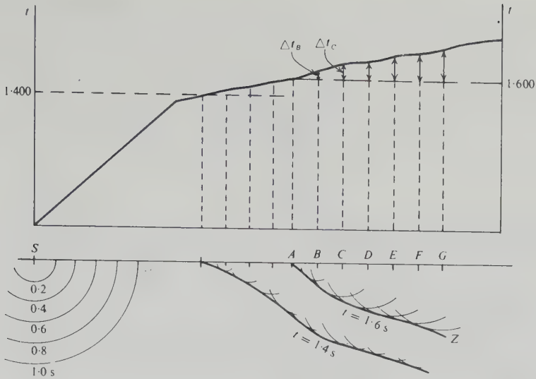
Figure 4.91. Reconstruction of wavefronts.
