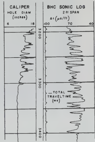
Figure 11.25. Portion of a sonic log. (From Schlumberger, 1987.)
