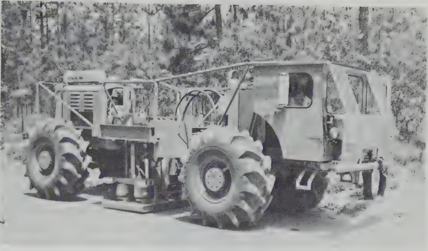
Figure 4.52. Vibrators mounted for off-road survey. (Courtesy Conoco.)
