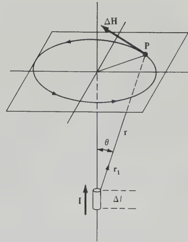
Figure 3.1. Ampère's law. A current \mathbf{I} through a length of conductor \Delta l creates a magnetizing field \Delta \mathbf{H} at a point P :
