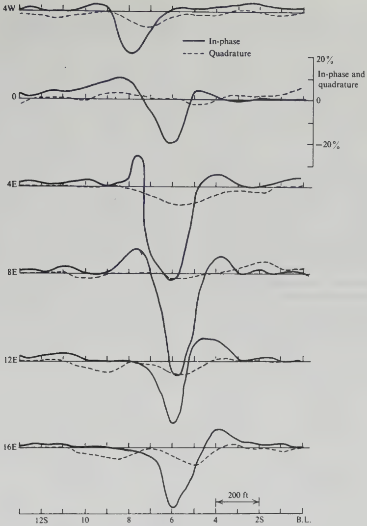
Figure 7.113. HLEM profiles, Chibougamau Area, Quebec.
