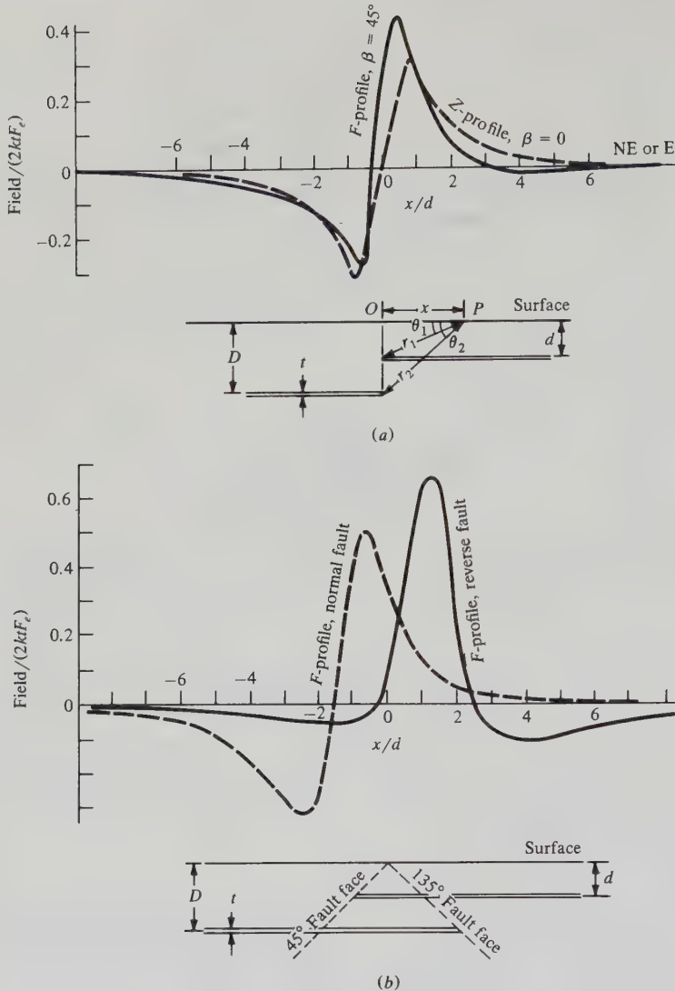
Figure 3.23. Thin-sheet fault approximation; D = 2d , I = 60^\circ . (a) F, Z profiles for vertical faults striking N-S and SE-NW ( \beta = 0^\circ, 45^\circ ). (b) F profiles for normal and reverse faults striking E-W; fault dip 45^\circ, 135^\circ .
