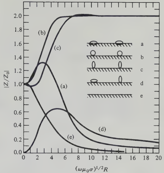
Figure 7.72. Mutual impedance ratios for systems (a) to (e) in Equation (7.41) as a function of (\omega\mu\sigma)^{1/2}R . (After Wait, 1955.)
