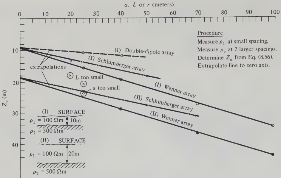
Figure 8.39. Graphical determination of overburden thickness using one small spread to get \rho_1 and two large spreads to get \rho_a .
