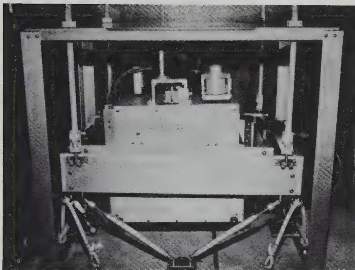
Figure 2.16. Photograph of a shipboard gravimeter.
