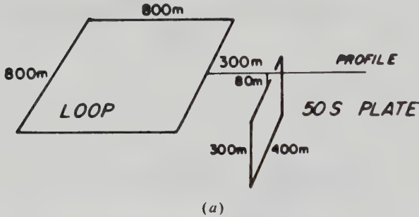
Figure 7.61. UTEM profiles over a dipping-plate model. (After West, Macnae, and Lamontagne, 1984.) (a) Geometry and dimensions of the model, and configuration of the primary field in the vicinity of the conductive plate.
