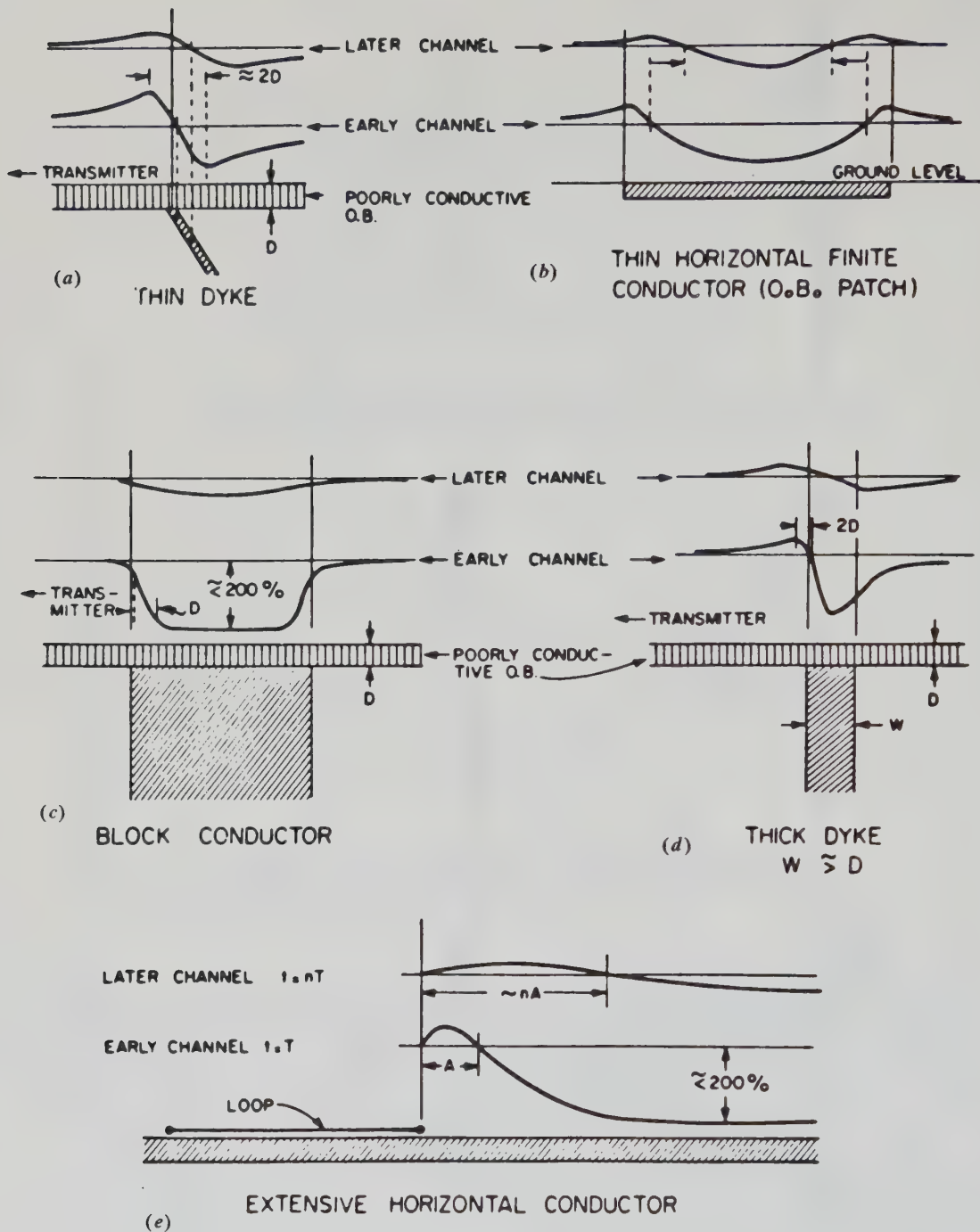
Figure 7.62. The form of continuously normalized UTEM H_z^s profiles over some simple shapes. All conductors are in free space. (After West, Macnae, and Lamontagne, 1984.)
