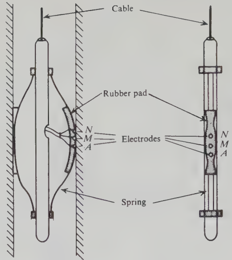
Figure 11.5. Microlog wall-resistivity arrangement.
