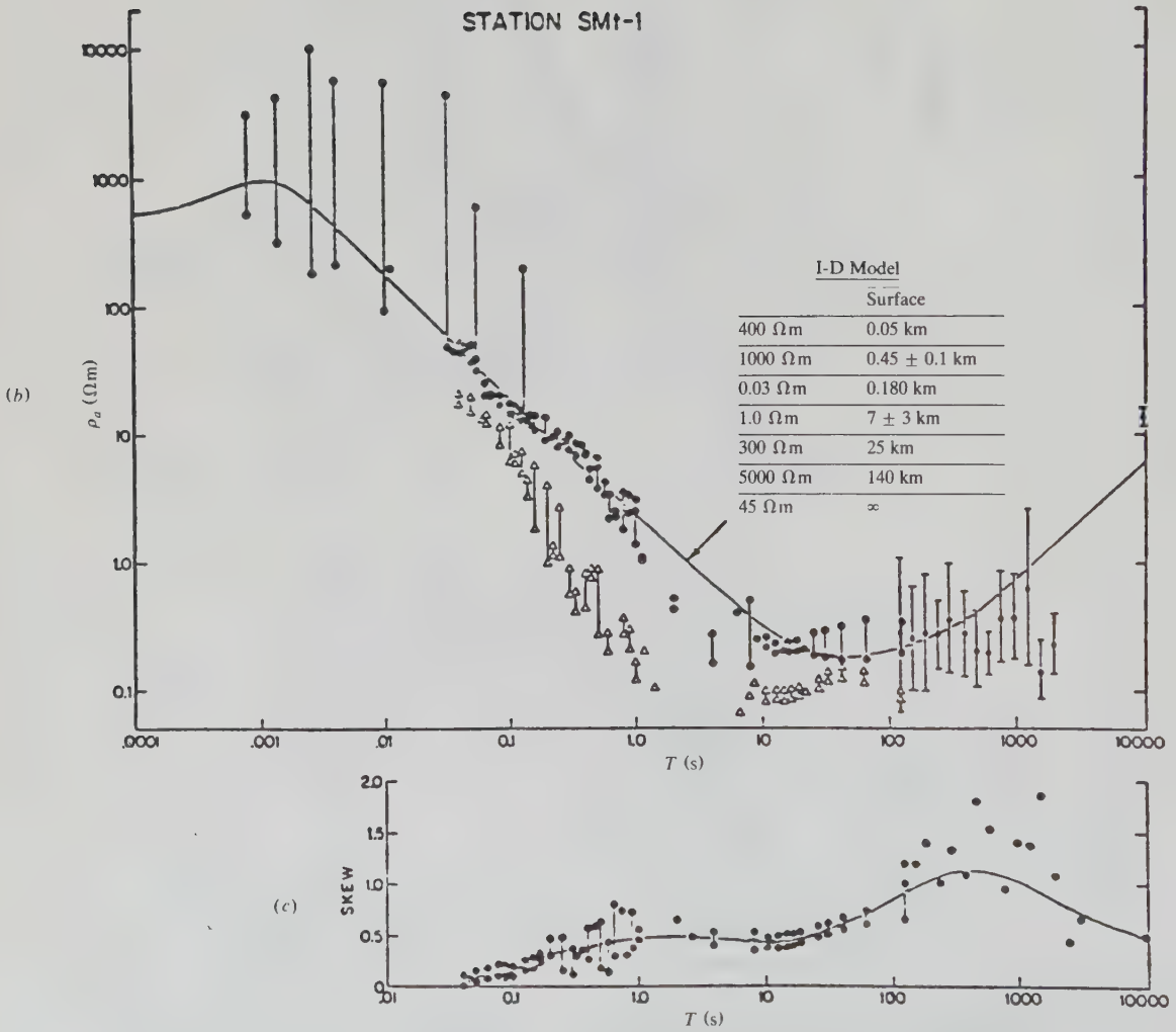
Figure 6.30. \rho_a results near Ste. Mathilde, Quebec. (a) Map showing elevations, locations of profiles 1–3 plus \rho_a contours. (b) Results for station SMT-1: \rho_a curve, tensor data in the principal axis of anisotropy from 0.03 to 10,000 s, and scalar data from 0.0008 to 0.13 s; dots and triangles are \rho_a values for the major and minor axes of anisotropy, respectively; error bars show maximum scatter from 0.0008 to 100 s, two standard deviations from 100 to 10,000 s; solid curve is for the 1-D model. (c) Skew ratios.
