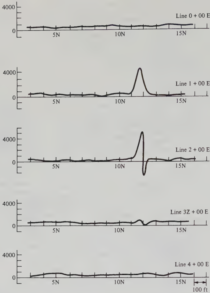
Figure 3.38. Vertical-component magnetic profiles, Rouyn-Noranda district, Quebec.
