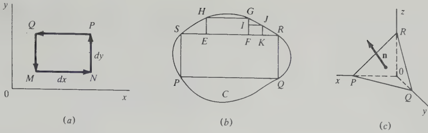
Figure A.3. Derivation of Stokes's theorem. (a) Evaluating a line integral around a rectangle. (b) Evaluating a line integral around an arbitrary closed planar curve C . (c) Resolving a surface integral over a plane triangle into components.
