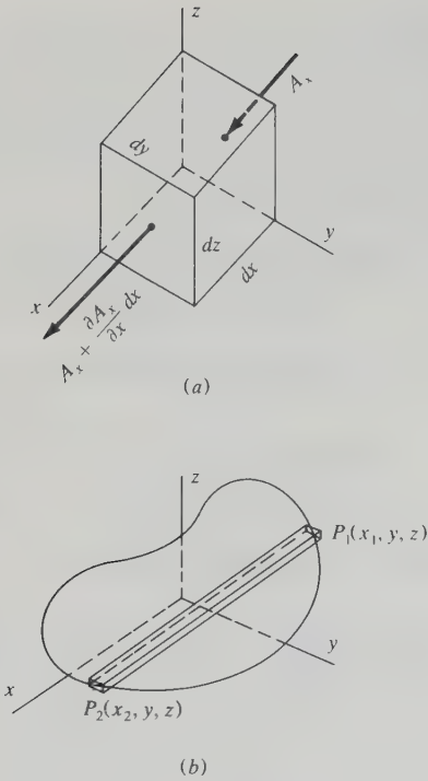
Figure A.2. Vector theorems. (a) Significance of \text{div } \mathbf{A} . (b) Derivation of Gauss's theorem.
