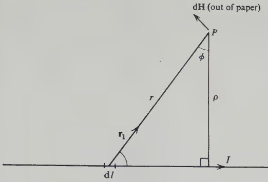
Figure 7.1. Illustrating the Biot-Savart law.
