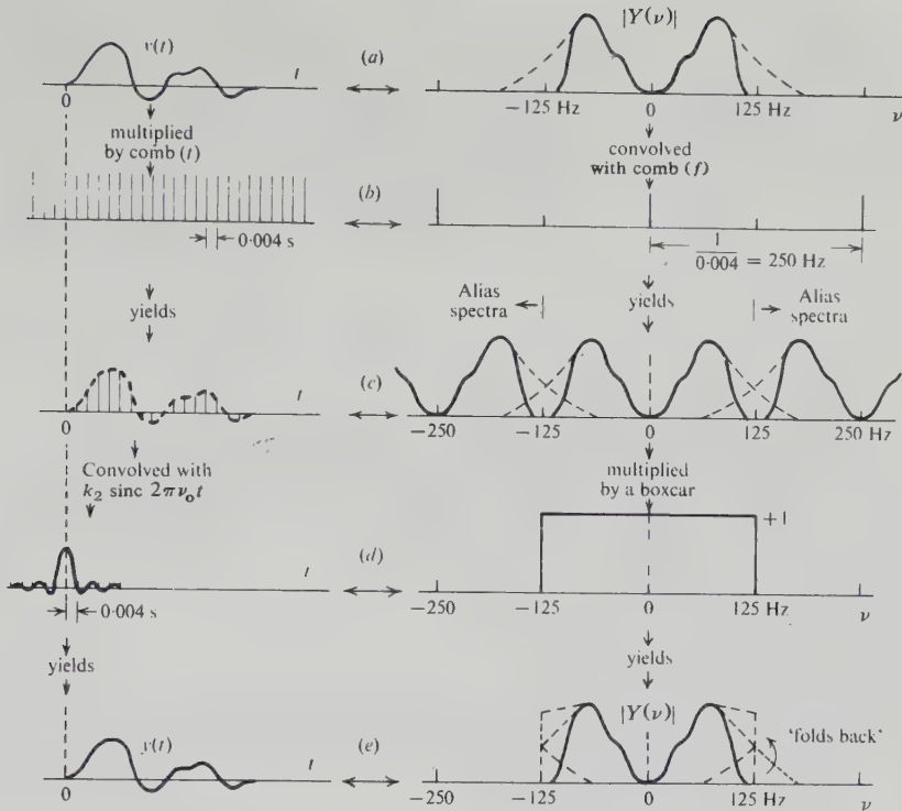
Figure 4.78. Sampling and reconstituting.
