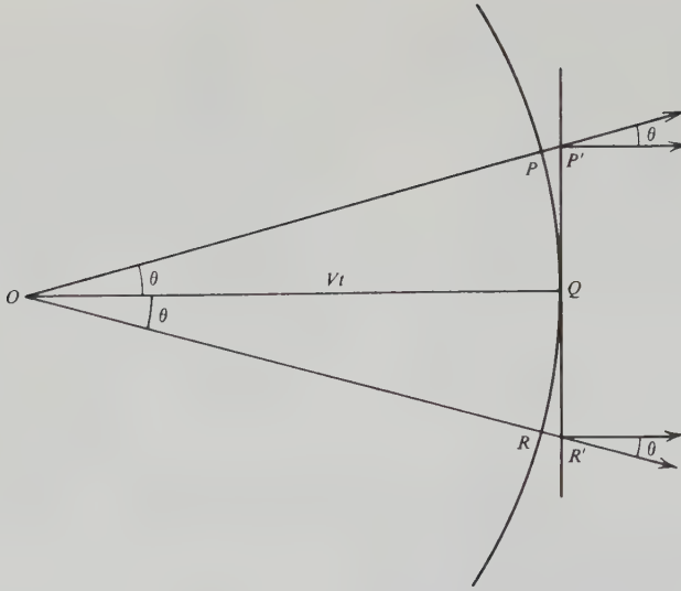
Figure 4.6. Relation between spherical and plane waves.
