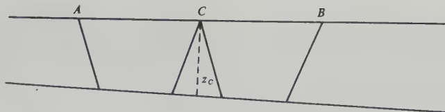
Figure 4.95. Refraction profile for determining depth to bedrock.
