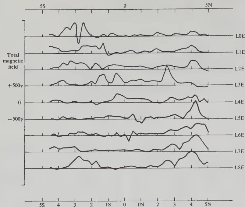
Figure 12.2. Total-field ground-magnetic profiles, Uchi Lake, northwestern Ontario.
