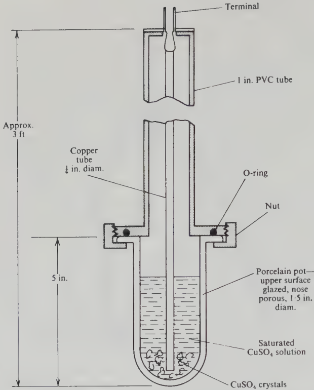
Figure 6.3. Walking-stick SP electrode.
