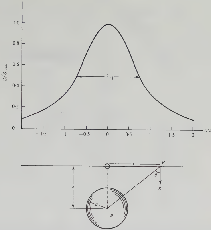
Figure 2.23. Gravity effect of a sphere.
