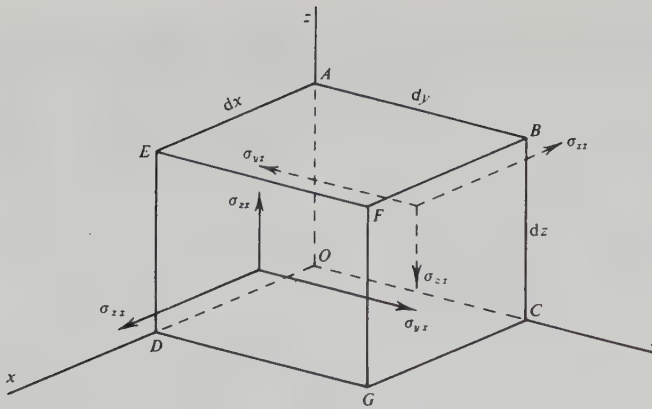
Figure 4.2. Components of stress.
