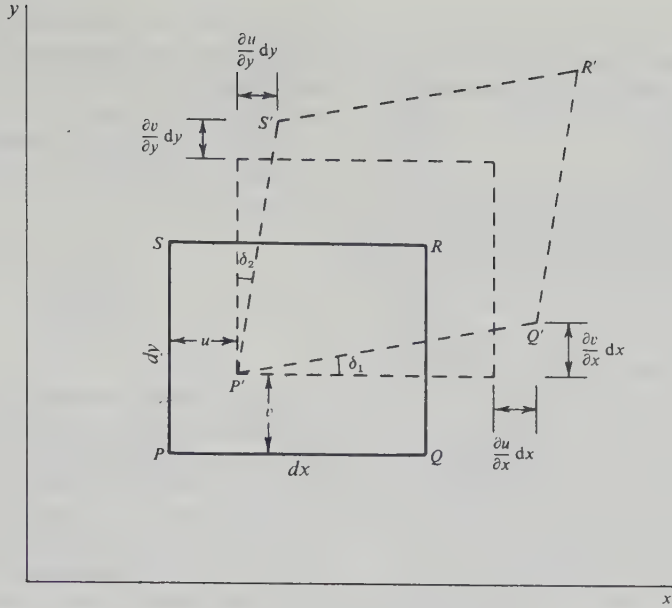
Figure 4.3. Analysis of two-dimensional strain.
