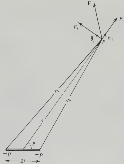
Figure 3.3. Calculating the field of a magnetic dipole.
