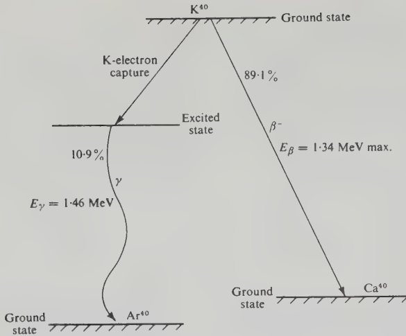
Figure 10.2. Energy-level diagram for radioactive potassium.
