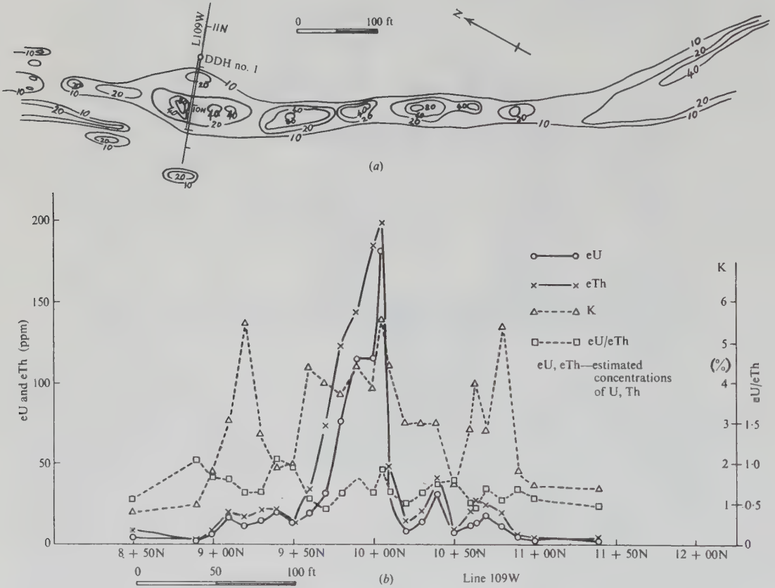
Figure 10.19. Results of radiometric survey over pegmatite, Portneuf, Quebec. (a) Isorad contours; contour interval 1,000 counts/min. (b) Radiometric profiles of eU, eTh, K, and eU/eTh ratio for line 109W.
