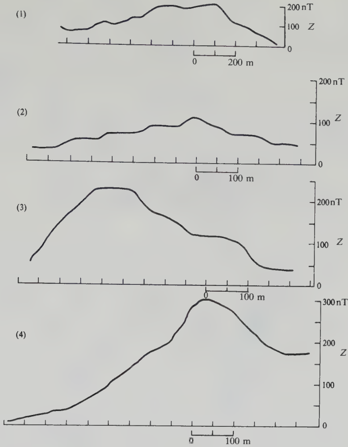
Figure 3.39. Vertical-component magnetic profiles, Manitoba Nickel Belt.
