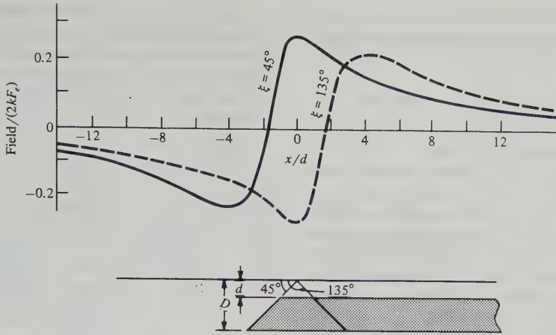
Figure 3.24. F profiles for a semiinfinite horizontal slab striking N-S, I = 45^\circ , dip of slab terminus 45 and 135^\circ , D = 3d .
