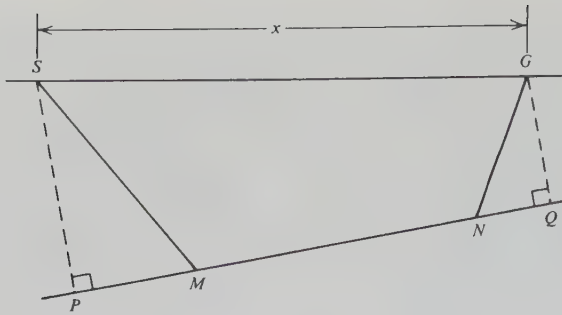
Figure 4.87. Illustrating delay time.
