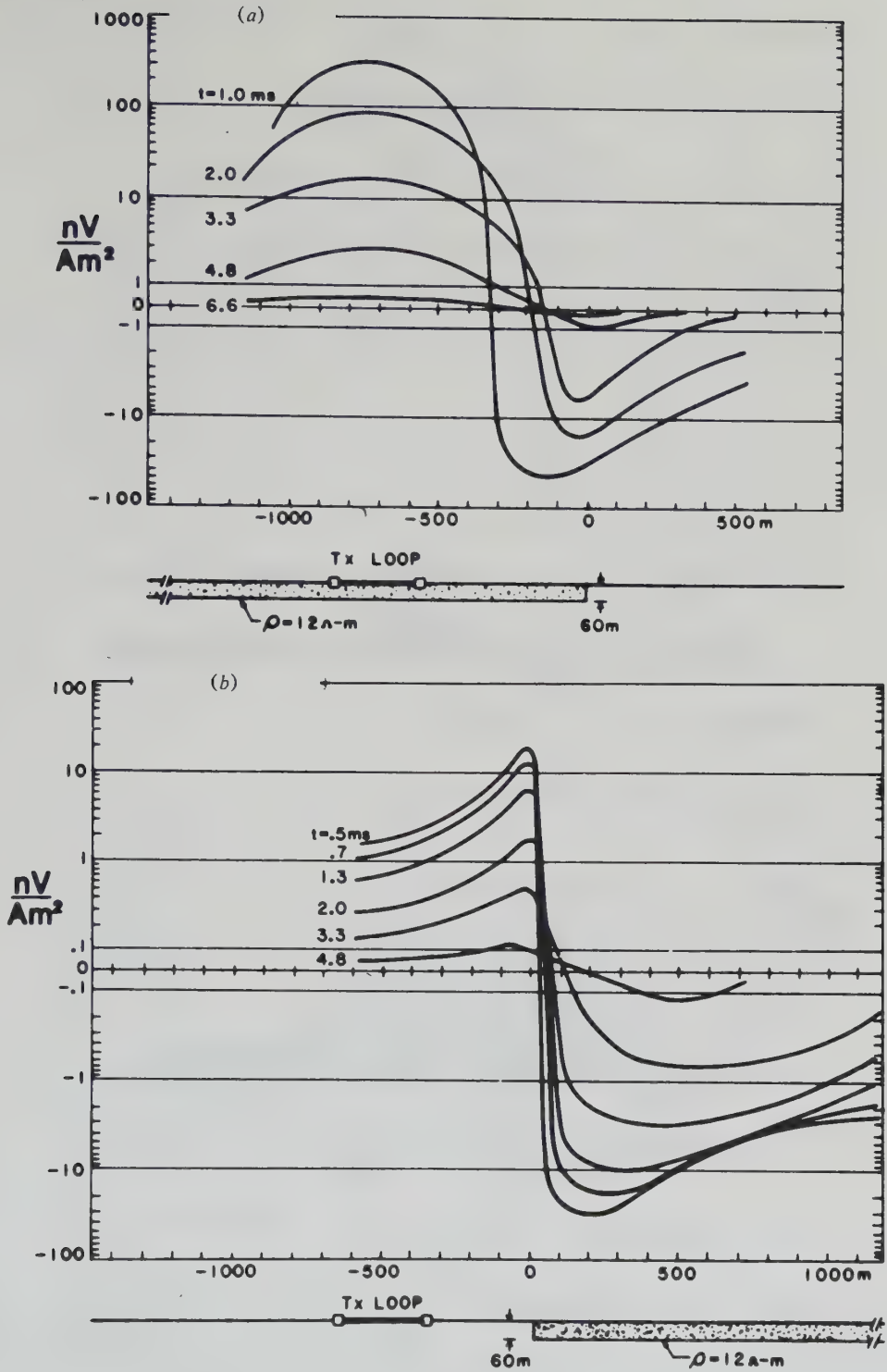
Figure 7.54. Comparison of responses of Turam-type (TDEM) and SIROTEM(1) over conductive overburden. Turam: Tx loop 600 \times 300 m in (a), (b), and (c). (After Spies and Parker, 1984.) (a) Tx on overburden \sim 550 m from edge. (b) Tx offset \sim 350 m from edge.
