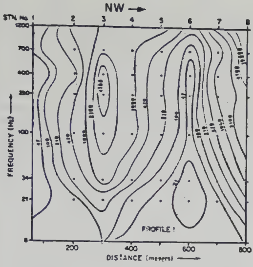
Profile 1 pseudo-section.
