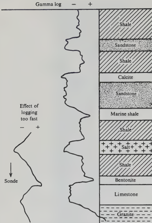
Figure 11.32. A \gamma -ray log.
