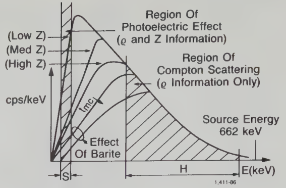
Figure 11.37. Gamma-ray energy spectrum showing the two windows in which measurements are made. The counts in the high-energy window H depend on density only, whereas those in the low-energy windows depend on both density and atomic number Z of the capturing atom. (From Snyder and Fleming, 1985.)
