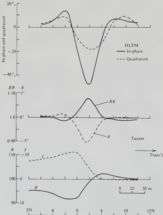
Figure 7.115. HLEM and Turam profiles, northern Quebec.
