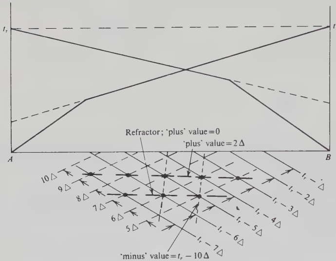
Figure 4.94. The plus–minus method. (After Hagedoorn, 1959.)
