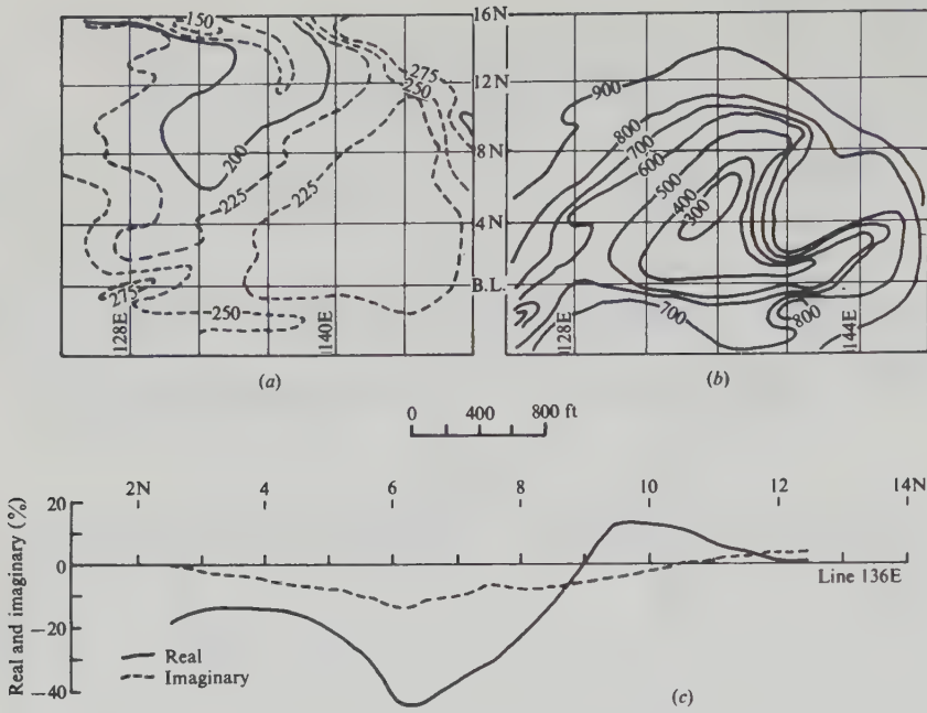
Figure 12.6. Magnetic and electrical data, Murray sulfide deposit, New Brunswick. (a) Magnetic contours; contour interval 25\gamma . (b) SP contours; contour interval 100 mV. (c) HLEM profile; frequency 440 Hz, T-R spacing 300 ft.
