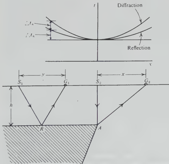
Figure 4.37. Diffraction traveltime curve.
