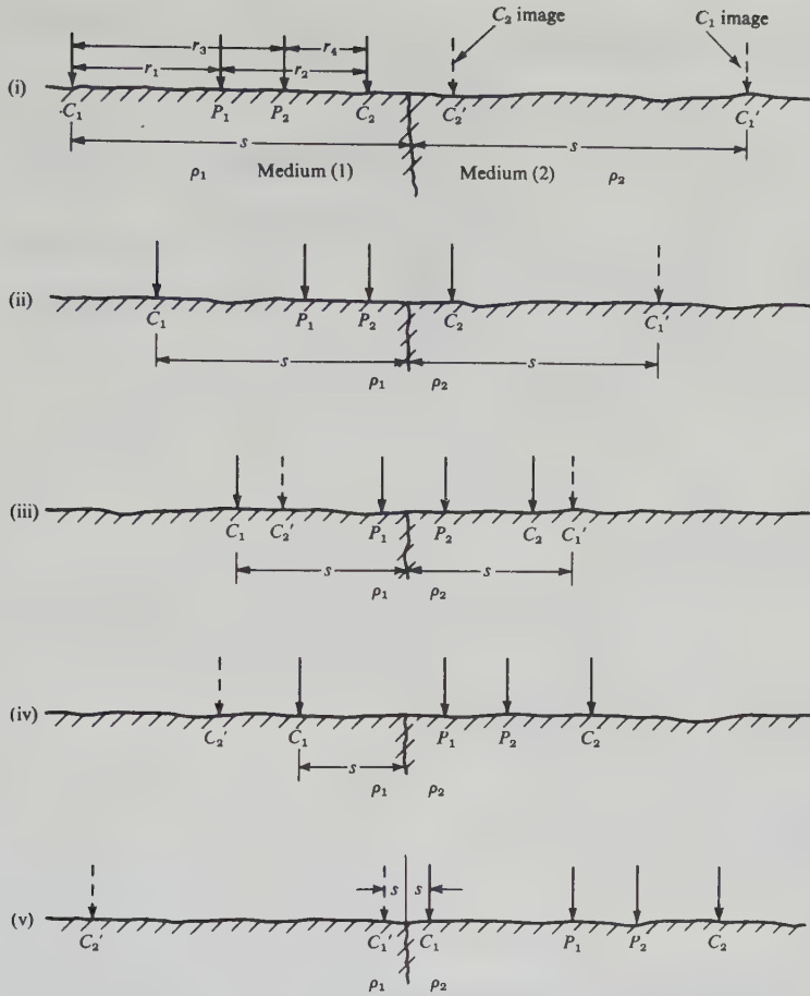
Figure 8.33. General resistivity spread over a vertical contact.
