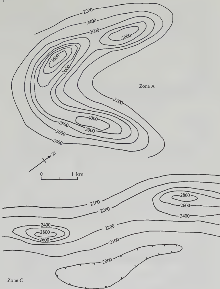
Figure 3.37. Ground magnetic contours, northern Manitoba. C.I. = 100 \text{ nT} .
