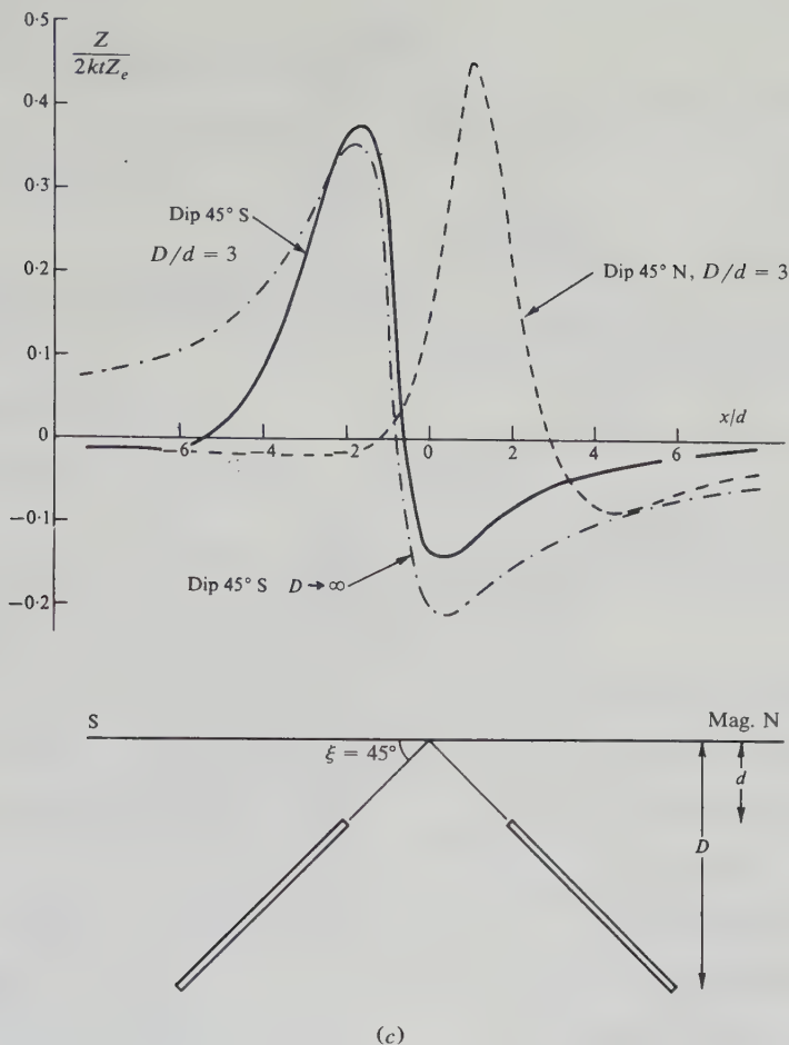
Figure 3.20. (Continued) (c) Z profiles for E-W strike, \xi = 45^\circ N and 45^\circ S , \beta = 90^\circ .
