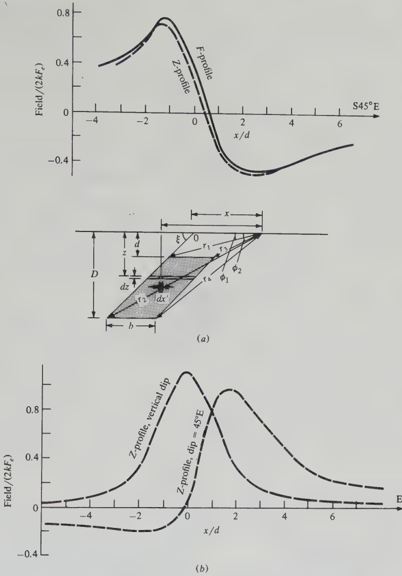
Figure 3.18. Profiles for dike model. L = \infty except for (d). (a) F, Z profiles for I = 60^\circ , \beta = 45^\circ , \xi = 45^\circ , b = 2d , D = 3.5d . (b) Z profiles for I = 75^\circ , \beta = 0^\circ , \xi = 45^\circ E and 90^\circ , b = 2d , D = \infty .
