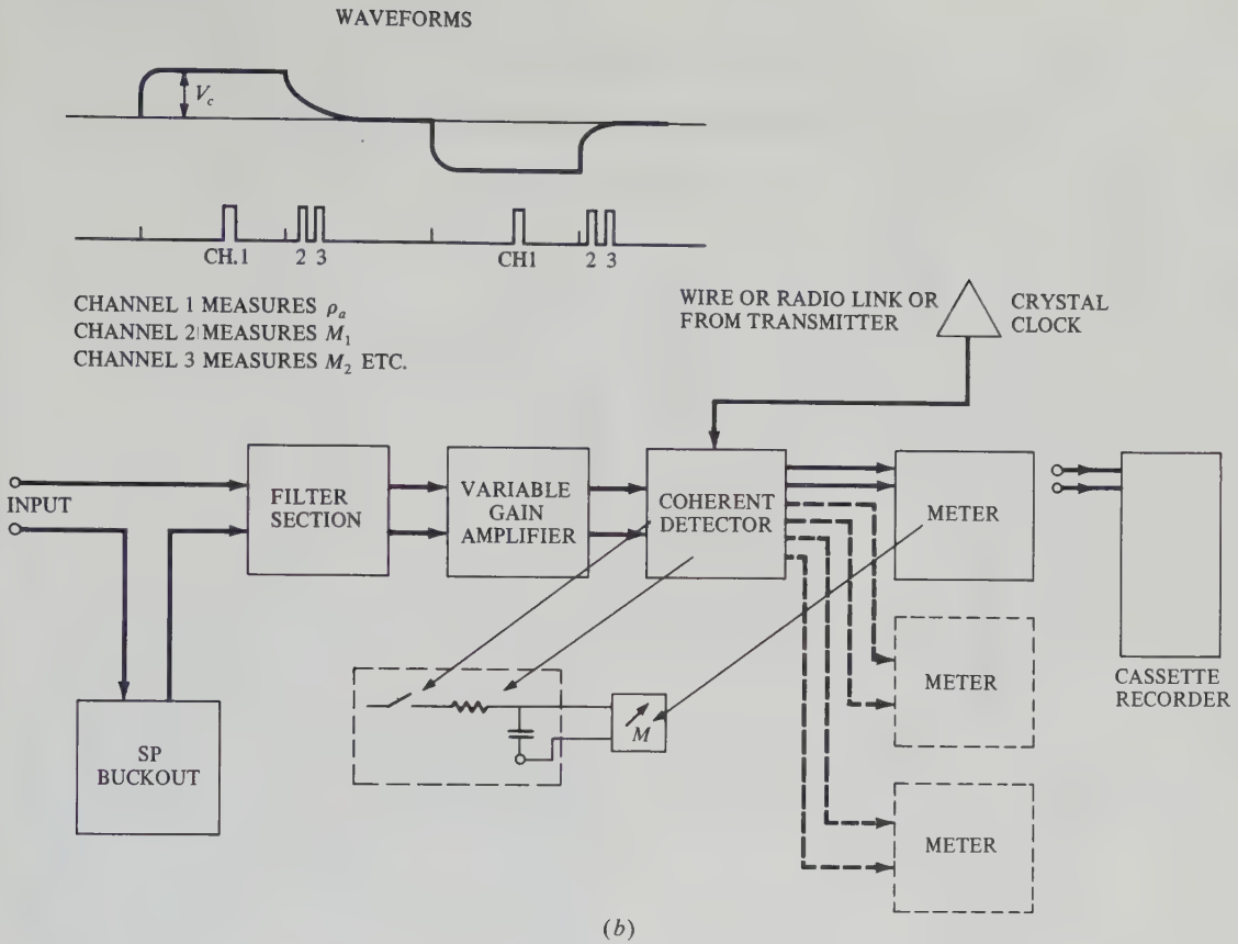
Figure 9.6. (Continued) (b) F-D receiver. (After Sumner, 1976.)
