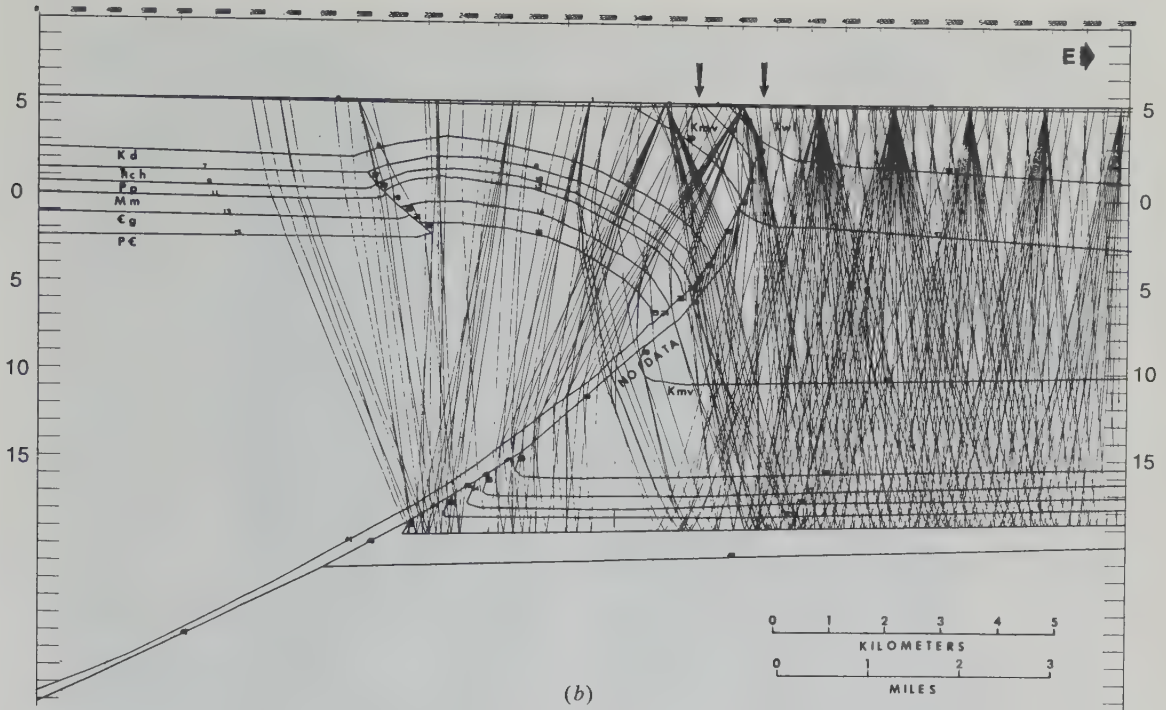
Figure 4.98. (Continued) (b) Ray tracing through a depth model (depths in kft 10^3 ).
