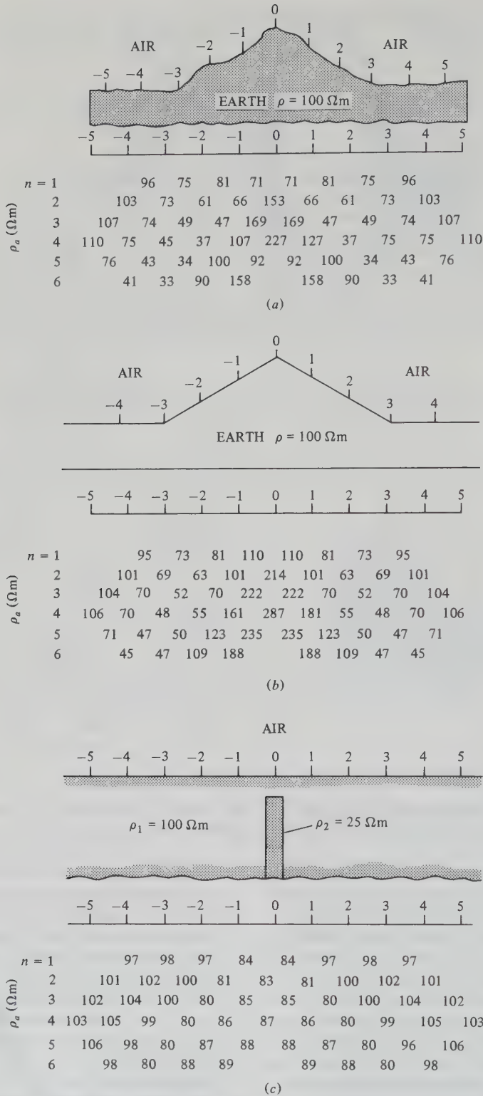
Figure 8.52. Effect of terrain on dipole-dipole resistivity survey. (a) Pseudodepth plot of \rho_a over 2-D ridge. (b) Model results for a 30^\circ ridge. (c) Results over a buried vertical conductive dike.
