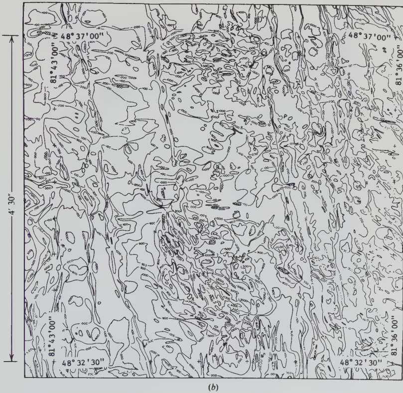
Figure 3.31. High-resolution aeromagnetic survey, Timmins area, Ontario. (From Bhattacharyya, 1971.) (a) Geological map. (b) Ground vertical-intensity map.
