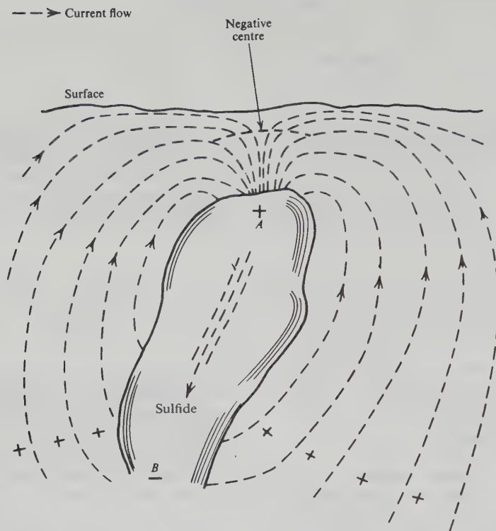
Figure 6.1. Oxidizing sulfide zone as a galvanic cell.
