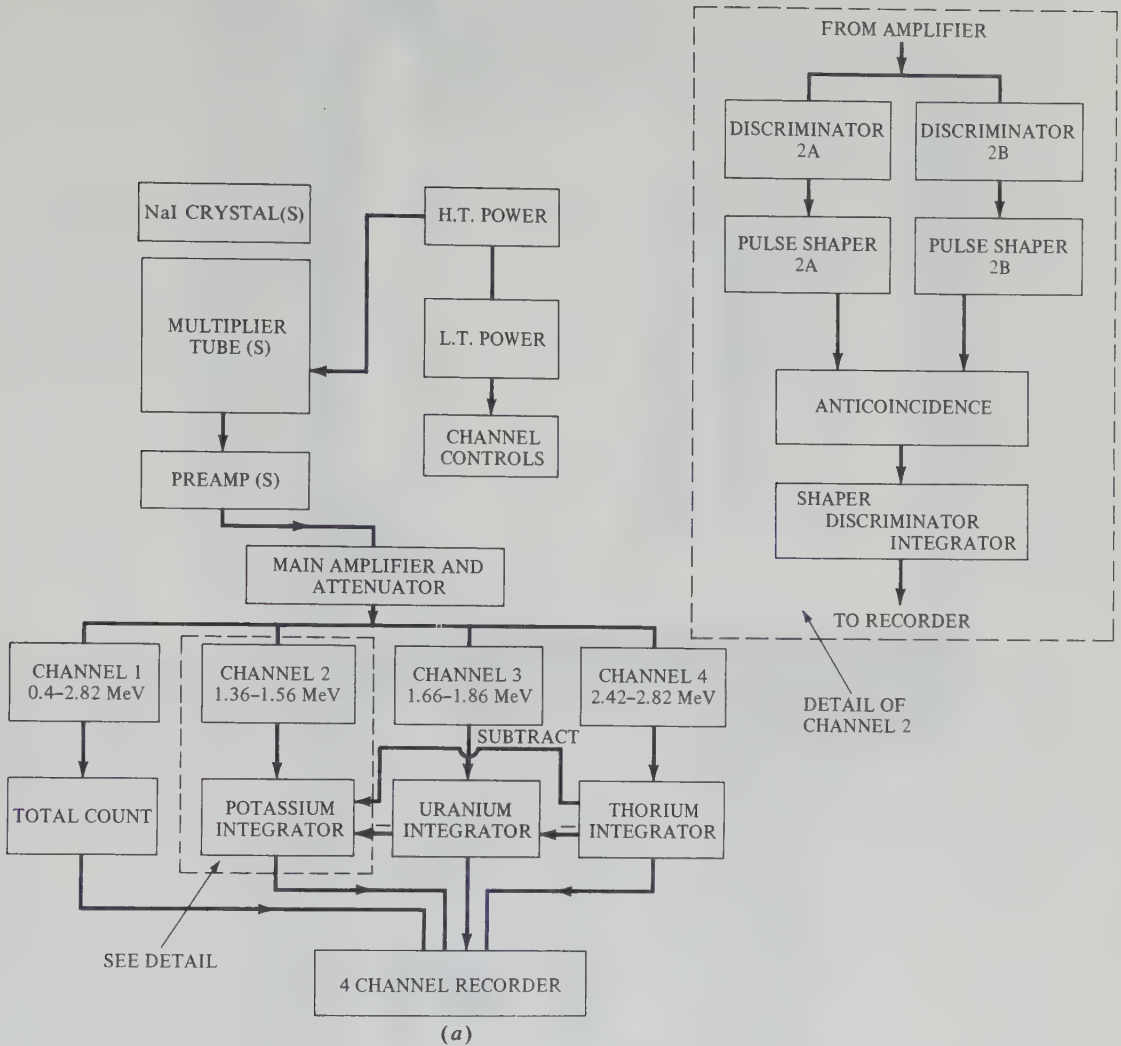
Figure 10.8. Four-channel \gamma -ray spectrometer. (a) Block diagram.
