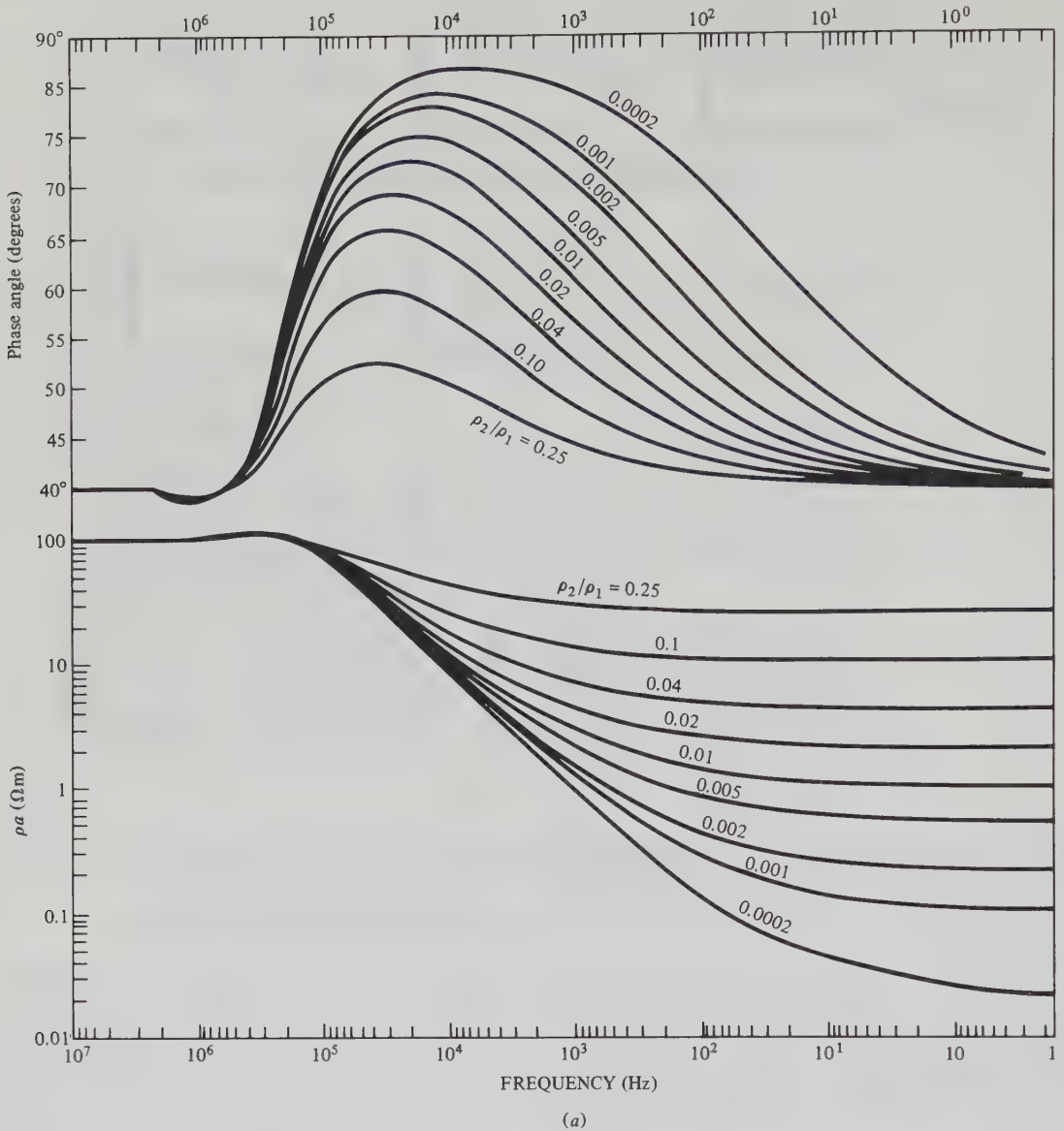
Figure 6.22. Master curves for MT sounding over two-layer earth. \rho_1 = 100 \text{ } \Omega\text{m} and z_1 = 10 \text{ m} . (a) \rho_2 < \rho_1 .
