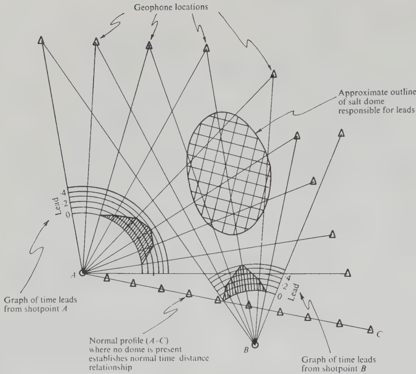
Figure 4.72. Fan shooting. (After Nettleton, 1940.)
