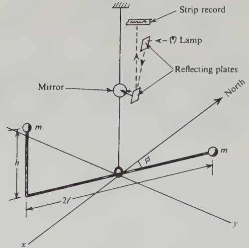
Figure 2.9. Torsion balance (schematic).
