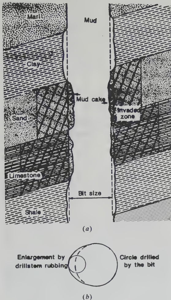
Figure 11.1. Borehole shape. (a) Conceptual vertical slice through a borehole showing caving and mud buildup on permeable formations. (From Tittman, 1986.) (b) Egg-shaped cross section of borehole showing most probable location of a sonde equipped with an "eccentering" arm.
