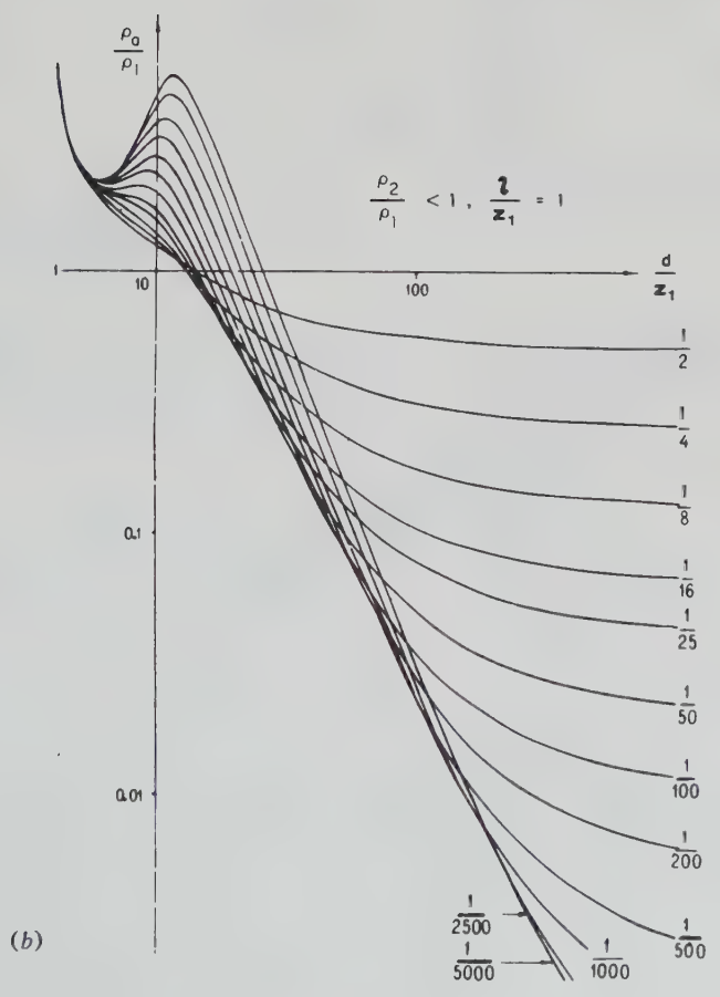
Figure 7.76. Master curves of late-time (\rho_a/\rho_1) versus (d/z_1) . [Parts (a) and (b): After McNeill, 1980; parts (c) to (f): After Kaufmann and Keller, 1983.] (a) Two-layer curves for resistive basement. (b) Same as (a) except for conductive basement.
