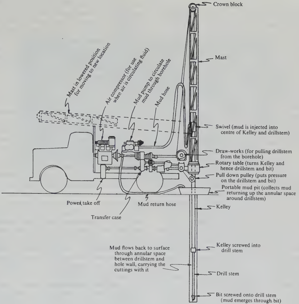
Figure 4.51. Rotary drill. (From Sheriff, 1984.)
