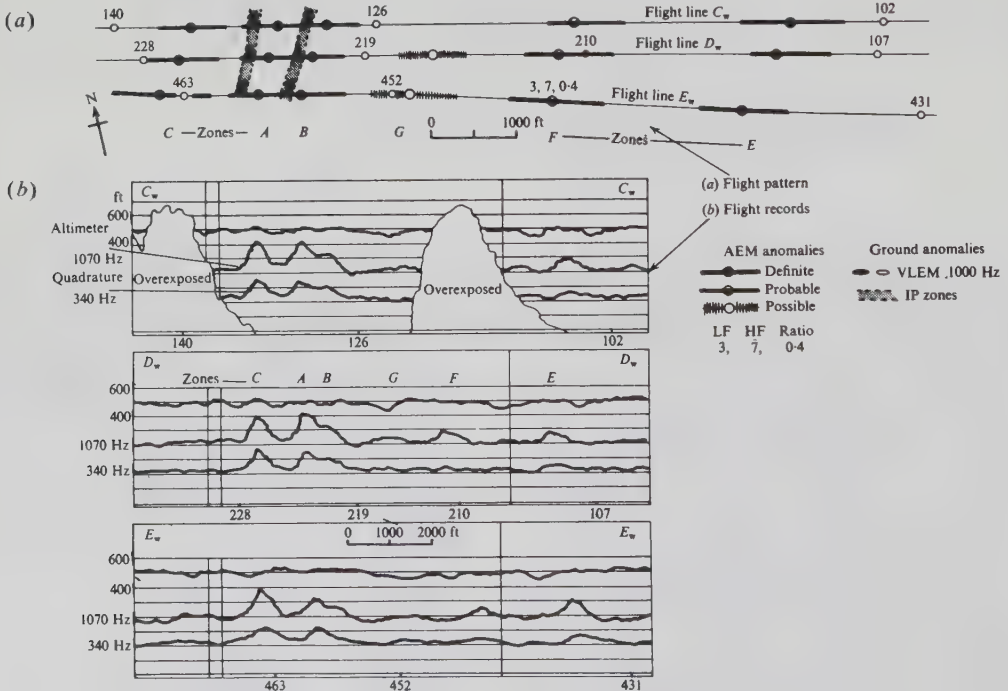
Figure 7.119. Quadrature airborne EM survey, Cavendish geophysical test site, Ontario. (a) Flight pattern. (b) Flight records.
