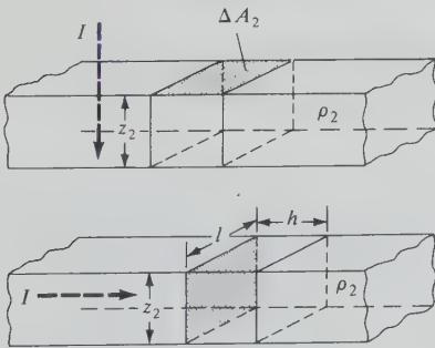
Figure 8.30. Effect of topography on expanding Wenner spread.
