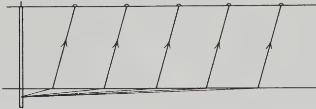
Figure 4.76. Refraction weathering profile.
