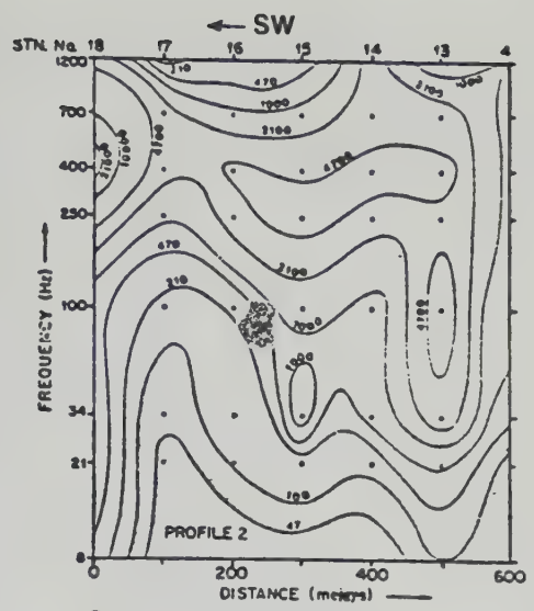
Profile 2 pseudo-section.
