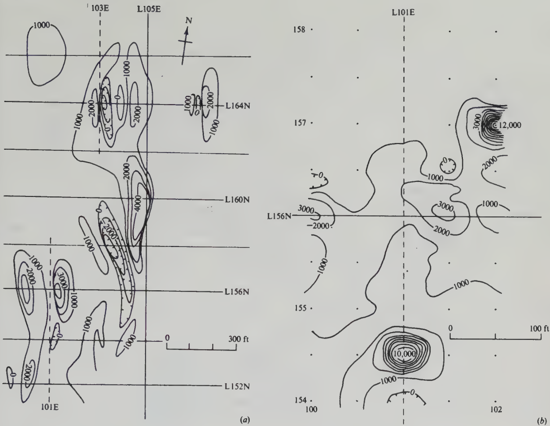
Figure 3.36. Effect of line spacing on magnetic data. (a) Conventional magnetic map, C.I. = 1,000 nT. (b) Detailed magnetic map centered at 156N, 101E.
