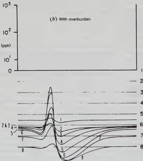
Figure 7.52. Approximate effect of conductive overburden. \ell = d = 600 m, z = 50 m, T-R = 100 m, \sigma = 30 S, dip = 30^\circ . Channel numbers are at the right in (a) and (b), channel response at the left. (After Bartel and Hohmann, 1985). (a) Response without overburden. (b) Response with overburden. (c) Overburden model.
