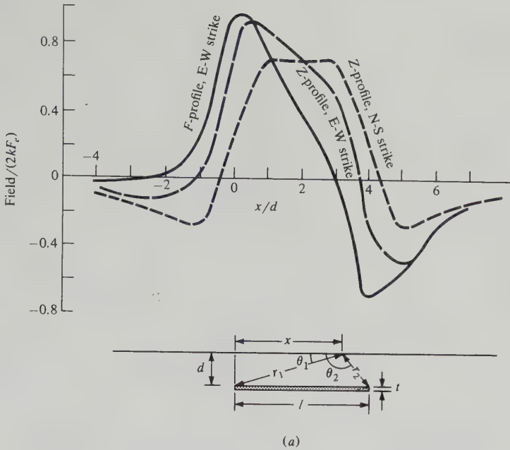
Figure 3.21. Thin horizontal plate of finite width, t/l = 0.125 . (a) Profiles for l = 60^\circ , \beta = 0^\circ and 90^\circ , d/l = 0.25 .
