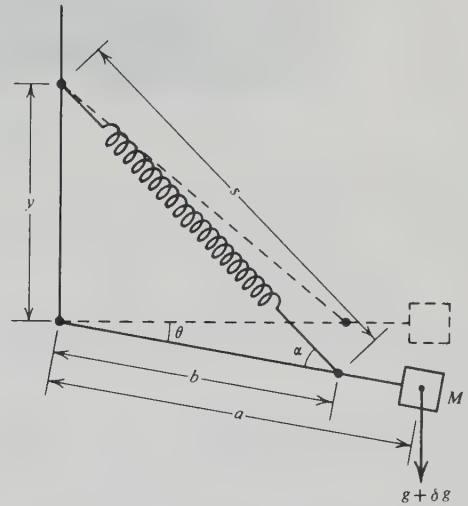
Figure 2.12. Lacoste–Romberg gravimeter.
