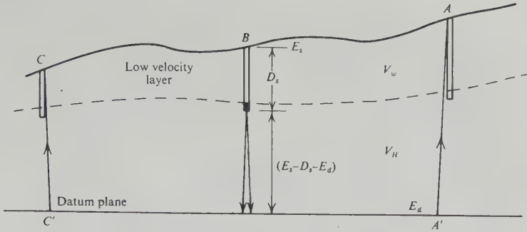
Figure 4.74. Calculation of weathering corrections.
