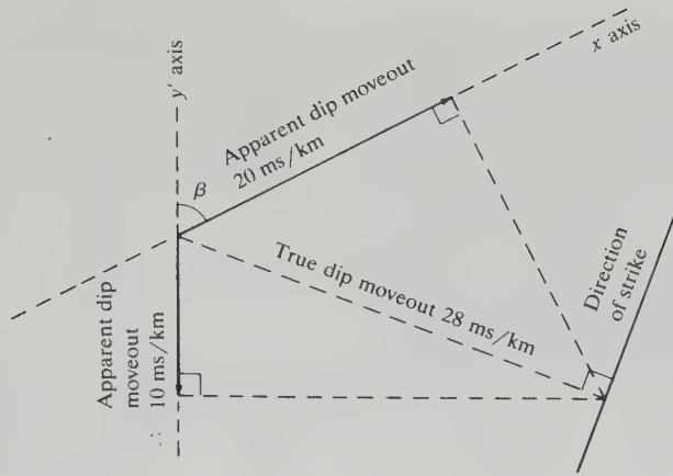
Figure 4.27. Resolution of cross-spread information.
