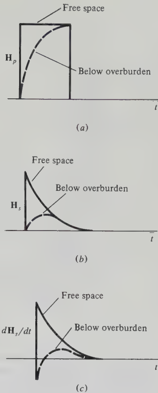
Figure 7.51. Effect of overburden (ob) on TDEM fields. (a) Primary field at target. (b) Secondary field at target. (c) Receiver response from target.
