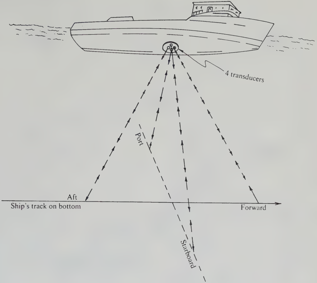
Figure B.3. Doppler-sonar navigation. (From Sheriff, 1984.)
