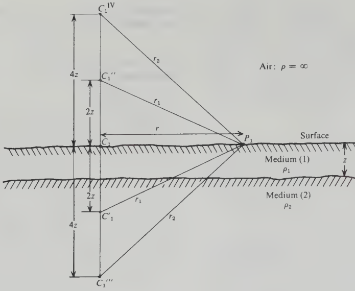
Figure 8.11. Images resulting from two horizontal beds.
