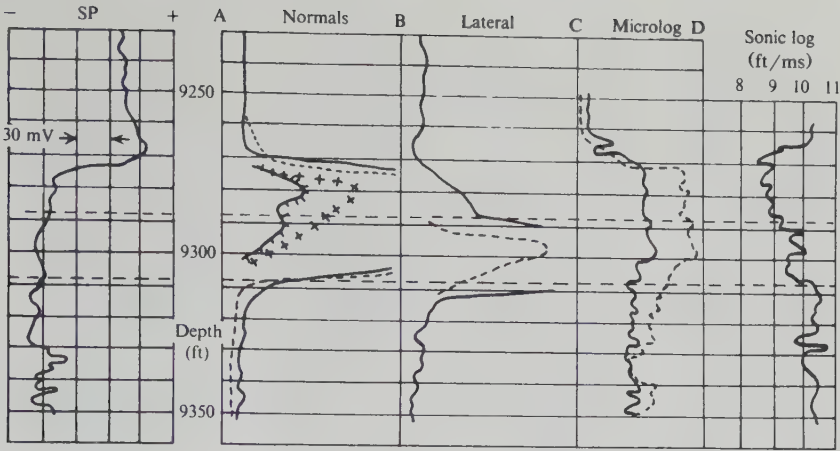
Figure 11.44. Log suite in Miocene sand section containing oil and gas. Full scale for the 16 in. normal (solid curve) is 10 \Omega m , for the amplified 16 in. normal (solid hatched) is 100 \Omega m , for the 64 in. normal (dashed) is 10 \Omega m , for the amplified 64 in. normal (crosses) is 1,000 \Omega m , for the 18 ft 8 in. lateral (solid) is 10 \Omega m , for the amplified 18 ft 8 in. lateral (dashed) is 100 \Omega m , and for the microlog inverse (solid) and for the micronormal (dashed) is 10 \Omega m .
