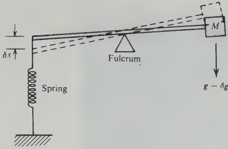
Figure 2.10. Basic principle of the stable gravimeter.
