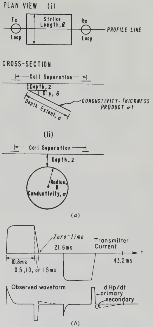
Figure 7.49. PEM(1) moving-source TDEM. (After Bartel and Hohmann, 1985.) (a) Geometry of thin-plate and sphere models. (b) Waveform for 10.8 ms pulse.
