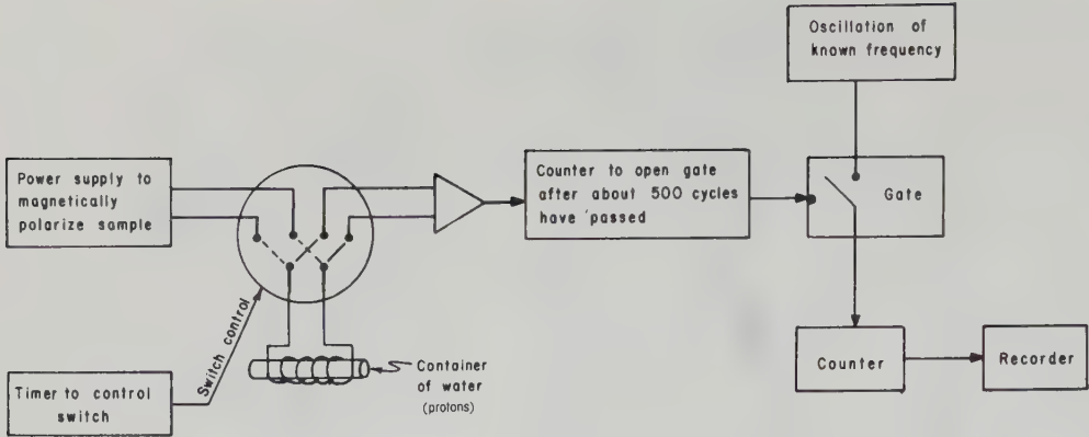
Figure 3.10. Proton-precession magnetometer. (From Sheriff, 1984.)
