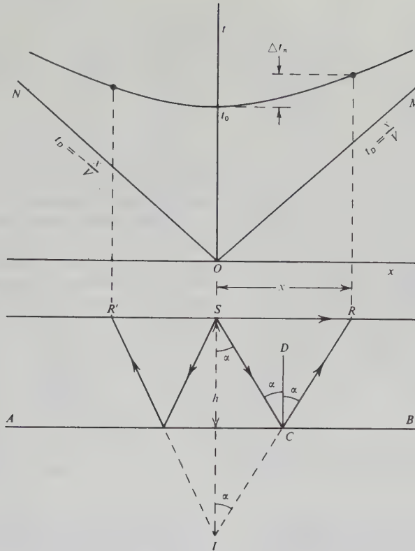
Figure 4.22. Geometry and traveltime curve for horizontal reflector.
