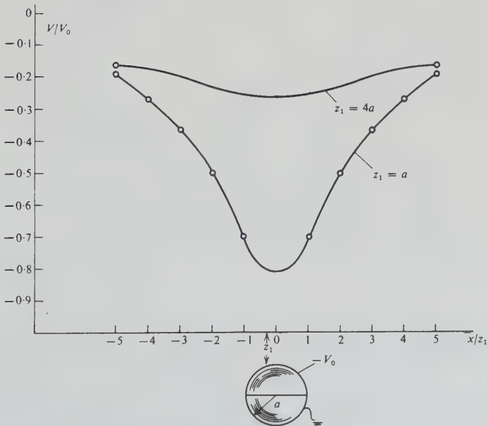
Figure 6.6. SP profiles over buried polarized sphere.
