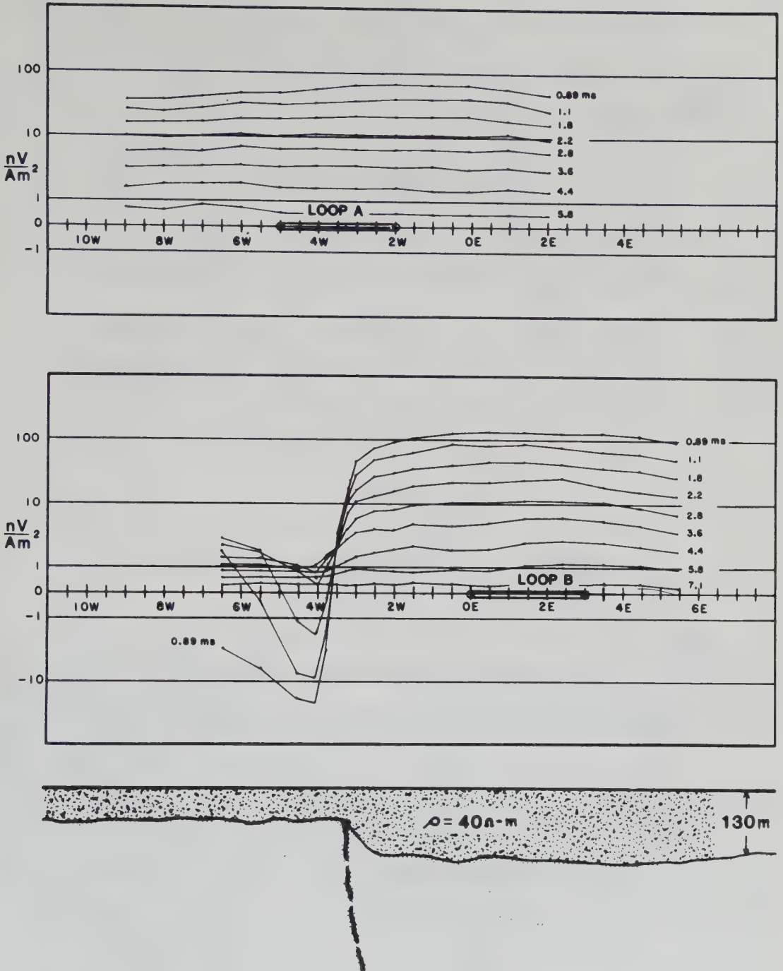
Figure 7.58. Field traverses obtained with a fixed-loop system for two different transmitter-loop positions. The strong anomaly recorded with loop B disappeared when loop A was used. (After Spies and Parker, 1984.)
