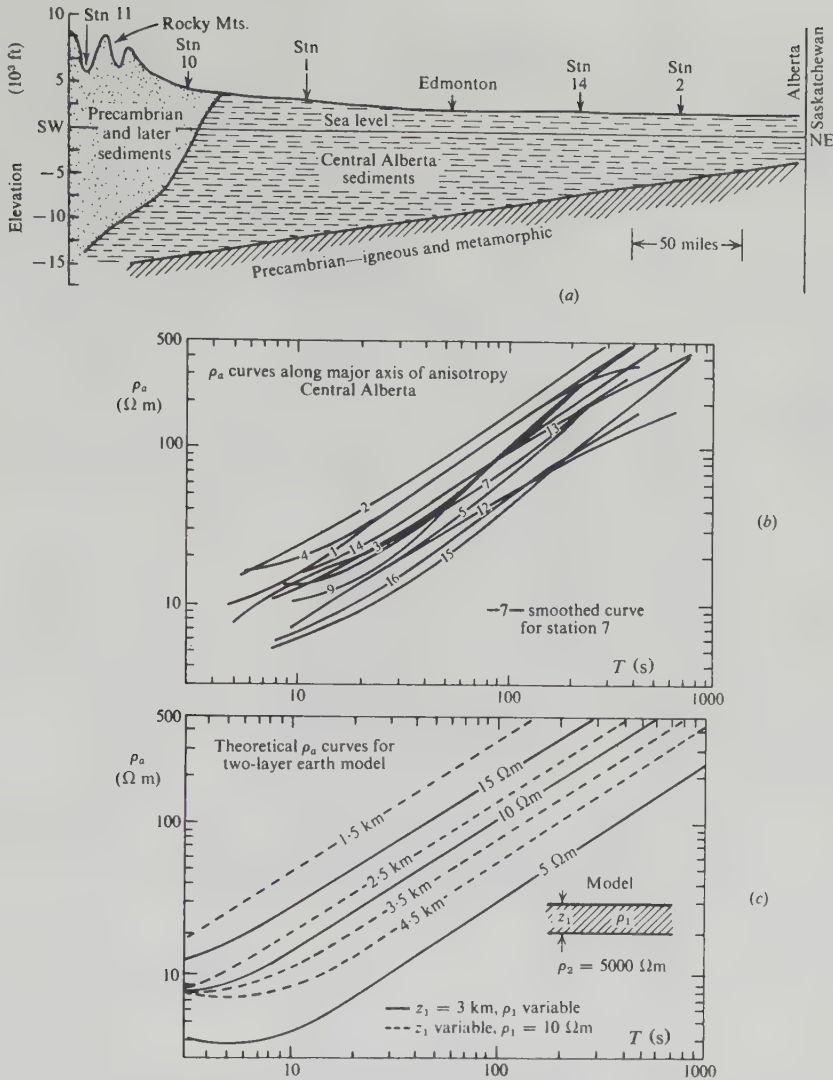
Figure 6.27. Magnetotelluric deep soundings in Central Alberta. (After Reddy and Rankin, 1971.) (a) Geological section. (b) \rho_a curves along major axis of anisotropy. (c) Theoretical \rho_a curves for two-layer earth.
