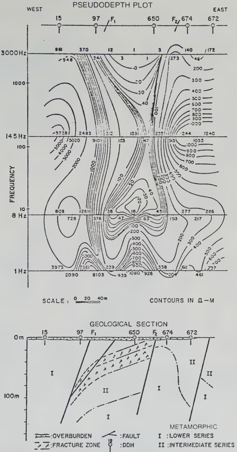
Figure 6.29. Magnetotelluric pseudodepth plot for conductive fracture zone, Northern Saskatchewan.
