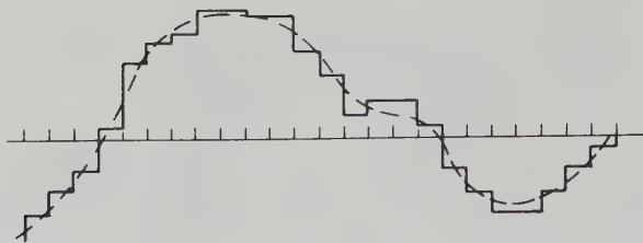
Figure 4.59. Conversion from digital to analog form.
