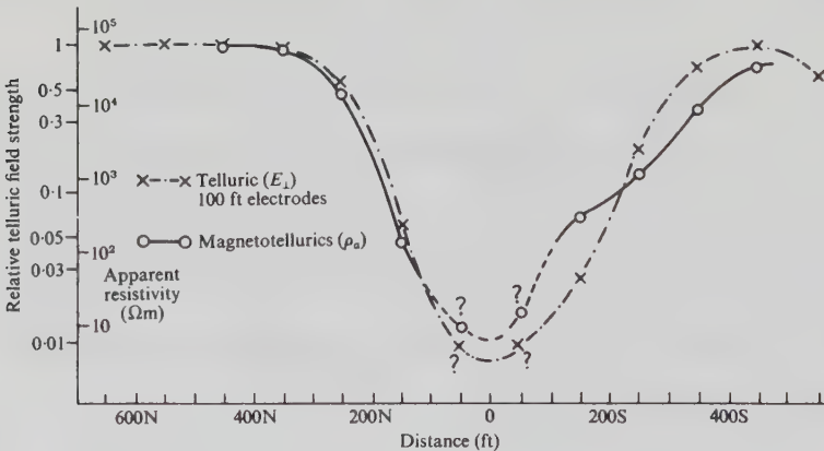
Figure 6.37. 8 Hz magnetotelluric profile, Northern Quebec.
