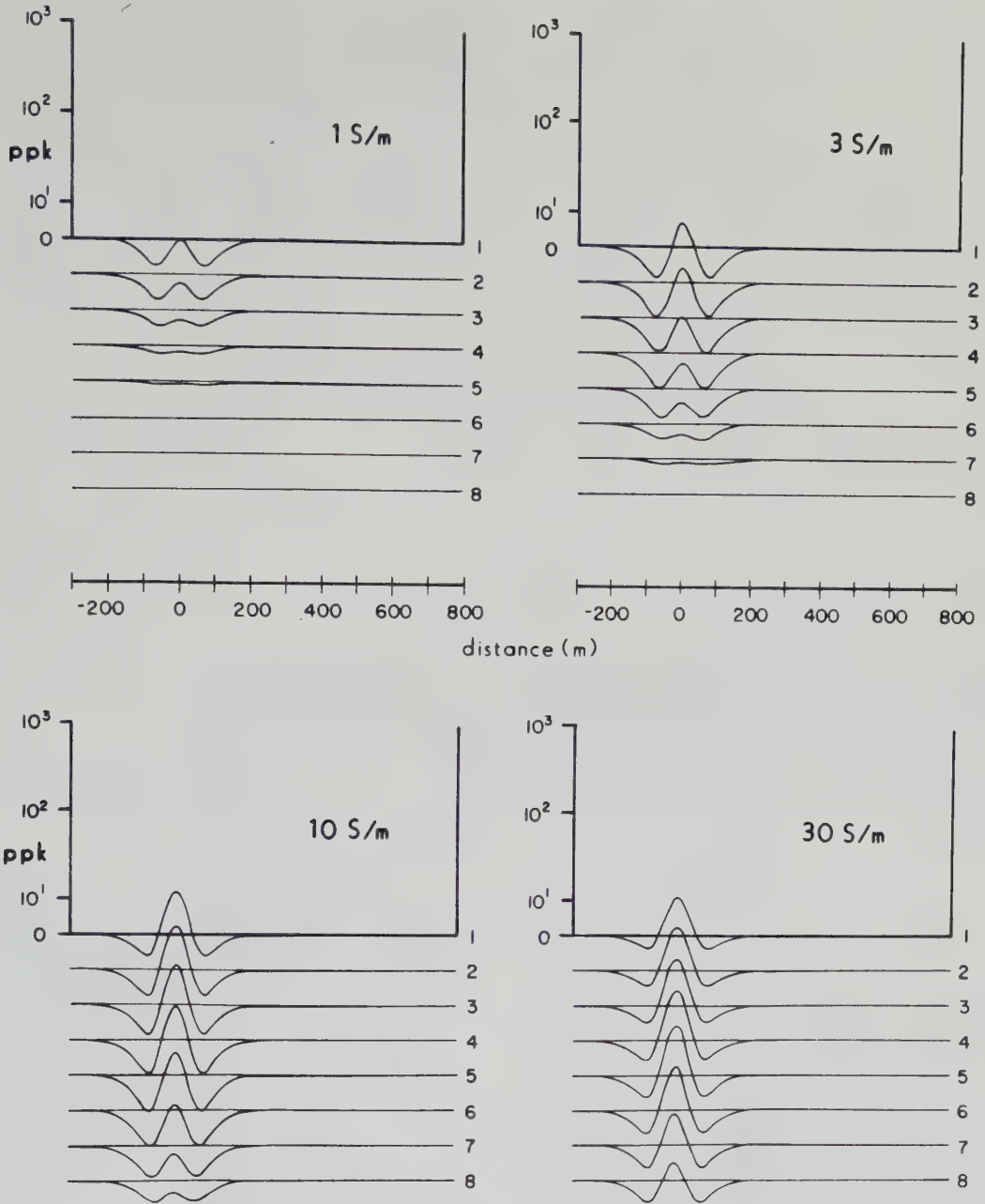
Figure 7.70. Response of PEM(1) system to a buried sphere as a function of conductivity. Radius of sphere = 50 m = depth to top, l = 100 m. (After Bartel and Hohmann, 1985.)
