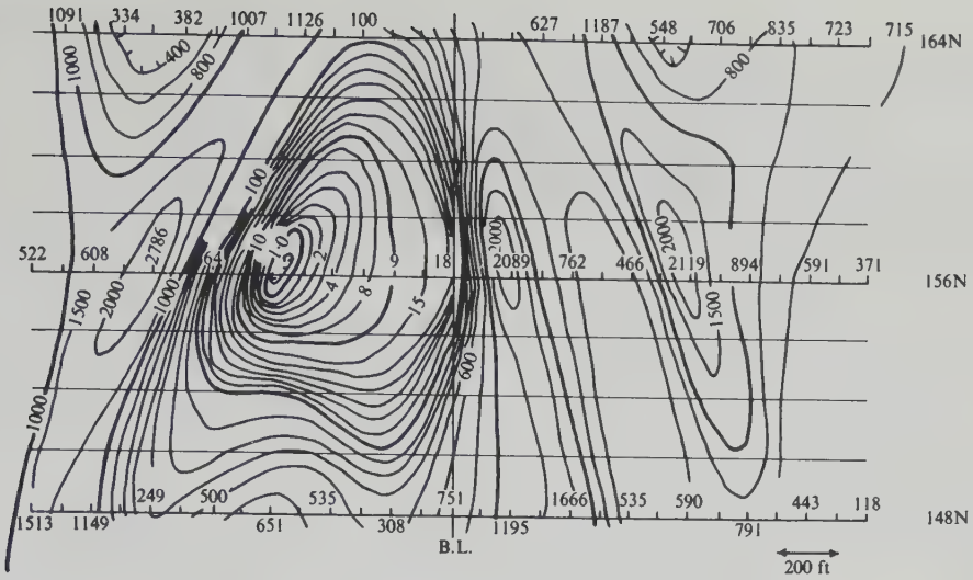
Figure 8.50. Apparent-resistivity contours ( \Omega m ), southern New Brunswick.
