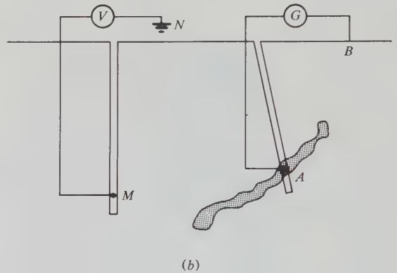
Figure 11.9. Resistivity log configurations for orebody definition. (After Roy, 1984.) (a) Directional resistivity method; the azimuthal direction of AB is changed 90^\circ between measurements. (b) Mise-à-la-masse method with the A electrode embedded in conductive orebody and potential measured in nearby boreholes.
