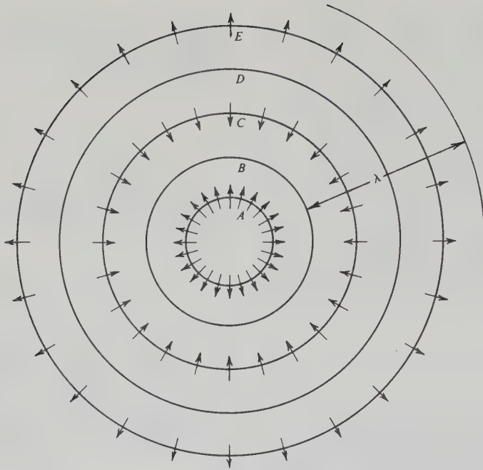
Figure 4.7. Displacements for a spherical P wave.
