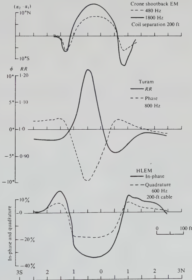
Figure 7.116. Shootback, Turam, and HLEM profiles, western Ontario.
