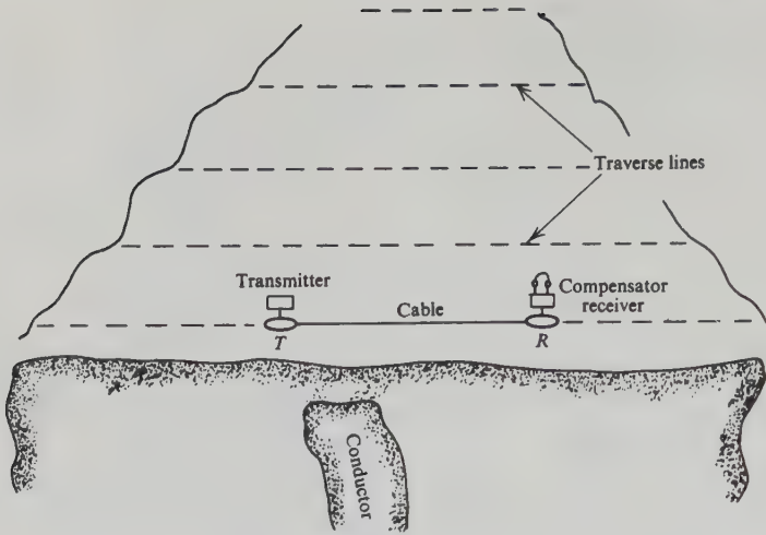
Figure 7.20. Horizontal-loop system.
