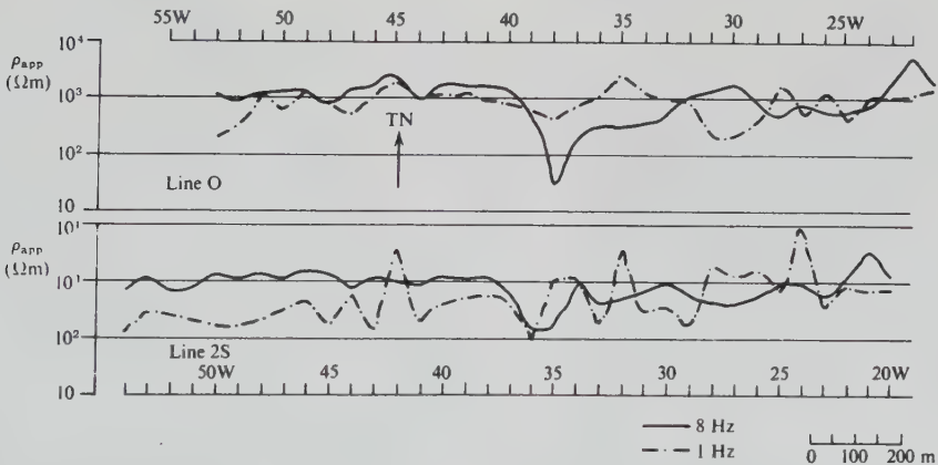
Figure 6.35. Telluric profiles at 1 and 8 Hz, Northeastern Brazil.
