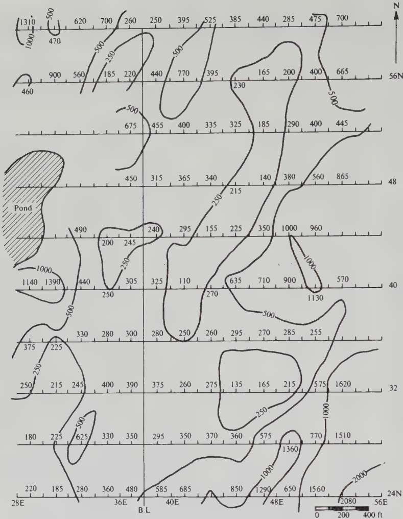
Figure 8.49. Apparent-resistivity contours ( \Omega ft ) for a base-metal zone, eastern Nova Scotia.
