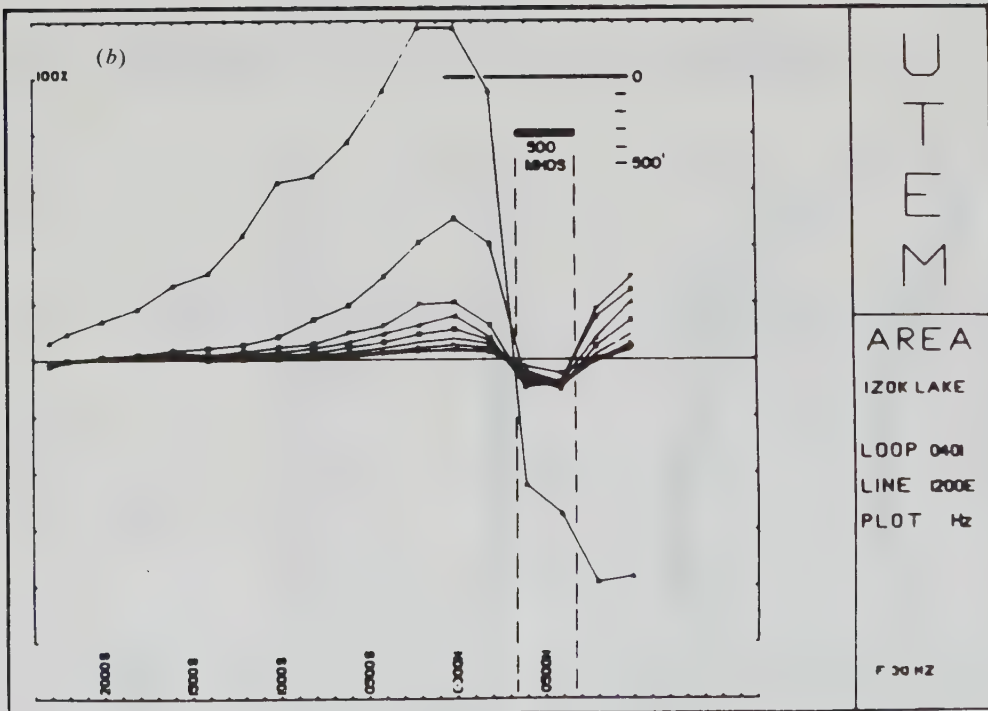
Figure 7.105. UTEM test over Izok Lake deposit, North West Territories, Canada. (After Podolsky and Slankis, 1979.) (a) Map of interpreted mineralization. (b) Profile along line 12E.
