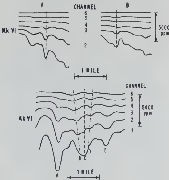
Figure 7.125. Input profiles over four bedrock conductors, Western Australia. Conductors are covered by varying thicknesses of conductive overburden.
