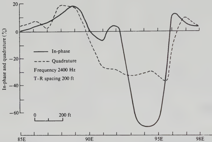
Figure 7.112. HLEM profiles, Eastern Townships, Quebec.
