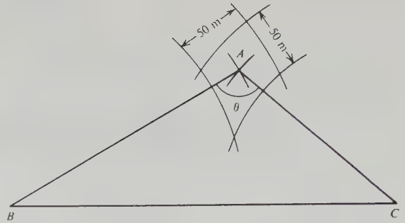
Figure B.1. Locating point A by striking arcs from fixed stations B and C (a rho-rho determination); effect of station angle on errors in position. \theta is the station angle, A is the mobile station, B and C are the shore stations. Point A can be anywhere inside the "parallelogram" formed by the four arcs. [Note: Range errors are not to scale.]
