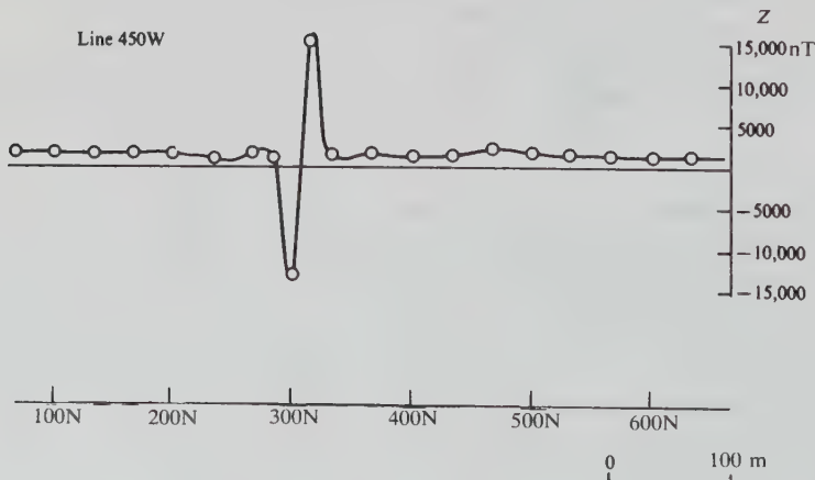
Figure 3.35. Vertical-component ground magnetic profile, East Africa.
