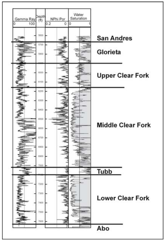
Fig. 7.42. Type log from the South Wasson Clear Fork field
