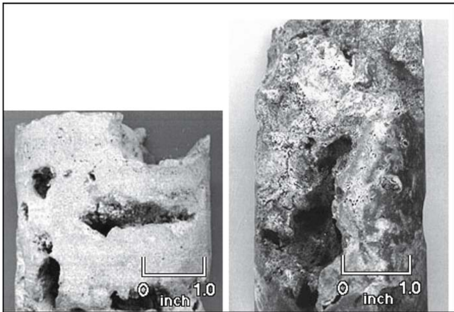
Fig. 8.12. Examples of cavernous porosity observed in cores. A Miami Oolite from the Miami aquifer, Miami, Florida. B Niagaran (Silurian), Michigan pinna-reef
