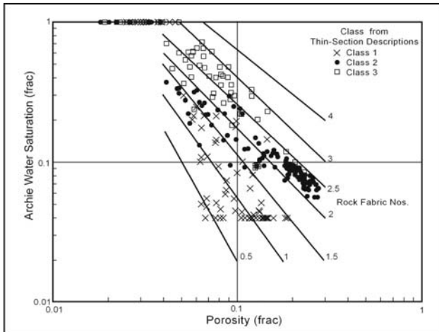
Fig. 7.24. Cross plot of porosity and water saturation for Haradh (Lucia 1995). The class 1 field is dominated by large crystalline dolostone. Grain-dominated packstones form the basis for the class 2 field. Data that overlap into the class 1 field may be responding to large-grain fabrics. Low porosity mud-dominated fabrics define the class 3 field. The class 4 boundary was spaced above the class 3 samples
