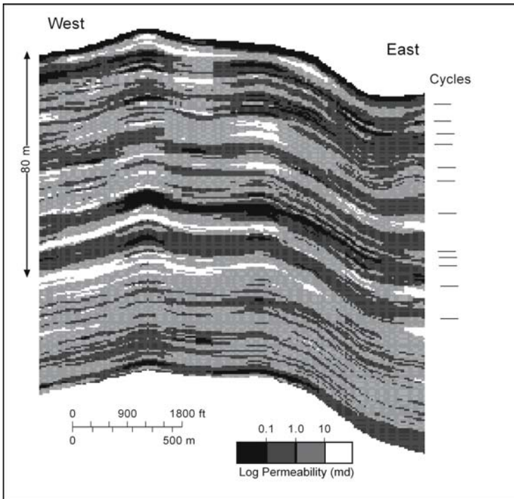
Fig. 7.50. North-to-south Stratamod cross section of the middle Clear Fork reservoir showing permeability distribution
