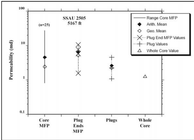
Fig. 5.14. Detailed permeability results from sample 5167 ft, Seminole San Andres Unit well 2505 showing variability factor of 50
