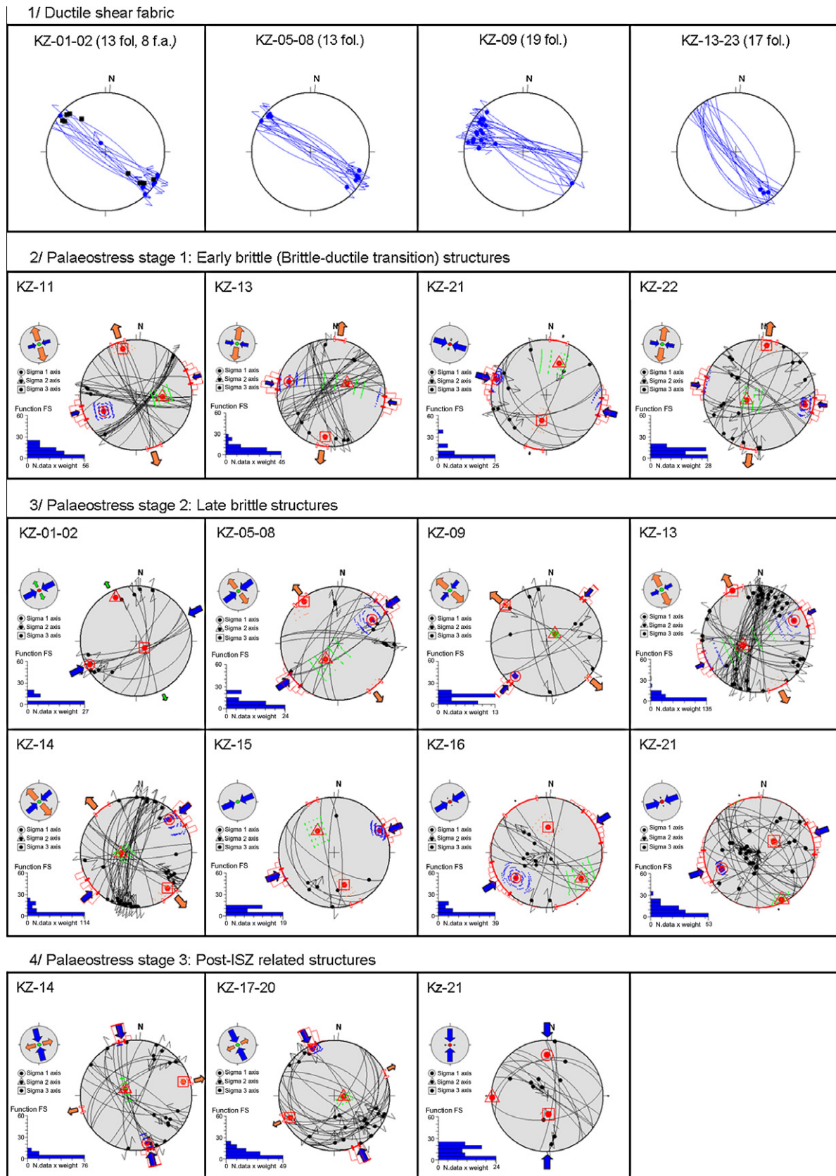
Fig. 7. Fault-slip data and stress inversion. Lower-hemisphere Schmidt stereonet of the fault-slip data subsets and corresponding stress tensor. Stress symbols show the horizontal stress axes ( S_{Hmax} and S_{Hmin} ) in function of the stress ratio R . Their length and colour symbolise the horizontal deviatoric stress magnitude, relative to the isotropic stress \sigma_i . Orange outward arrows: \sigma_3 stress axis, green arrows: \sigma_2 stress axis (outward when extensional \sigma_2 > \sigma_i ) and inward when compressional \sigma_2 < \sigma_i ), blue inward arrows: \sigma_1 axis. The vertical stress \sigma_v is symbolised by a solid circle, orange for extensional regimes \sigma_1 \sim \sigma_v , green for strike-slip regimes \sigma_2 \sim \sigma_v or blue for compressional regimes \sigma_3 \sim \sigma_v . The histogram represents the distribution of the weighted misfit function. The uncertainties related to the stress axis determination are plotted as small dots (blue for \sigma_1 , green for \sigma_2 , orange for \sigma_3 ), and the distribution of possible S_{Hmax} orientations is shown on the outer margin of the net, with 5° frequency interval (bars) and 1 \sigma confidence region (bold red line). fol. = foliations, f.a. = fold axes.
