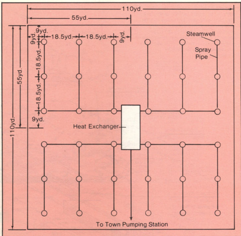
Schematic plan view of one of four square areas (110 yd \times 110 yd) in lava field on Heimaey, where heat is extracted from cooling lavas at depth. Each one-fourth of this square area (55 yd \times 55 yd) can generate 5 megawatts (MW) of hot water at peak load (or 2.5 MW at normal load). (From information provided by Próf. Svienbjörn Björnsson, University of Iceland ).
