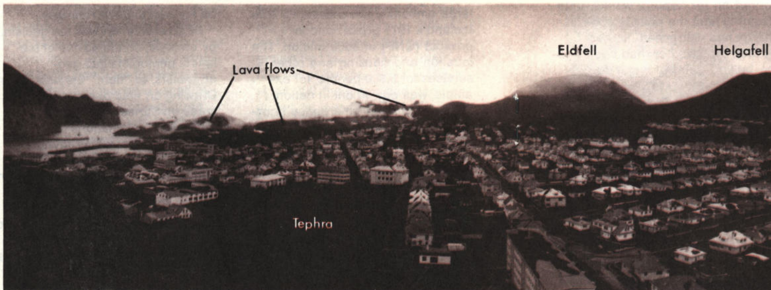
A panoramic view east-southeast across the fishing port of Vestmannaeyjar on May 5, 1973. Dark, tephra-covered ground is apparent, with lava flows into the town and harbor in the left background.
