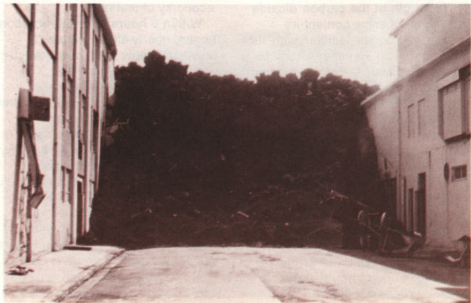
View on July 23, 1973, southeast from dock area in the northern part of Vestmannaeyjar toward edge of lava flow where it stopped against and between two fish-factory buildings. Two boys can be seen in the right background sweeping up the tephra. By July 1974 the lava had been completely removed and restoration of the factories had begun.
