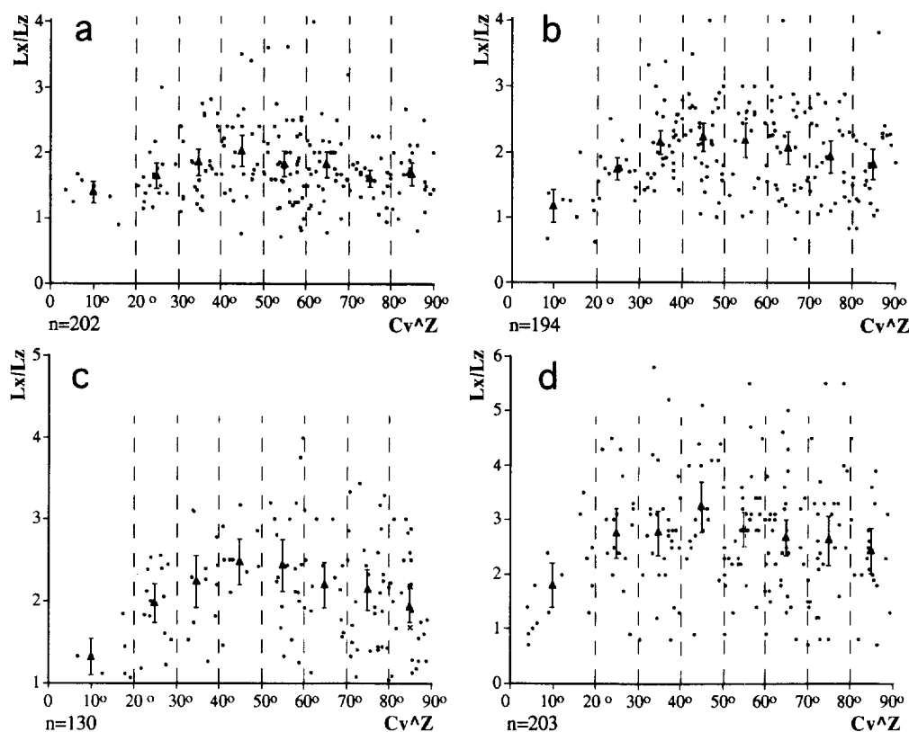
Fig. 7. Plot of aspect ratios ( L_x/L_z ) of detrital quartz grains versus the C_v \wedge Z angle. The mean aspect ratios through intervals of 10^\circ of C_v \wedge Z (dashed vertical bars) are shown as triangles (the first interval unites data of 0-20^\circ of C_v \wedge Z , as the amount of grains having small C_v \wedge Z angles was too small). Vertical bars show 95% confidence intervals for calculated means.
