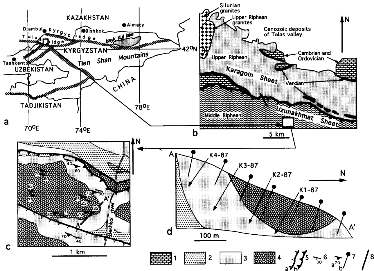
Fig. 1. Geological sketches and location maps of the study area. (a) Regional geographic setting. (b) Simplified geological map showing locations of the main regional tectonic elements. (c) Geological map of the study area showing location of the section. (d) Geological cross-section and location of specimens examined (shown by arrows). Legend for the geological map (c) and cross-section (d): 1, Karabura Formation—intercalations of marble and carbonaceous sandstone; 2–4, Uzunakhmat Formation, 2, Member 1—phyllites with interbeds of sandstone; 3, Member 2—intercalation (2–10 m) of sandstone and phyllitic beds; 4, Member 3—sandstone and microconglomerate; 5, faults: a—reverse faults, b—thrusts; 6, strike and dip of bedding; 7, orientation of cleavage: a—in the map, b—in the section; 8, location of the section.
