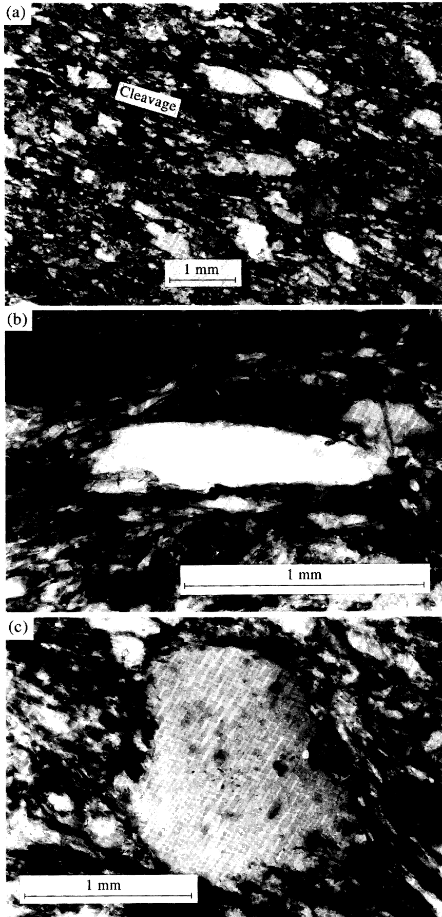
Fig. 2. Photomicrographs of cleaved sandstones. (a) Alignment of fine-grained phyllosilicates (chlorite, muscovite) defining a pervasive schistosity. The majority of detrital grains are flattened and truncated against the cleavage. (b) Very thin, flattened pressolved detrital quartz ( X -grains) with smooth sides aligned parallel to the cleavage. (c) Grains showing only slightly modified detrital shapes ( Z -grains). Such grains have rounded or irregular boundaries against the cleavage and exhibit long tails of pressure shadows.
