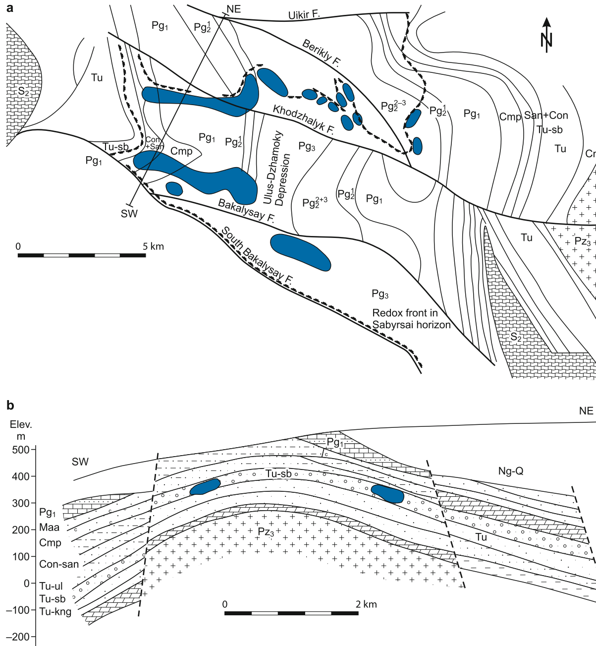
Fig. 15.15. Nurabad District, Sabysai deposit, a schematic plan and b SW-NE section showing the distribution of ore bodies hosted in Upper Turonian Sabysai Horizon (explanations and legend see at Fig. 15.5 ) (after Karimov et al. 1996)
