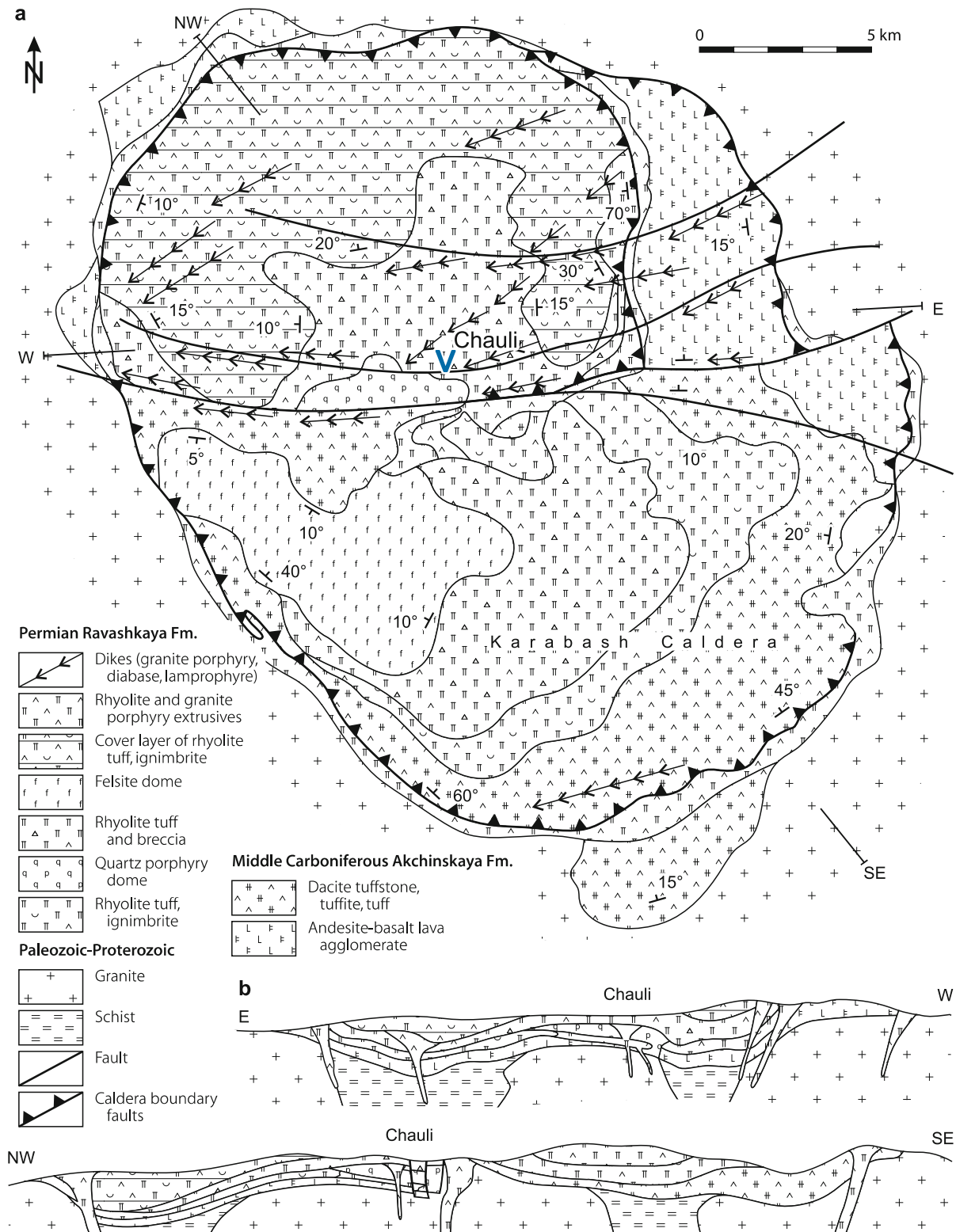
Fig. 15.17. Karamazar region, Chauli deposit, a geological map of and b sections across the Karabash Caldera showing the lithologic-structural setting of the volcanic-type deposit (see Fig. 7.2 for location) (after Laverov et al. 1993)
