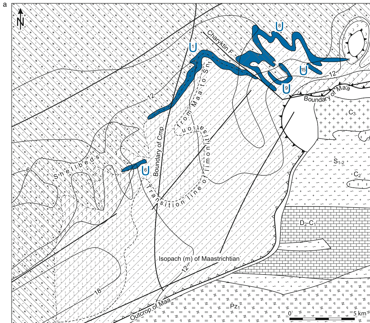
Fig. 15.8. Zarafshan District, Sugrally deposit, geological map illustrating the distribution of alteration facies a in Maastrichtian and b in Lower Senonian sediments and the related position of U ore bodies (explanations and legend see at Fig. 15.5 ) (after Shchetchkin and Kislyakov 1993)
