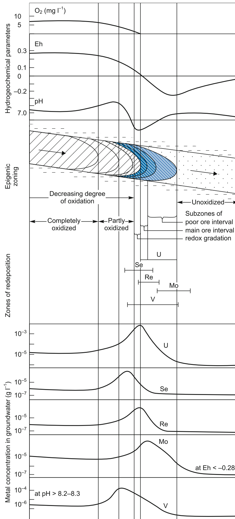
Fig. 15.3. Kyzylkum Basins, schematic section across a redox front documenting typical hydrogeochemical conditions and related differentiated oxidation zones as well as the concentration of U, Se, Re, Mo, and V in groundwater and distribution of these elements across the redox interface (after Karimov et al. 1996)
